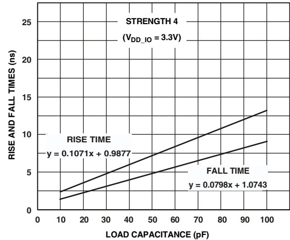
Figure 36. Typical Output Rise and Fall Time (10%–90%, V_{DD\_IO} = 3.3\text{ V} ) vs. Load Capacitance at Strength 4
