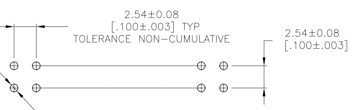
RECOMMENDED HOLE LAYOUT
