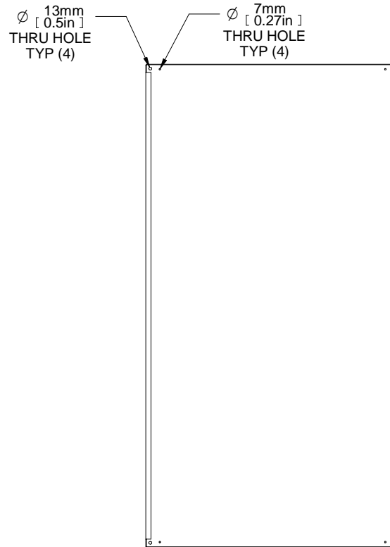
REAR VIEW
