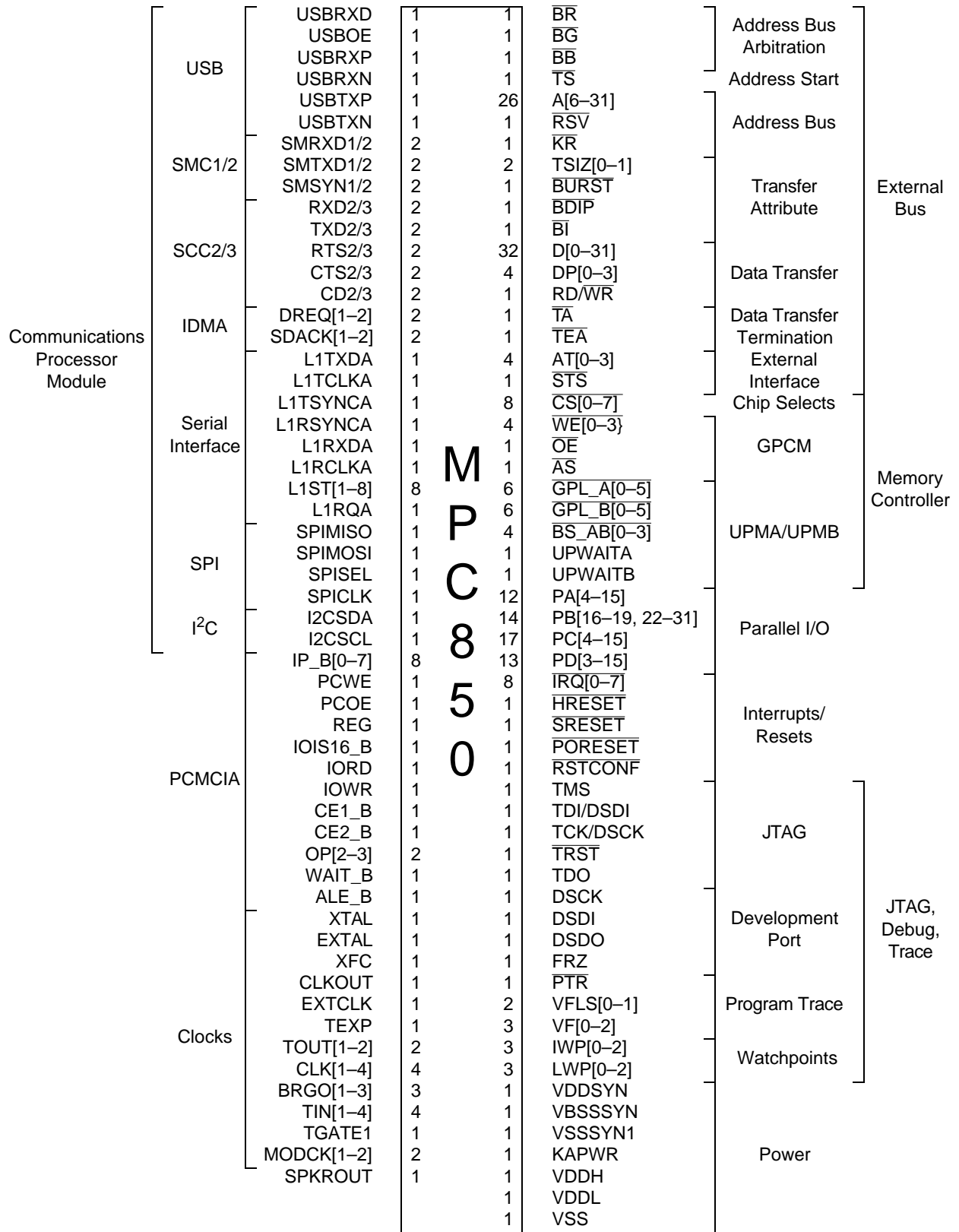
Figure 2. MPC850 Functional Signal Diagram
