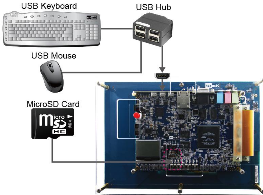
Figure 1-7 VEEK-MT-SoCKit Setup
