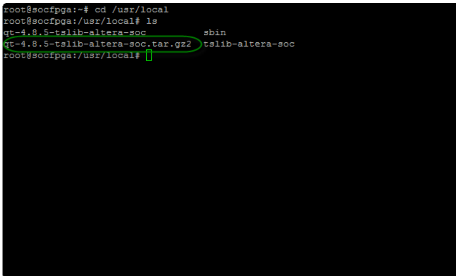
Figure 8-6 Check qt-4.8.5-tslbi-altera-soc.tar.gz2
