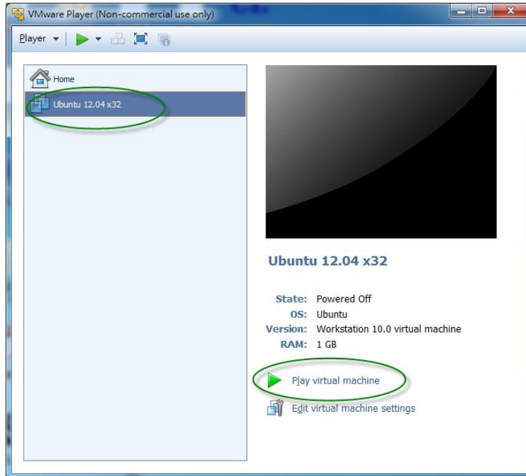
Figure 2-26 Start Ubuntu
