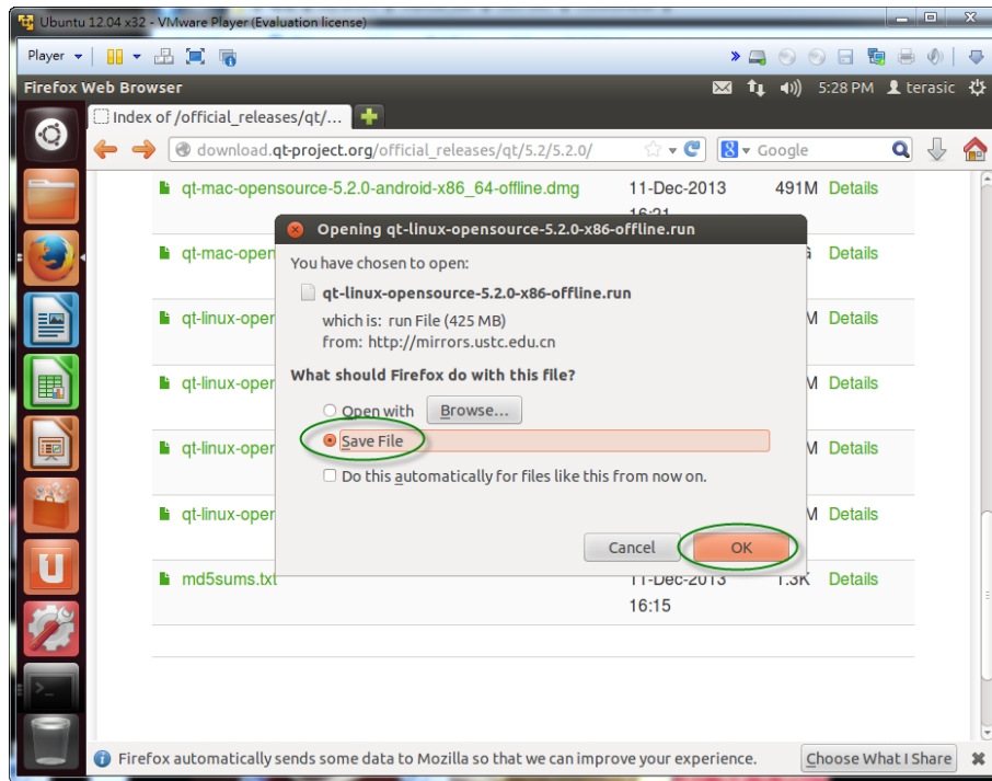
Figure 6-2 Opening Dialog
