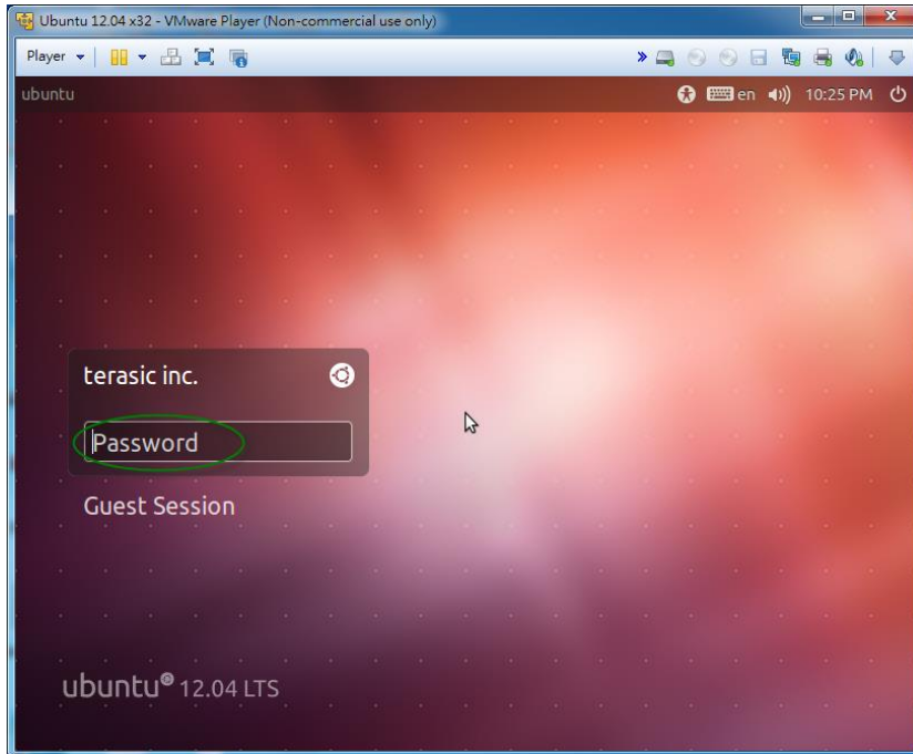
Figure 2-23 Ubuntu Login
