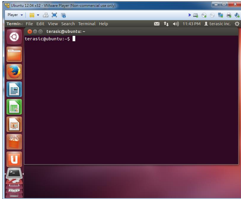
Figure 2-27 Linux Terminal
