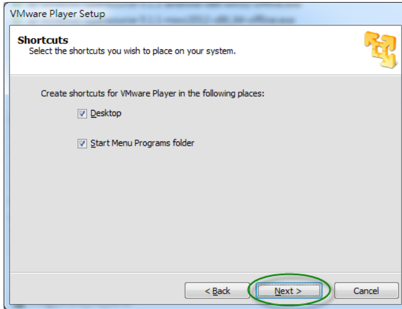
Figure 2-8 Shortcuts Dialog
