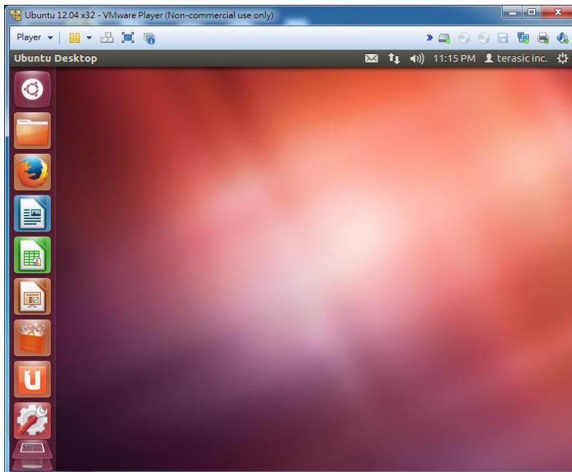
Figure 2-24 Ubuntu Desktop
