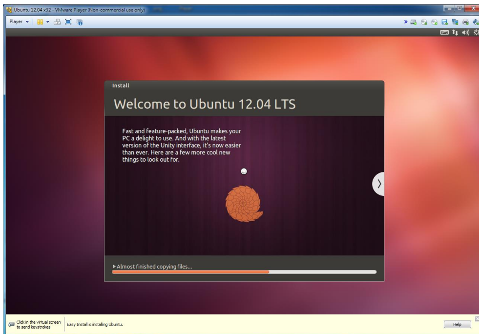
Figure 2-22 Installation Progress
