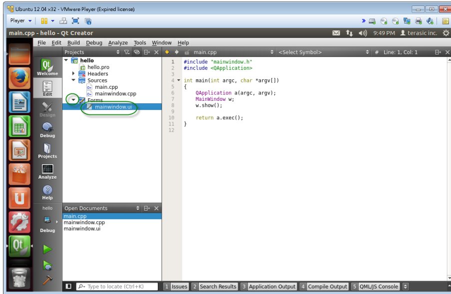
Figure 6-27 Open GUI
