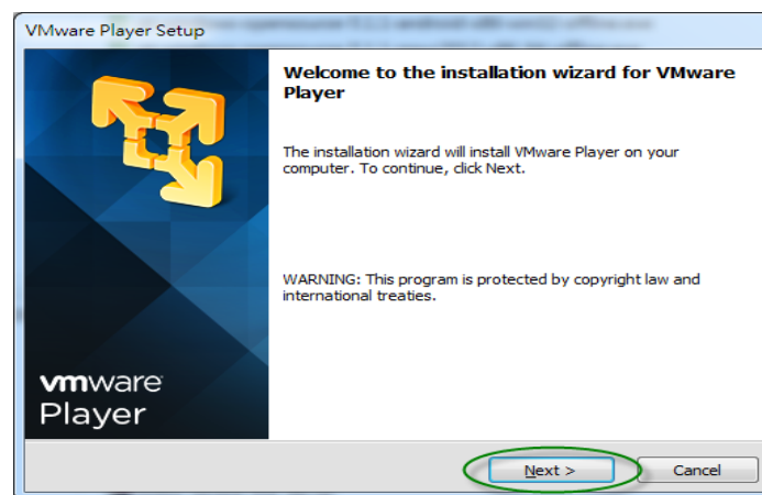
Figure 2-3 Welcome Dialog
