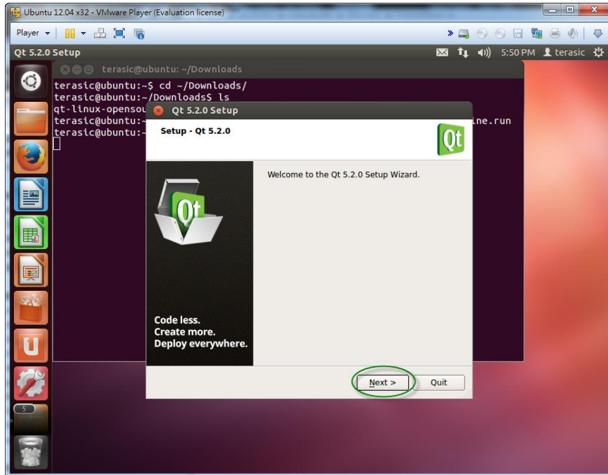
Figure 6-6 Welcome Dialog
