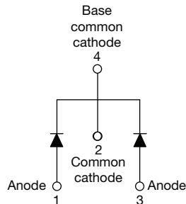
3L TO-220AB
