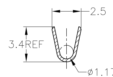
SECT. C-C
