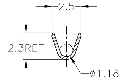
SECT. B-B
