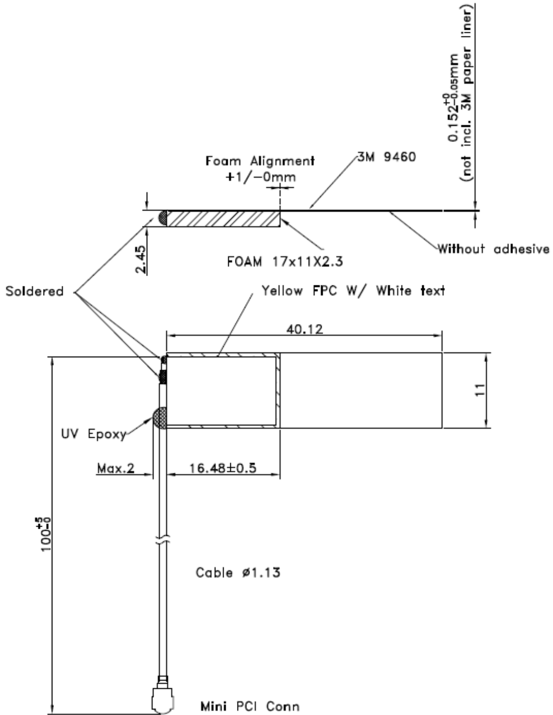
Figure 2 Physical Dimensions
