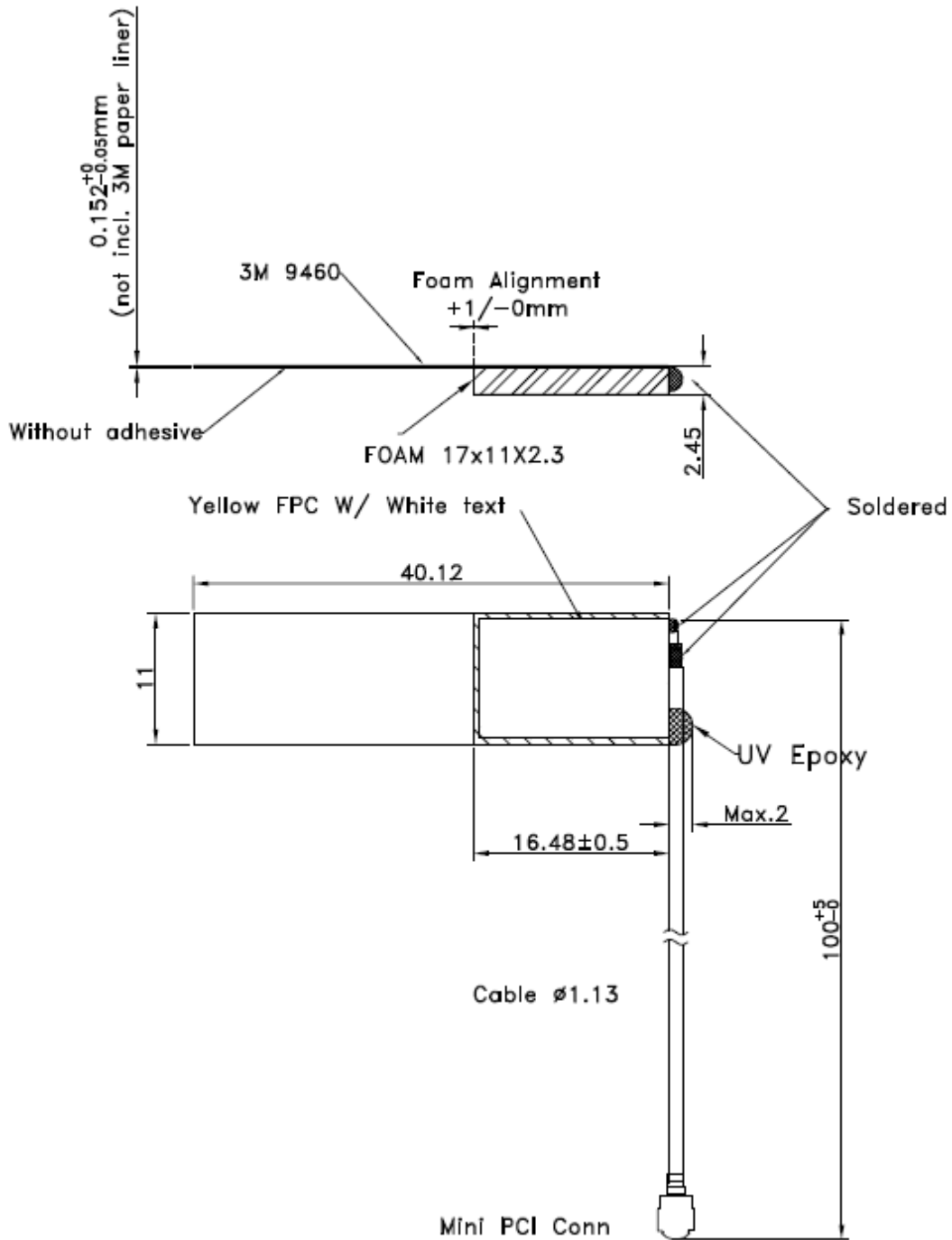
Figure 1 Physical Dimensions
