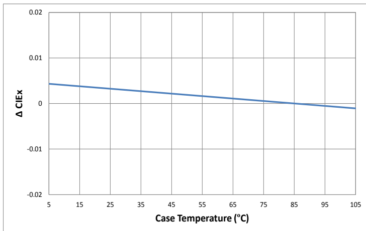
Change in CIE x vs. Case Temperature (3000K, 80CRI)
