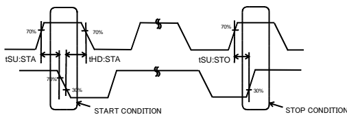
Figure 1.-(b) Start-Stop Bit Timing
