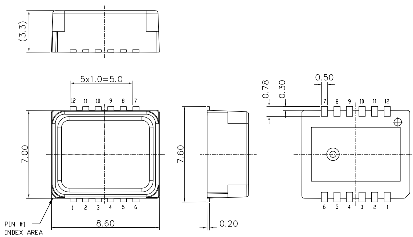
Figure 3. Housing dimensions
