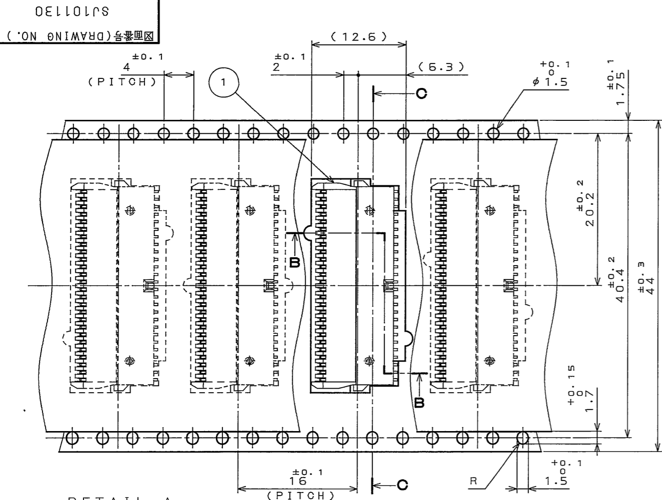
DETAIL A (SCALE 2:1)
