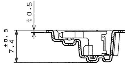
SECT. B-B (SCALE 2:1)
