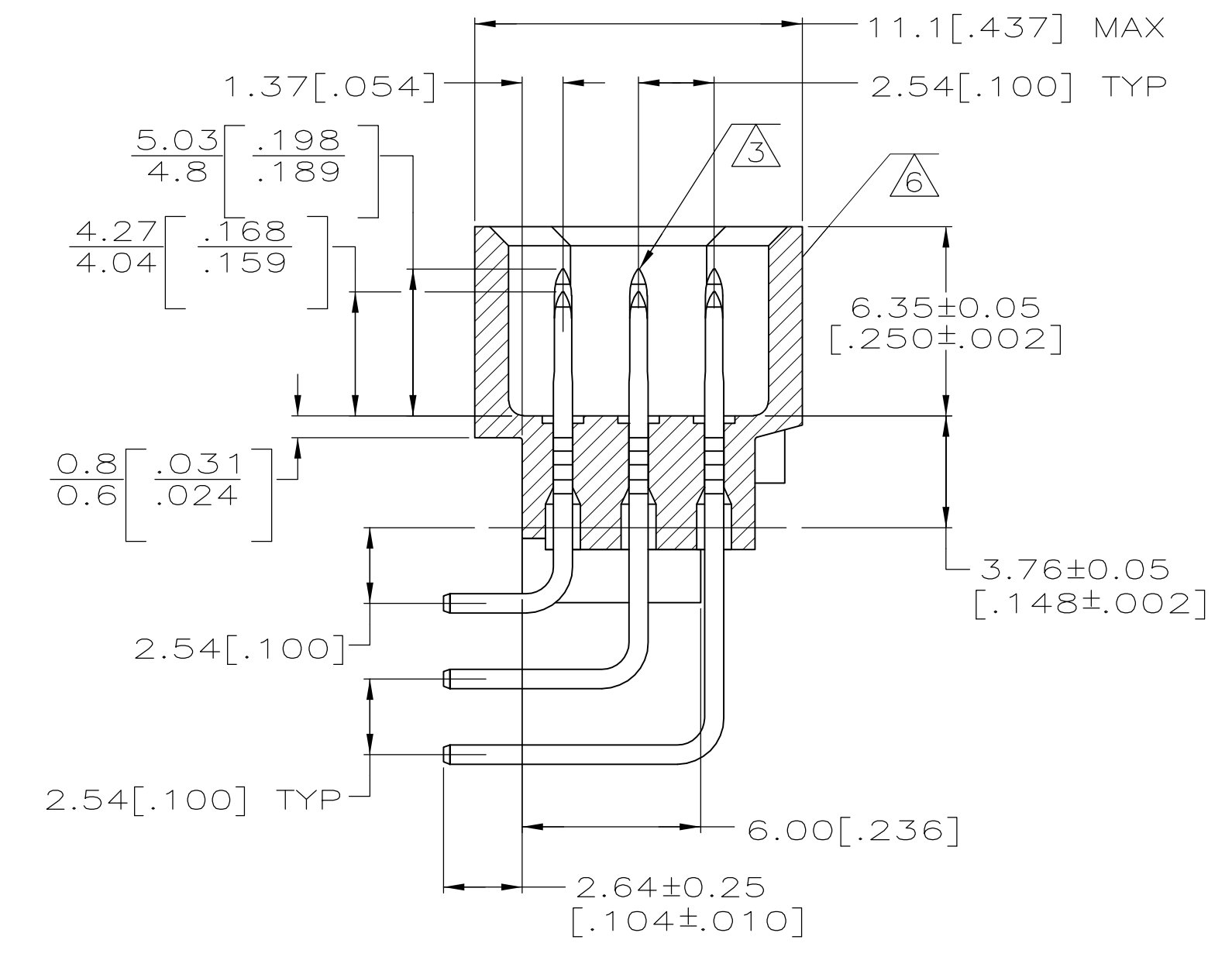
SECTION Z-Z
