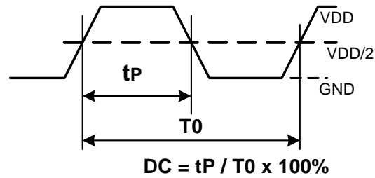
Figure 7. Output Duty Cycle (DC)
