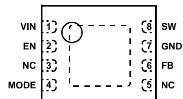
ISL9108 (8 LD 2X3 DFN) TOP VIEW
