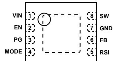
ISL9107 (8 LD 2X3 DFN) TOP VIEW
