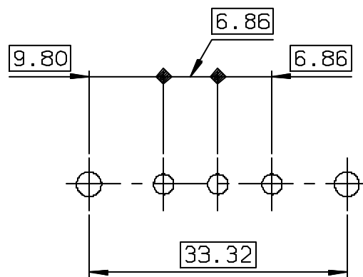
LAYOUT DIMENSIONS (after plating) CONNECTOR SIDE VIEW
