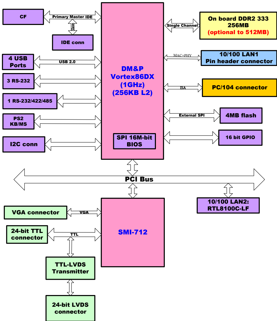
Figure 2.3 Block Diagram
