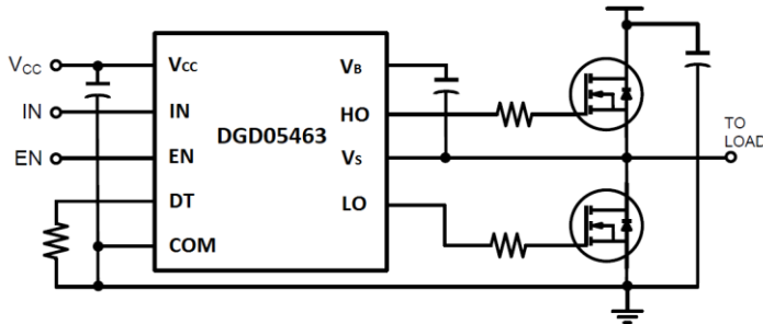
Typical Configuration
