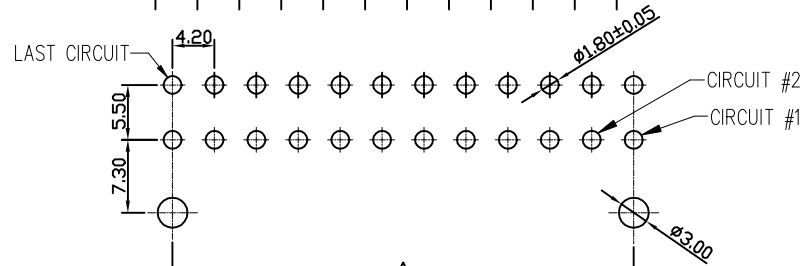
PCB LAYOUT COMPONENT SIDE FOR 6 ~ 24 POS.
