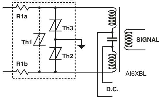
Figure 18. ISDN Protection
