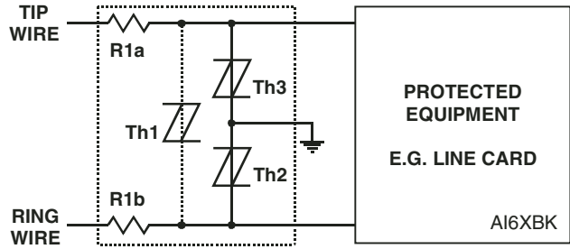
Figure 17. Protection Module
