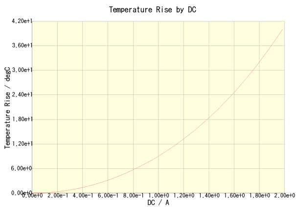
CLF6045T-220M-CA(Amb. Temp. = 20degc)
