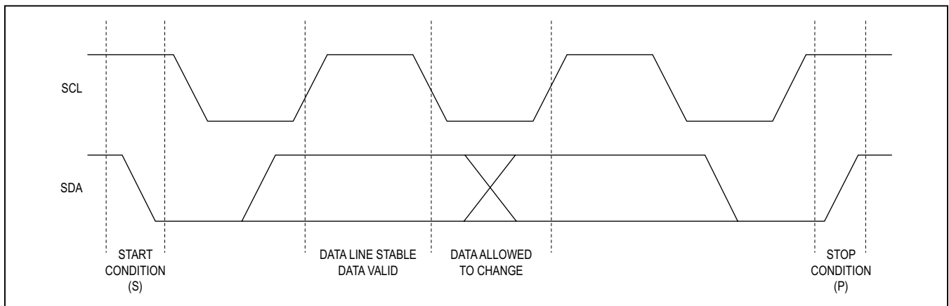
Figure 15. Bit Transfer
