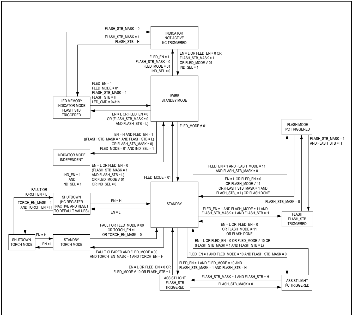
Figure 9. State Flowchart
