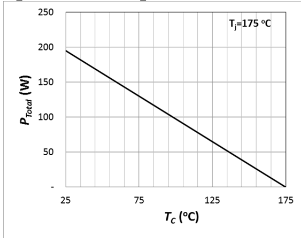
Fig. 19 Power Derating
