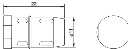
Dimensional drawing
