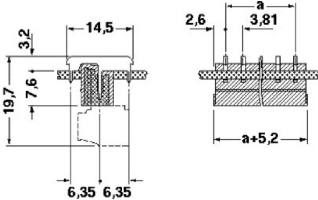
Dimensioned drawing
