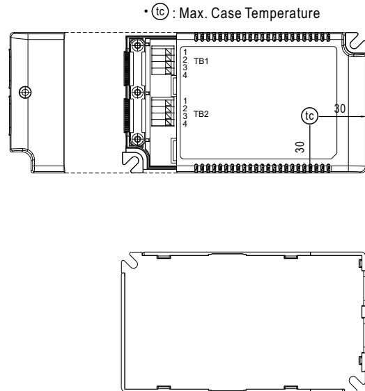
Terminal Pin No. Assignment(TB2)
