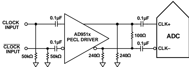
Figure 54. Differential PECL Sample Clock (Up to 1 GHz)
