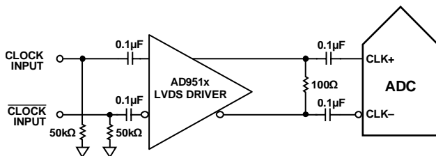
Figure 55. Differential LVDS Sample Clock (Up to 1 GHz)
