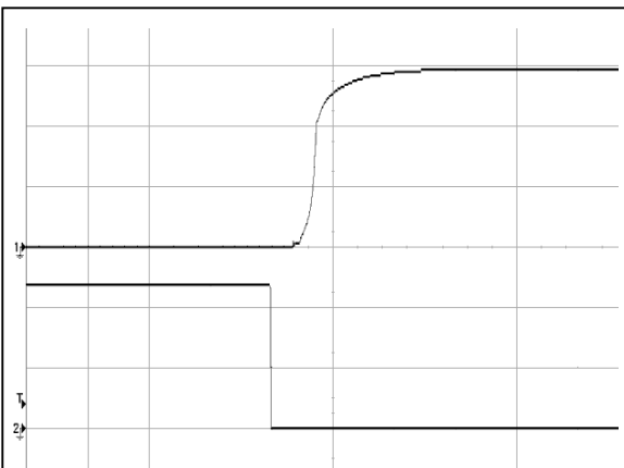
Figure 5: AGF700-48S30-6L Remote ON Waveform (200mS/div) Ch 1: V o (10V/div) Ch 2: Remote ON (20V/div)
