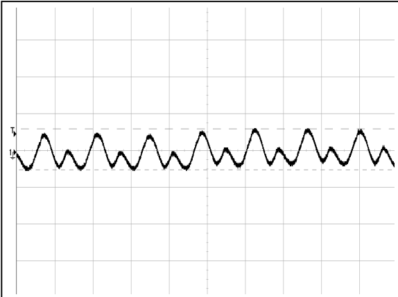
Figure 1: AGF700-48S30-6L Input Reflected Ripple Current Waveform Ch 1: I i (5 \mu S/div, 20mA/div)
