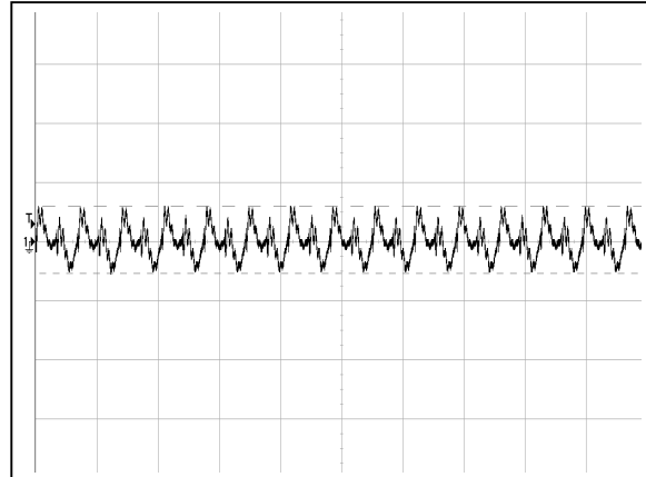
Figure 2: AGF700-48S30-6L Ripple and Noise Measurement Ch 1: V o (10 \mu s/div, 100mV/div)
