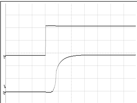
Figure 3: AGF700-48S30-6L Output Voltage Startup Characteristic (200mS/div) Ch 1: V in (20V/div) Ch 2: V o (10V/div)
