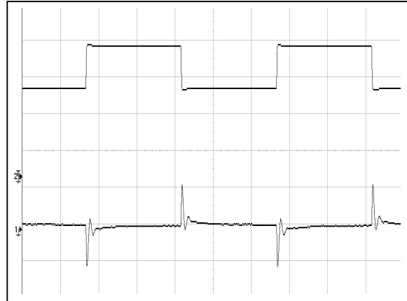
Figure 8: AGF700-48S30-6L Transient Response 50%-75%-50% load change, 0.1A/uS slew rate, Ch 1: Vo (200mV/div) Ch 2: Io (5A/div)
