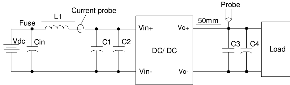
Figure 24 Input ripple & output ripple & noise test configuration
