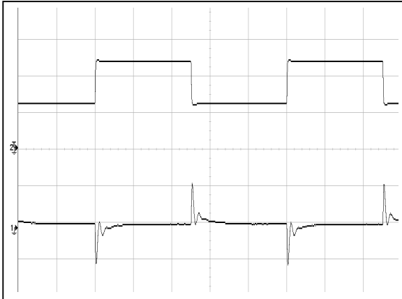
Figure 7: AGF700-48S30-6L Transient Response 25%-50%-25% load change, 0.1A/uS slew rate, Ch 1: Vo (200mV/div) Ch 2: Io (5A/div)
