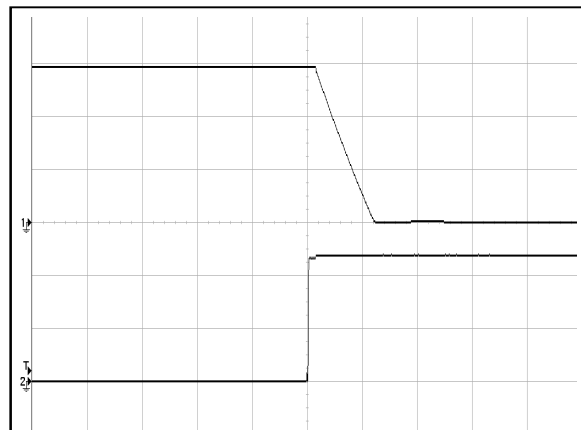
Figure 6: AGF700-48S30-6L Remote OFF Waveform (1mS/div) Ch1: V o (10V/div) Ch 2: Remote OFF (20V/div)
