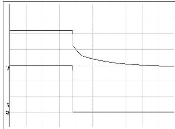
Figure 4: AGF700-48S30-6L Turn Off Characteristic (500mS/div) Ch 1: V in (20V/div) Ch 2: V o (10V/div)
