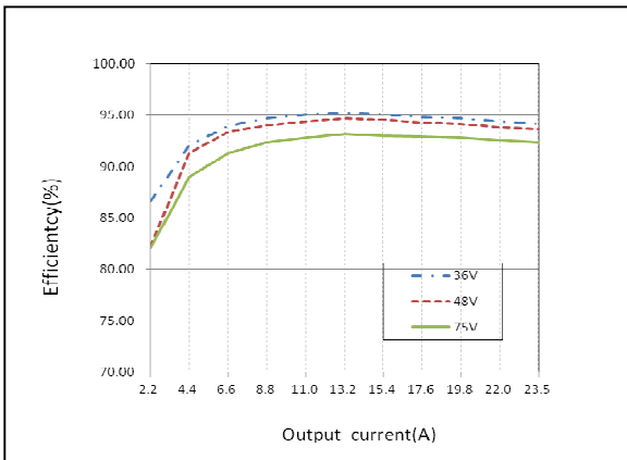
Figure 9: AGF700-48S30-6L Efficiency Curves @ 25 °C Ta=25 °C, Tc=40 °C, Vo=30V
