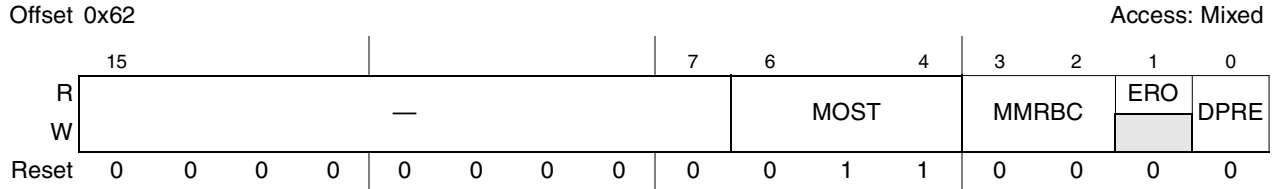
Figure 16-52. PCI-X Command Register
