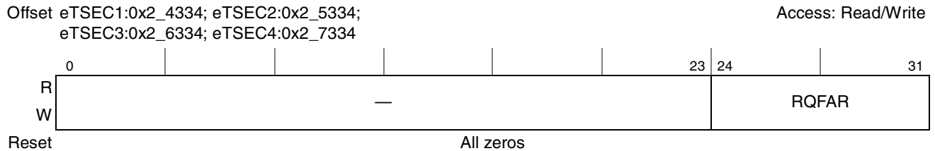
Figure 14-32. Receive Queue Filer Table Address Register Definition
