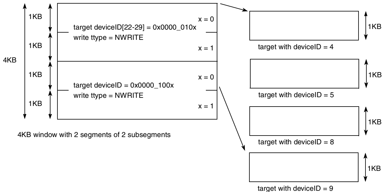
Figure 17-54. Example of Multi-Targeting
