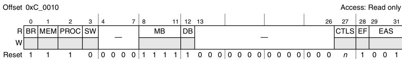
Figure 17-6. Processing Element Features Capability Register (PEFCAR)
