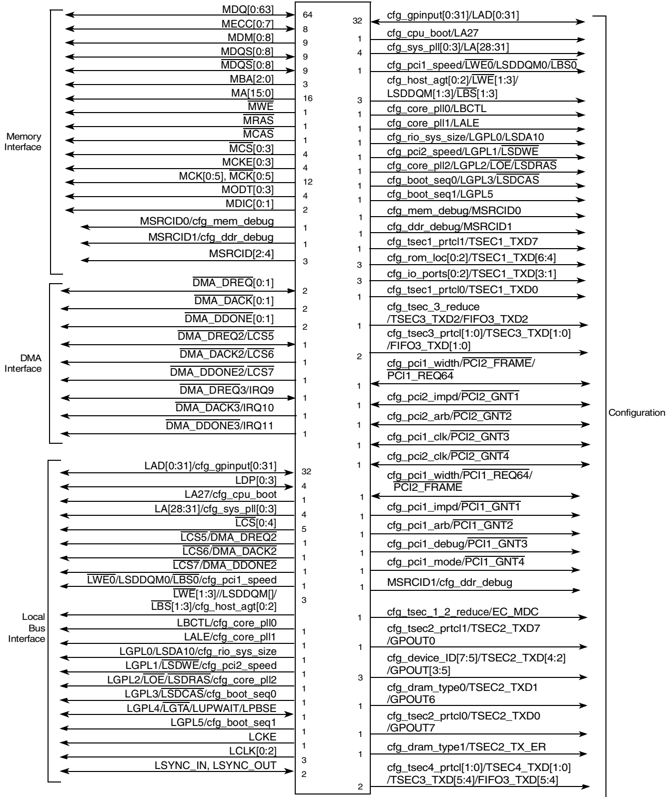
Figure 3-3. MPC8548E Signal Groupings (3/3) (Continued)
