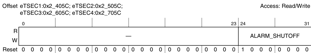
Figure 14-12. FIFO_RX_ALARM_SHUTOFF Register Definition
