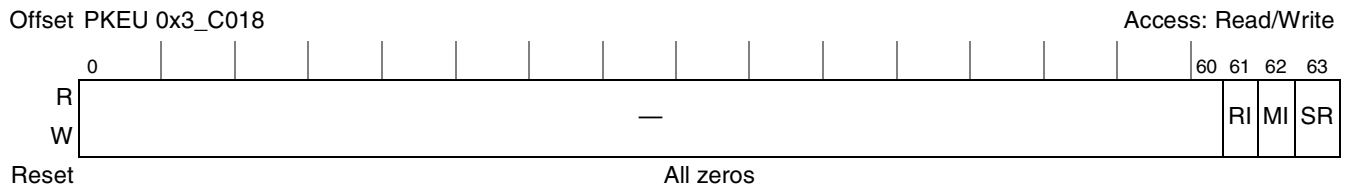
Figure 19-12. PKEU Reset Control Register
