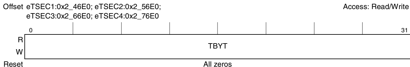
Figure 14-81. Transmit Byte Counter Register Definition
