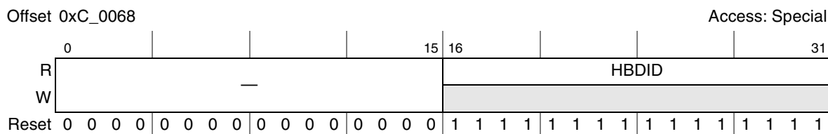
Figure 17-14. Host Base Device ID Lock Command and Status Register (HBDIDLCSR)
