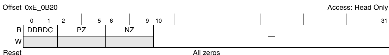
Figure 20-20. DDR Calibration Status Register (DDRCSSR)
