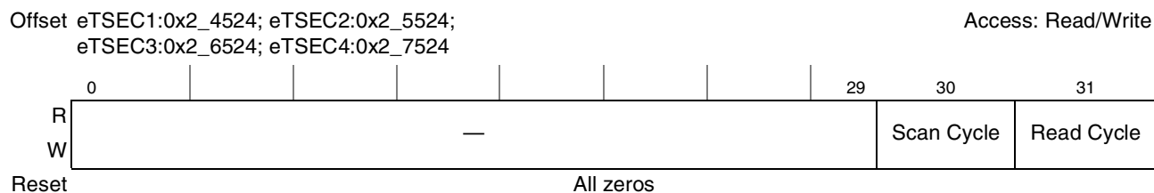
Figure 14-47. MIIMCOM Register Definition
