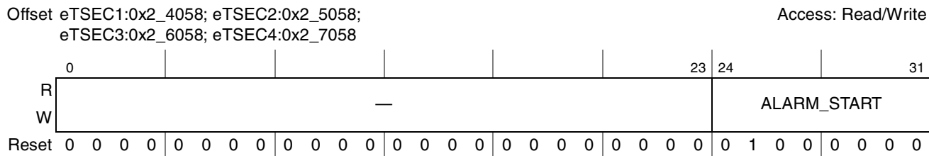
Figure 14-11. FIFO_RX_ALARM Register Definition
