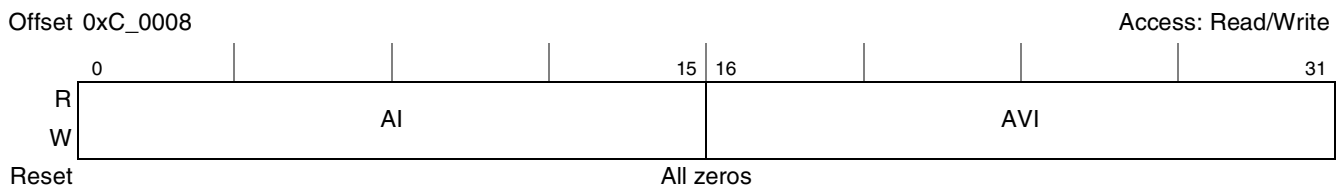
Figure 17-4. Assembly Identity Capability Register (AIDCAR)
