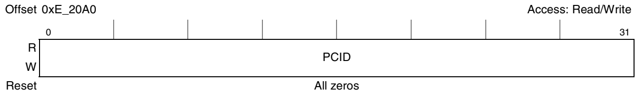
Figure 22-17. Programmed Context ID Register (PCIDR)
