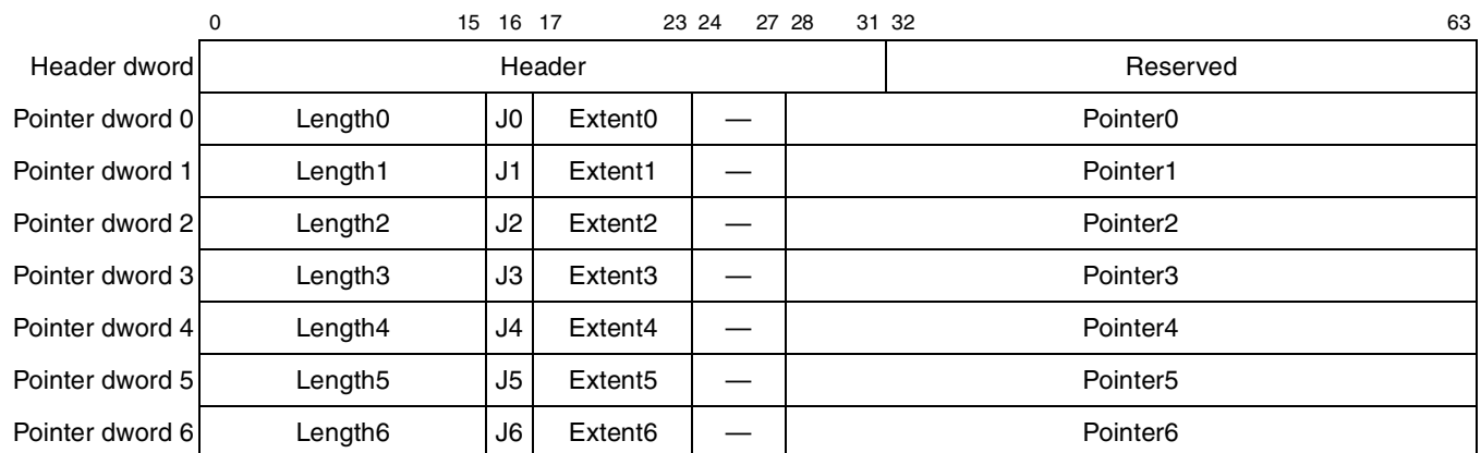
Figure 19-3. Descriptor Format
