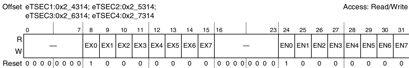
Figure 14-30. RQUEUE Register Definition
