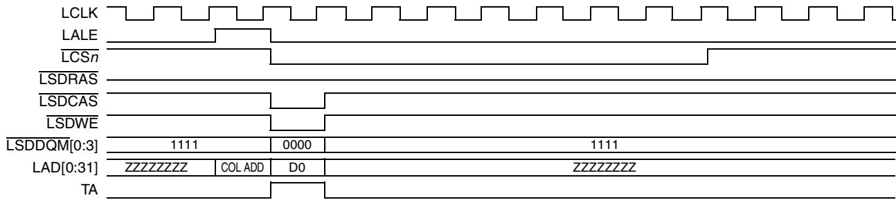
Figure 13-46. SDRAM Single-Beat Write, Page Hit
