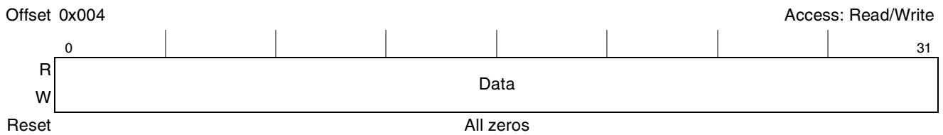
Figure 16-4. PCI/X CFG_DATA Register
