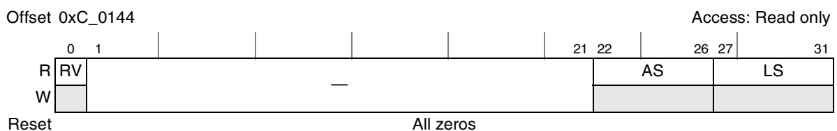
Figure 17-21. Link Maintenance Response Command and Status Register (LMRESPCSR)
