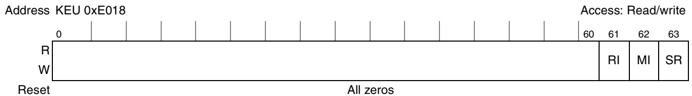
Figure 19-64. KEU Reset Control Register
