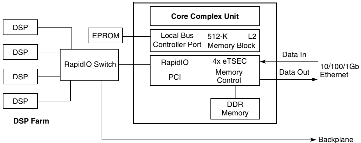
Figure 1-9. MPC8548E as a Control Plane Processor for a DSP Farm Interconnected with RapidIO
