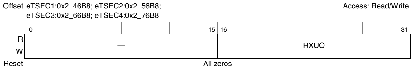
Figure 14-71. Receive Unknown Opcode Packet Counter Register Definition
