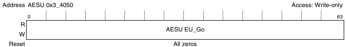
Figure 19-58. AESU EU Go Register
