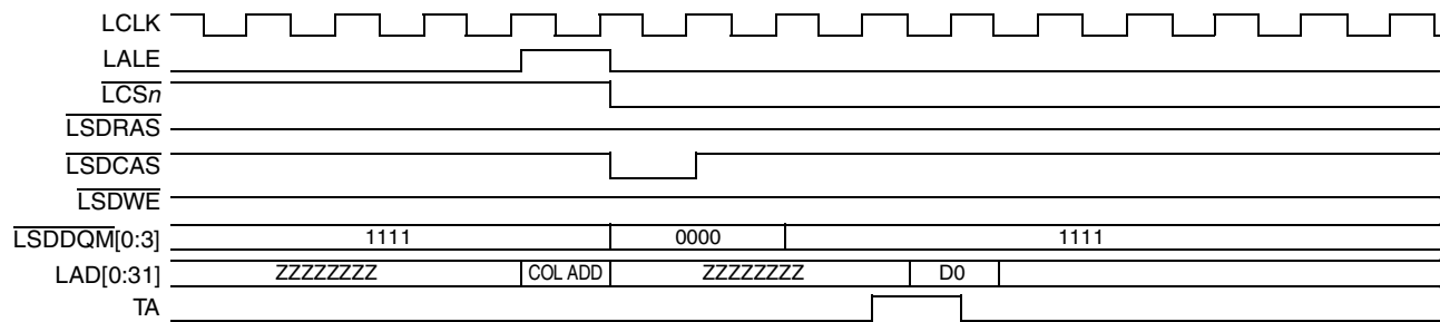
Figure 13-43. SDRAM Single-Beat Read, Page Hit, CL = 3
