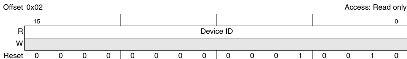
Figure 16-28. PCI Device ID Register
