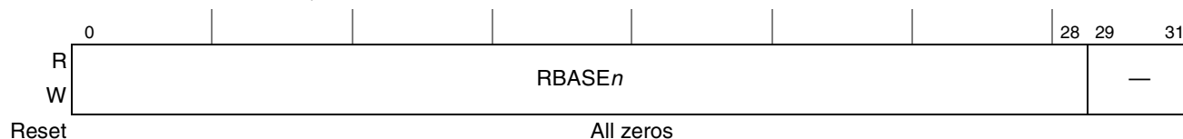
Figure 14-40. RBASE Register Definition
