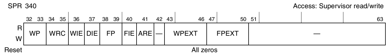
Figure 6-10. Timer Control Register (TCR)
