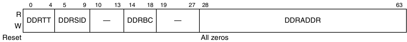
Figure 22-21. DDR Trace Buffer Entry
