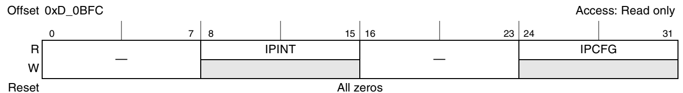
Figure 17-52. IP Block Revision Register 2 (IPBRR2)
