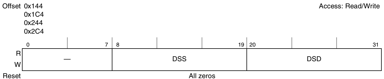
Figure 15-23. Destination Stride Registers (DSR n )
