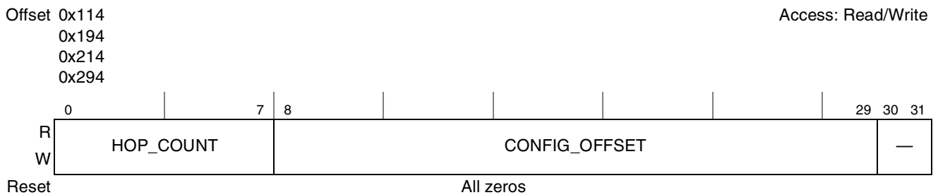
Figure 15-11. Source Address Registers for RapidIO Maintenance Reads (SAR n )
