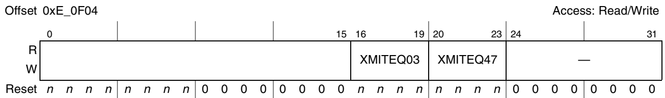
Figure 20-24. SerDes Control Register 0 (SRDSCR0)
