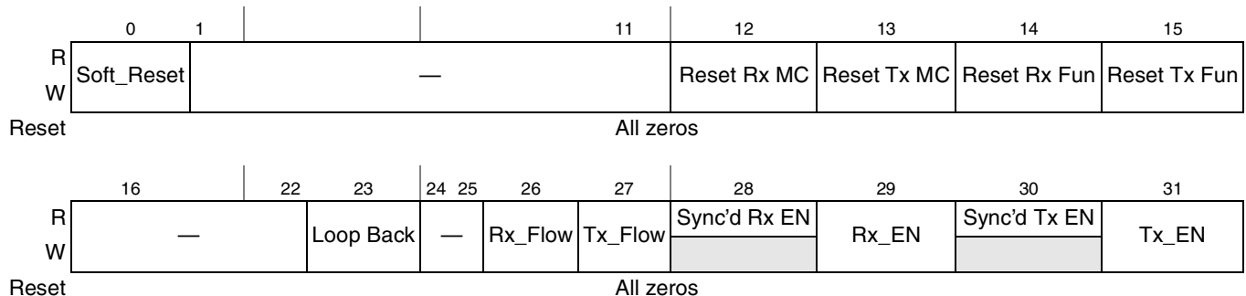
Figure 14-41. MACCFG1 Register Definition
