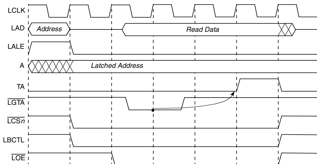
Figure 13-33. External Termination of GPCM Access
