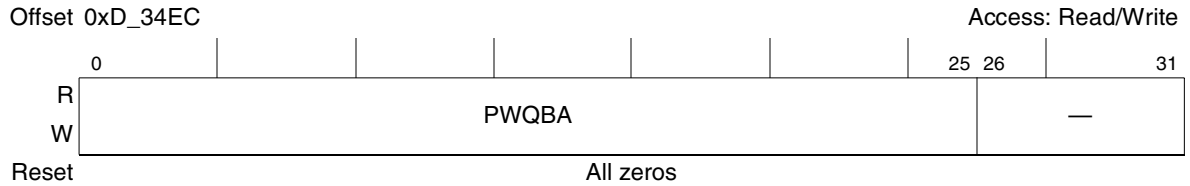
Figure 17-98. Inbound Port-Write Queue Base Address Register (IPWQBAR)
