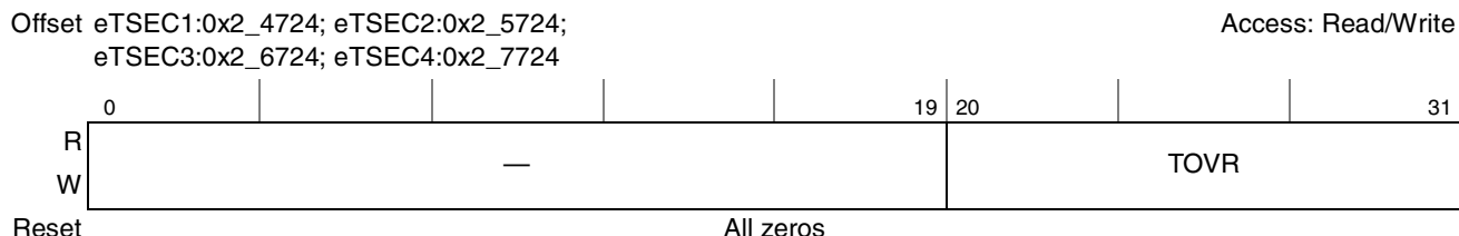
Figure 14-97. Transmit Oversized Frame Counter Register Definition
