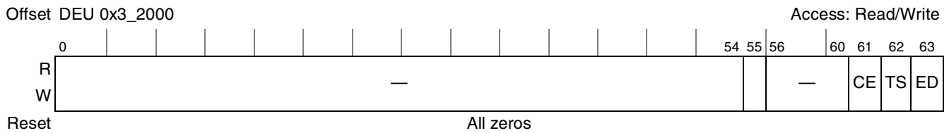
Figure 19-17. DEU Mode Register
