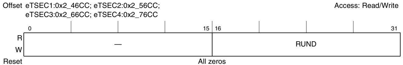
Figure 14-76. Receive Undersize Packet Counter Register Definition
