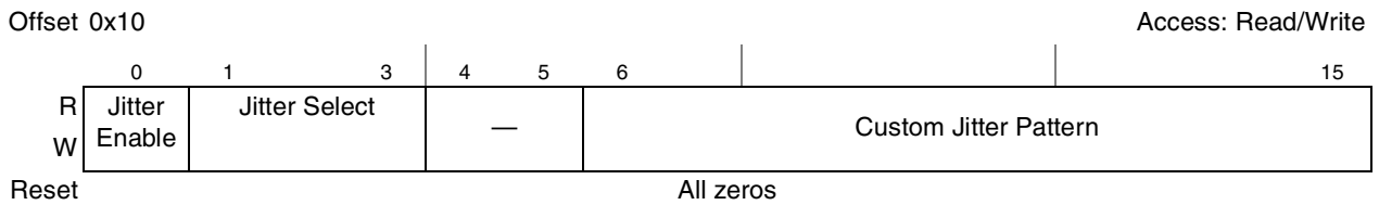
Figure 14-118. Jitter Diagnostics Register Definition
