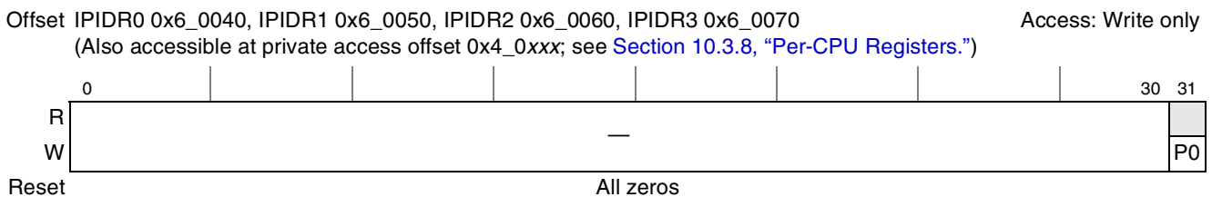
Figure 10-42. Interprocessor Interrupt Dispatch Registers (IPIDR0–IPIDR3)
