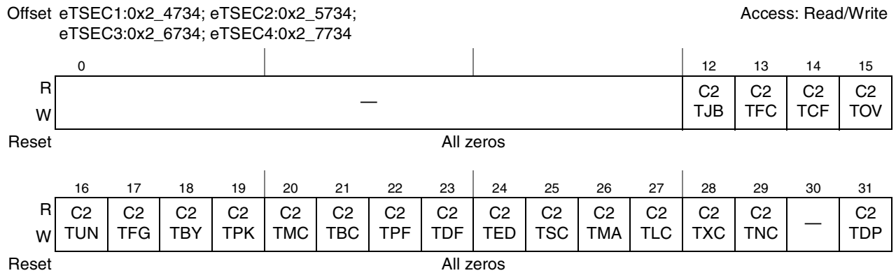
Figure 14-101. Carry Register 2 (CAR2) Register Definition
