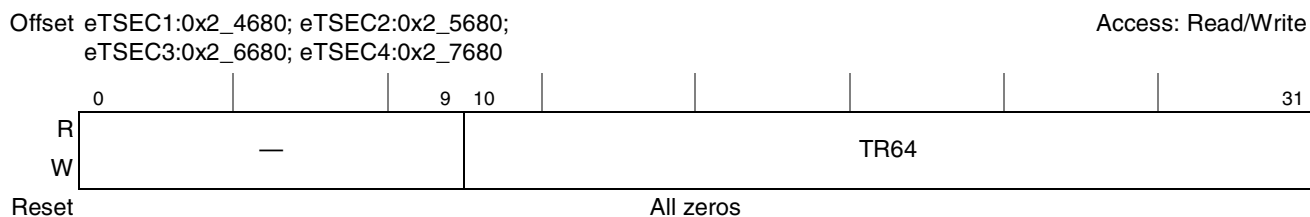
Figure 14-57. Transmit and Receive 64-Byte Frame Register Definition
