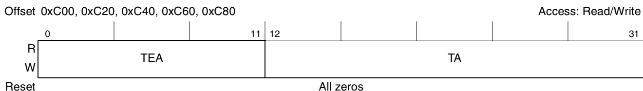
Figure 16-6. PCI/X Outbound Translation Address Registers (POTAR n )
