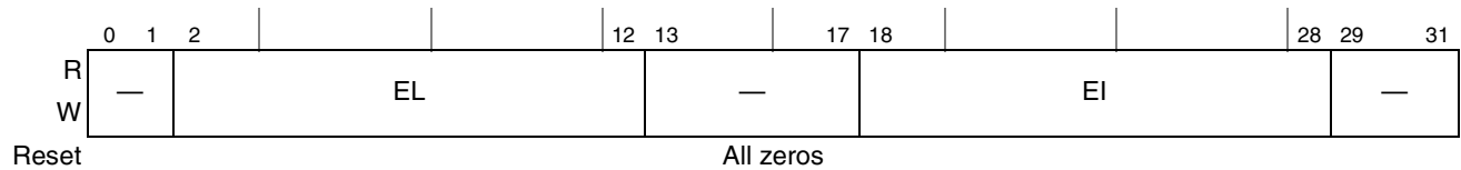
Figure 14-109. ATTRELI Register Definition
