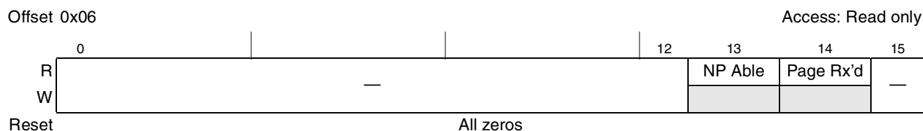
Figure 14-114. AN Expansion Register Definition
