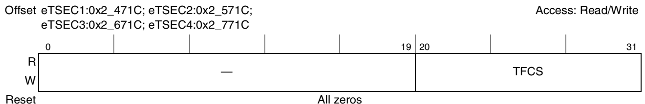
Figure 14-95. Transmit FCS Error Counter Register Definition
