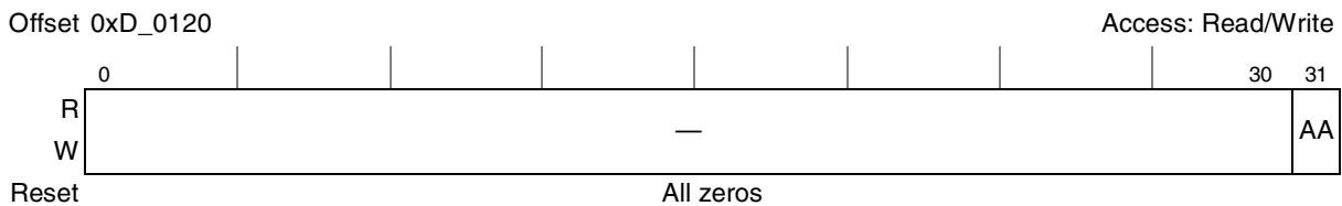
Figure 17-45. Accept-All Configuration Register (AACR)
