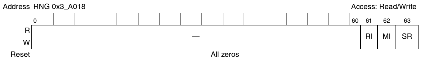
Figure 19-46. RNG Reset Control Register
