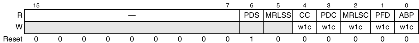
Figure 18-93. PCI Express Slot Status Register
