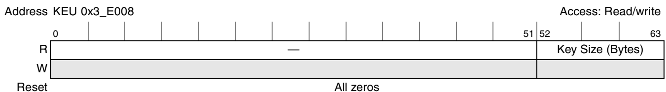
Figure 19-62. KEU Key Size Register
