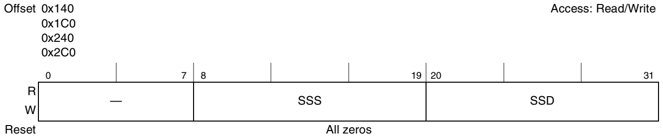
Figure 15-22. Source Stride Registers (SSR n )
