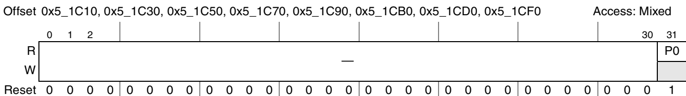
Figure 10-34. Shared Message Signaled Interrupt Destination Registers (MSIDR n )
