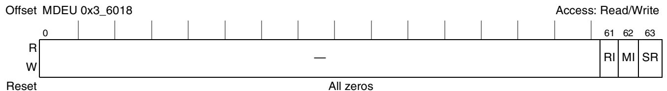
Figure 19-37. MDEU Reset Control Register
