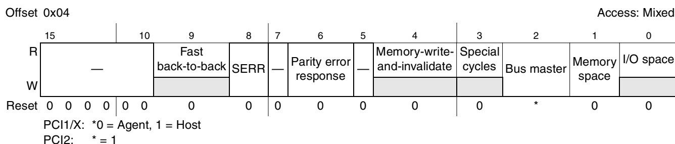
Figure 16-29. PCI Bus Command Register
