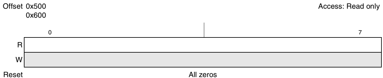
Figure 12-2. Receiver Buffer Registers (URBR0, URBR1)
