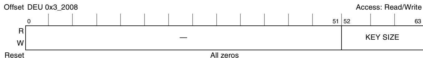
Figure 19-18. DEU Key Size Register
