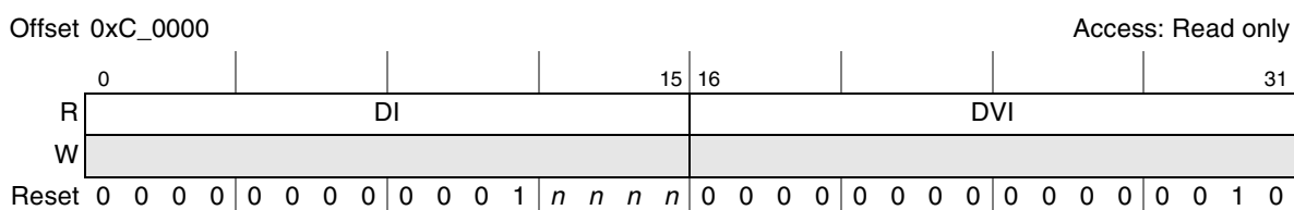
Figure 17-2. Device Identity Capability Register (DIDCAR)
