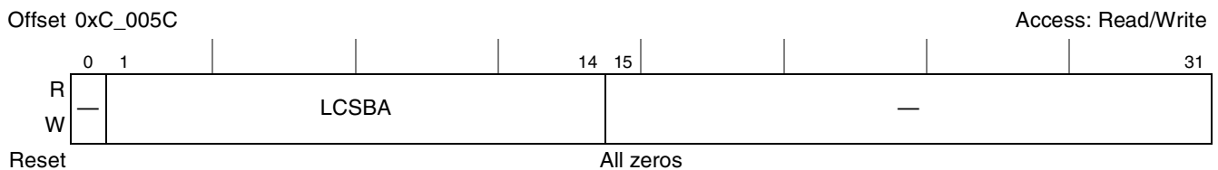
Figure 17-12. Local Configuration Space Base Address 1 Command and Status Register (LCSBA1CSR)
