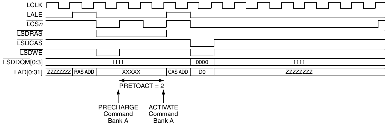
Figure 13-36. PRETOACT = 2 (2 Clock Cycles)
