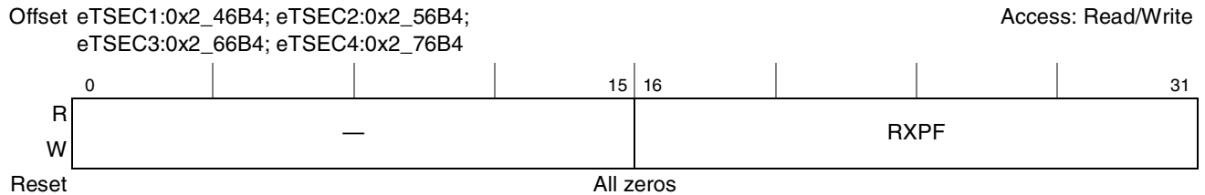
Figure 14-70. Receive Pause Frame Packet Counter Register Definition
