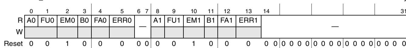
Figure 17-9. Mailbox Command and Status Register (MCSR)
