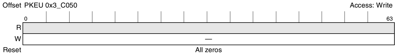
Figure 19-16. PKEU EU Go Register
