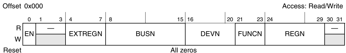
Figure 18-2. PCI Express Configuration Address Register (PEX_CONFIG_ADDR)
