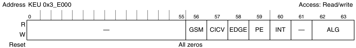
Figure 19-61. KEU Mode Register
