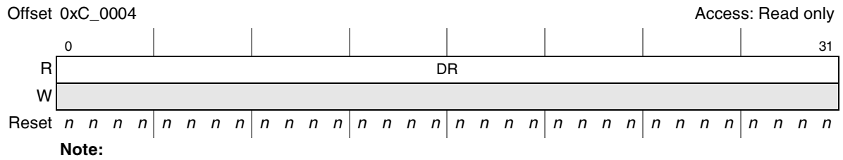
Figure 17-3. Device Information Capability Register (DICAR)
