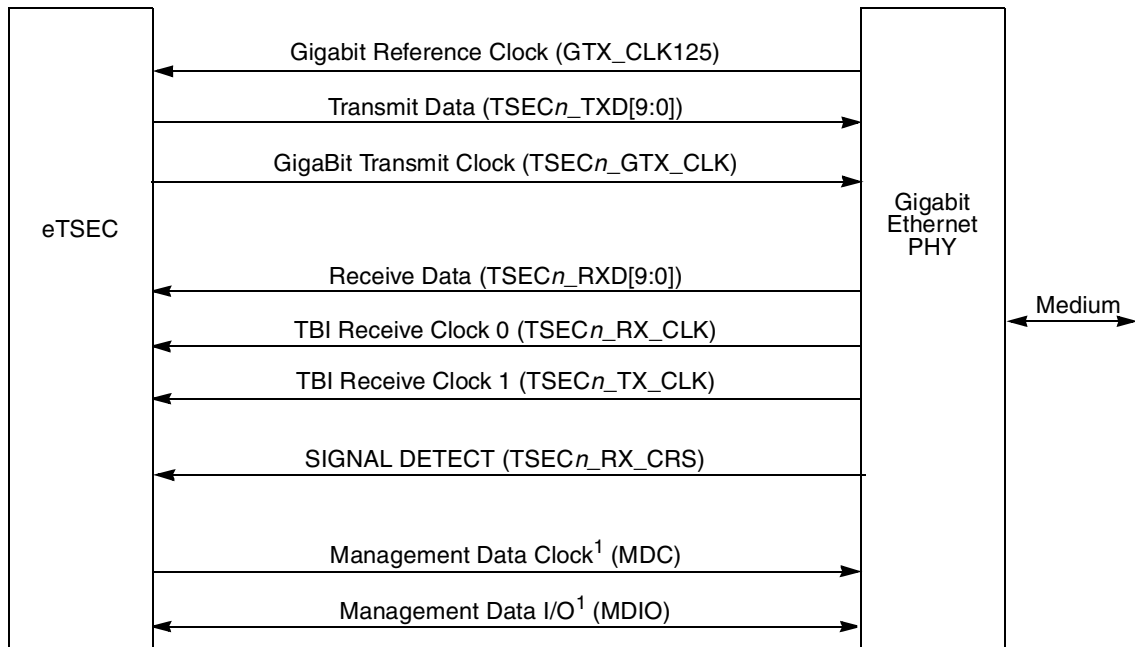
Figure 14-124. eTSEC-TBI Connection
