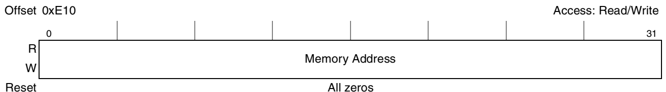
Figure 16-19. PCI/X Error Address Capture Register (ERR_ADDR)
