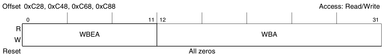
Figure 16-8. PCI/X Outbound Window Base Address Registers (POWBAR n )
