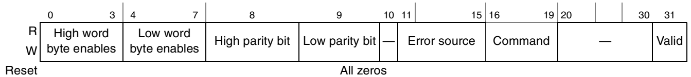
Figure 16-18. PCI/X Error Attributes Capture Register (ERR_ATTRIB)
