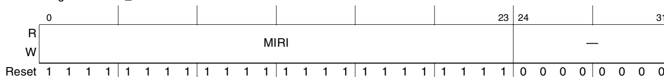
Figure 17-82. Inbound Message n Maximum Interrupt Report Interval Registers (IM n MIRIR)
