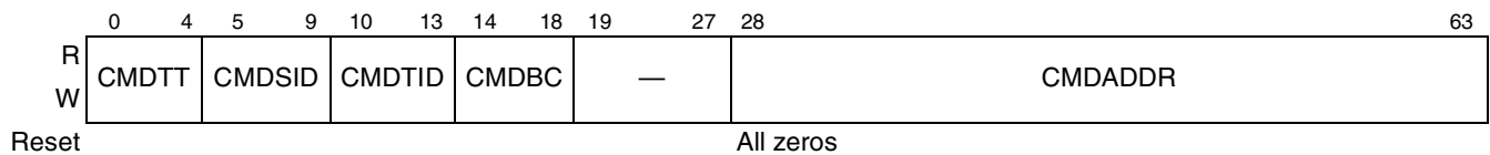
Figure 22-20. e500 Coherency Module Dispatch (CMD) Trace Buffer Entry
