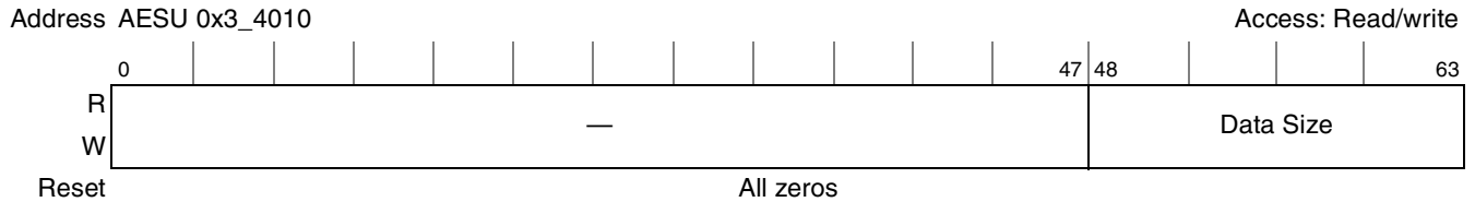
Figure 19-53. AESU Data Size Register
