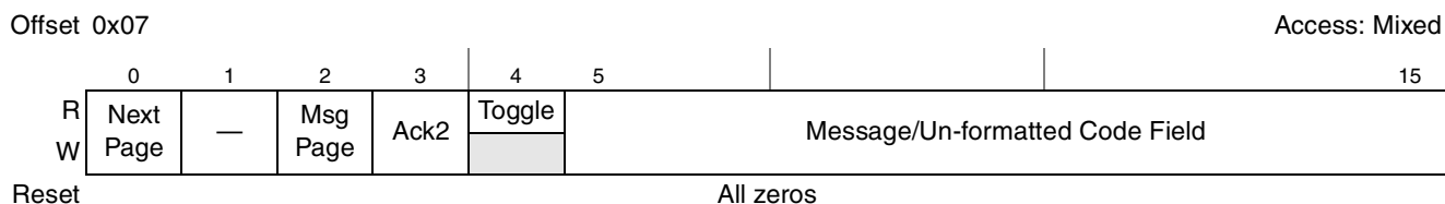
Figure 14-115. AN Next Page Transmit Register Definition
