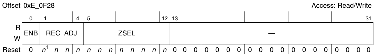
Figure 20-26. TSEC12 I/O Overdrive Control Register (TSEC12IOOVCR)
