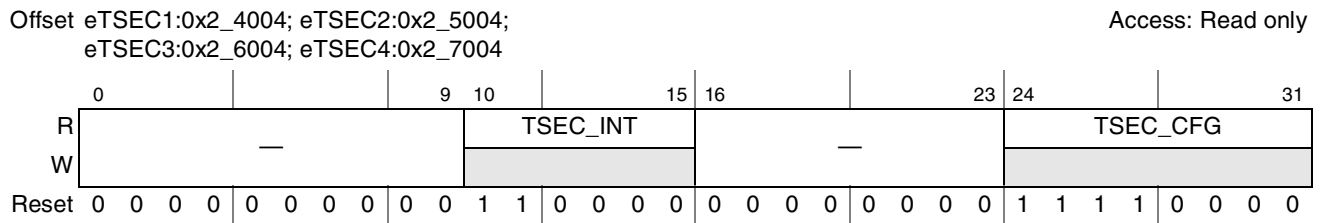
Figure 14-3. TSEC_ID2 Register
