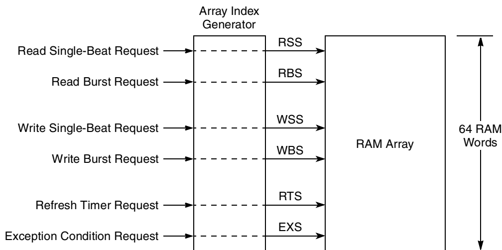
Figure 13-54. RAM Array Indexing
