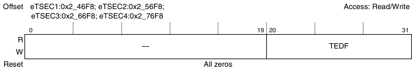
Figure 14-87. Transmit Excessive Deferral Packet Counter Register Definition
