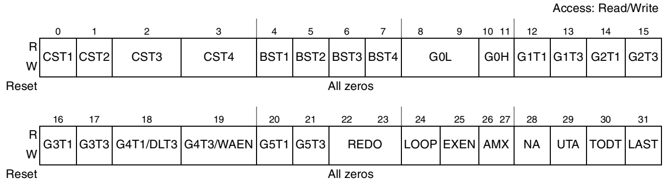
Figure 13-58. RAM Word Field Descriptions
