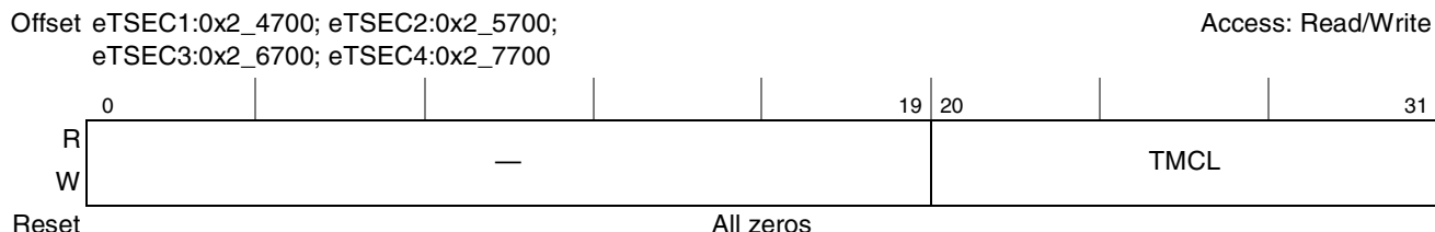
Figure 14-89. Transmit Multiple Collision Packet Counter Register Definition
