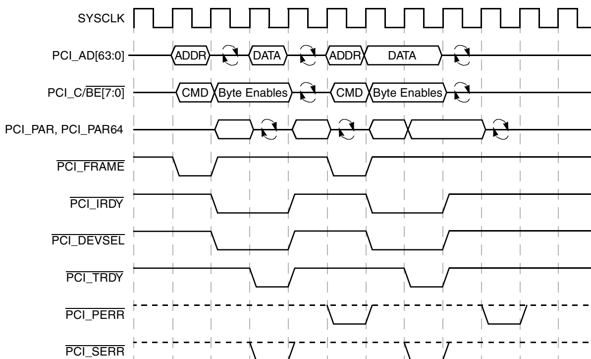
Figure 16-66. PCI Parity Operation
