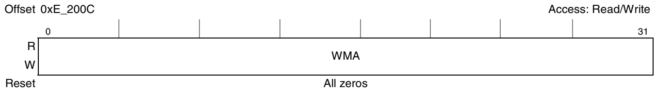
Figure 22-4. Watchpoint Monitor Address Register (WMAR)
