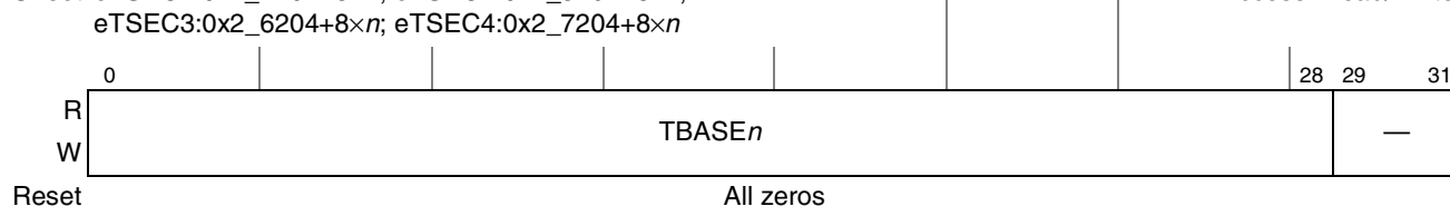
Figure 14-26. TBASE Register Definition
