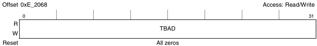
Figure 22-16. Trace Buffer Access Data Register (TBADR)
