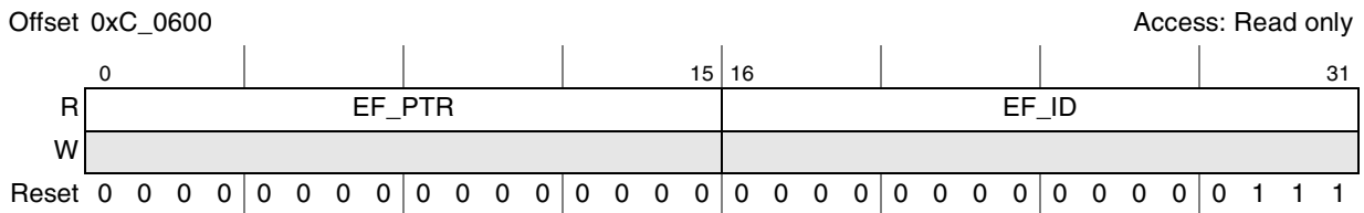
Figure 17-25. Error Reporting Block Header (ERBH)
