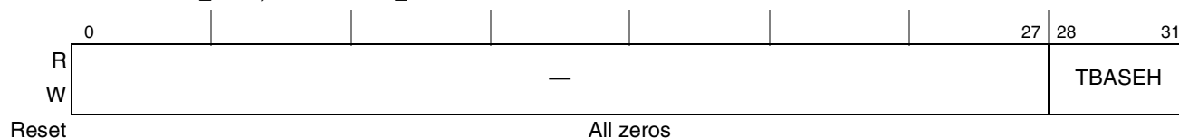
Figure 14-25. TBASEH Register Definition
