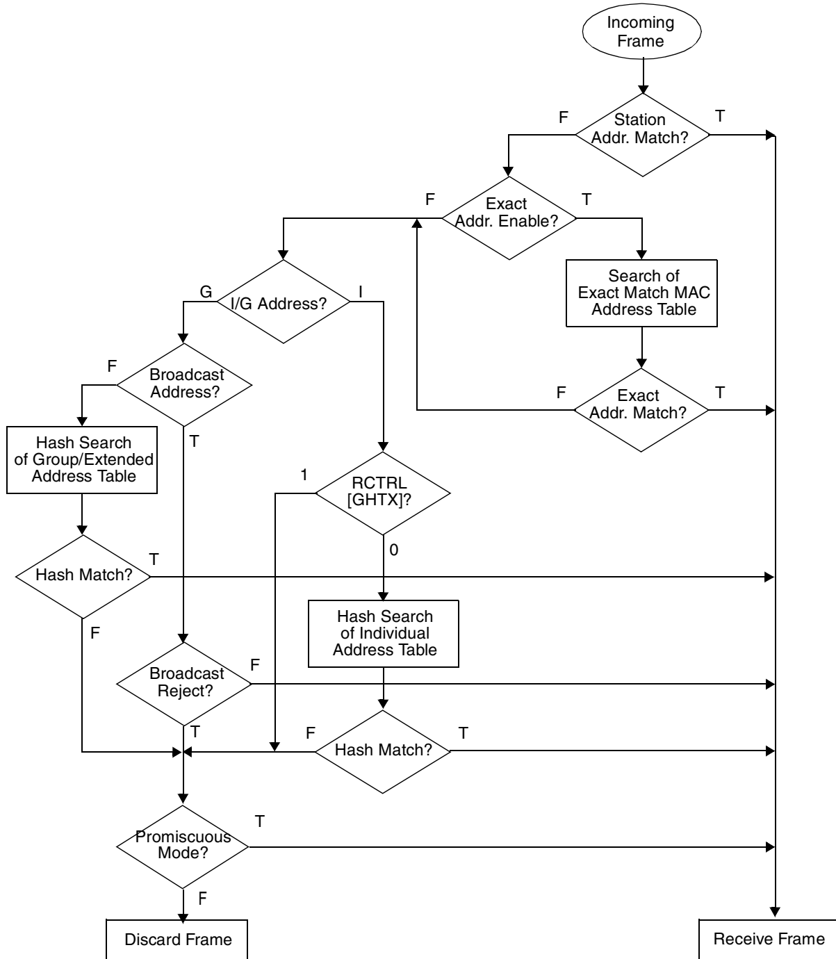
Figure 14-134. Ethernet Address Recognition Flowchart
