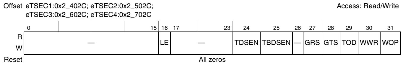
Figure 14-9. DMACTRL Register
