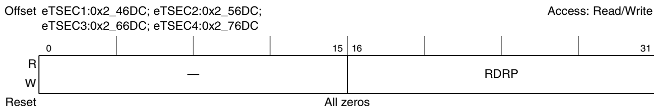
Figure 14-80. Receive Dropped Packet Counter Register Definition
