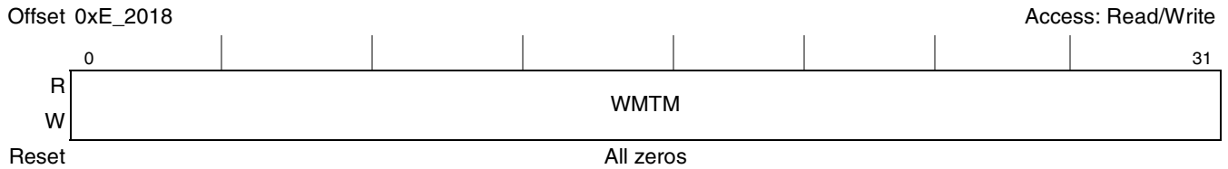
Figure 22-6. Watchpoint Monitor Transaction Mask Register (WMTMR)
