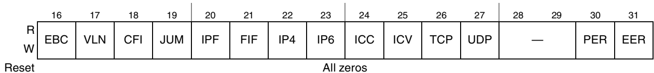
Figure 14-35. Receive Queue Filer Table Property ID1 Register Definition
