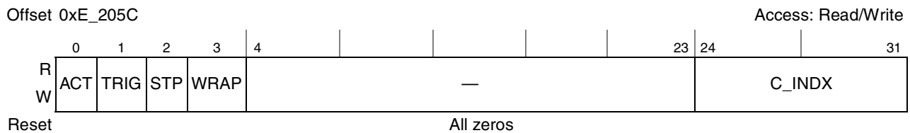
Figure 22-13. Trace Buffer Status Register (TBSR)
