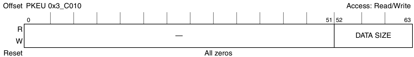
Figure 19-11. PKEU Data Size Register
