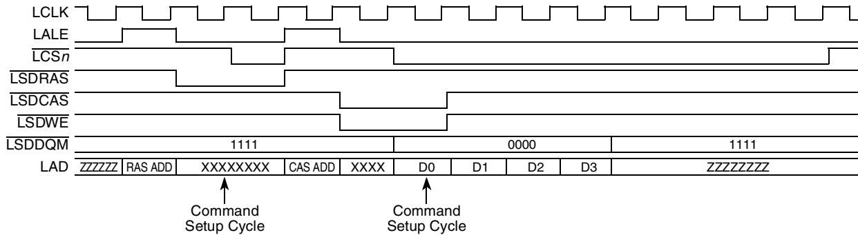
Figure 13-41. BUFCMD = 1, LCRR[BUFCMDC] = 2
