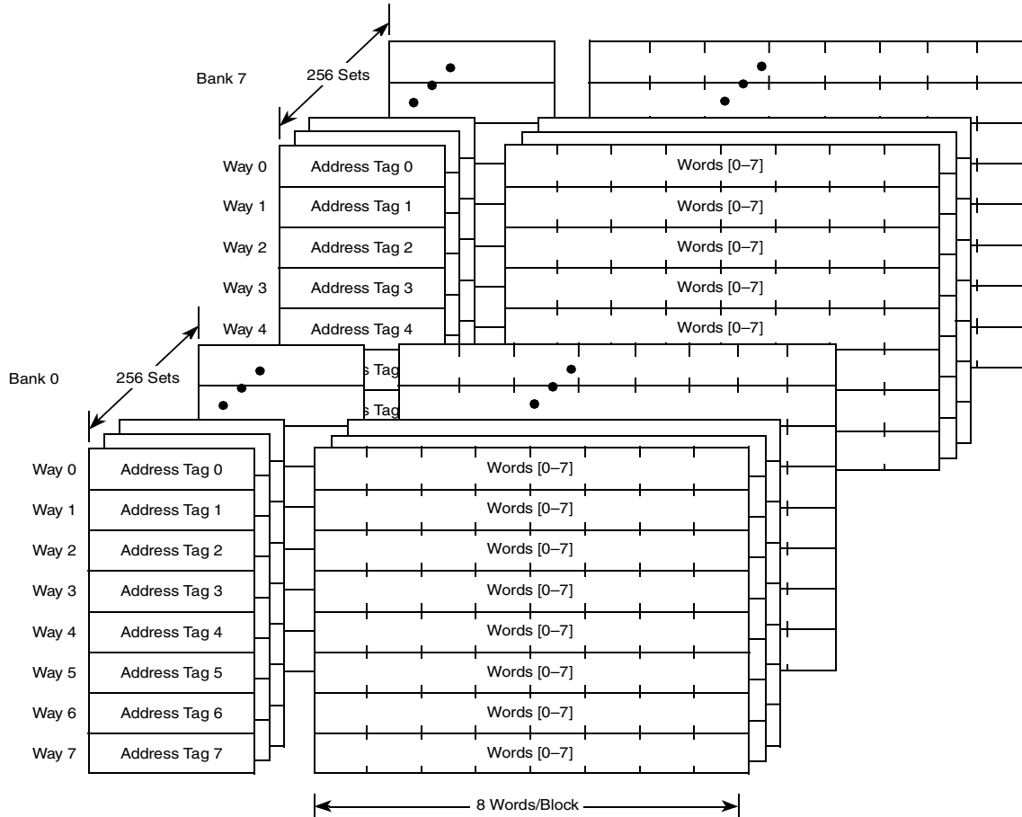
Figure 7-2. Cache Organization
