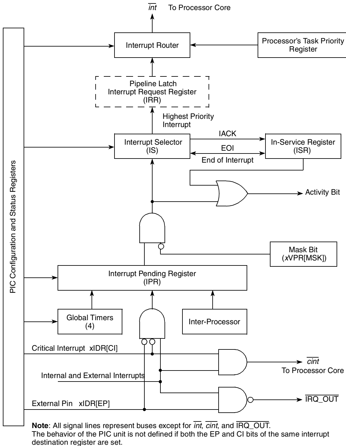
Figure 10-47. PIC Interrupt Processing Flow Diagram
