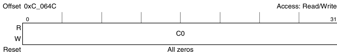
Figure 17-34. Packet/Control Symbol Error Capture Command and Status Register 0 (PCSECSR0)
