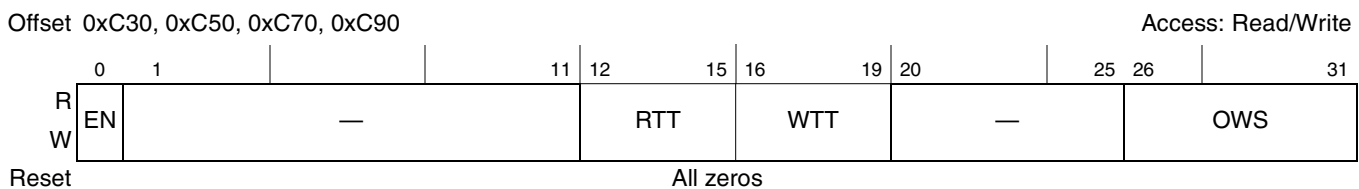
Figure 16-10. PCI/X Outbound Window 1–4 Attributes Registers (POWAR1–POWAR4)
