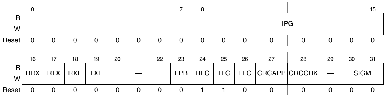
Figure 14-107. FIFOCFG Register Definition
