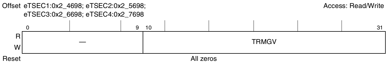
Figure 14-63. Transmit and Received 1519- to 1522-Byte VLAN Frame Register Definition
