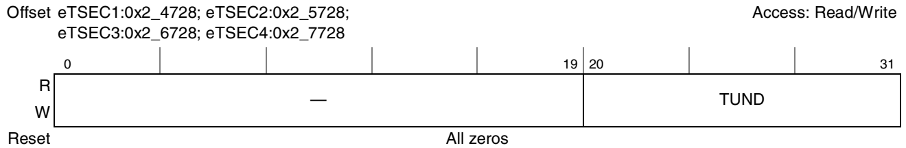
Figure 14-98. Transmit Undersize Frame Counter Register Definition
