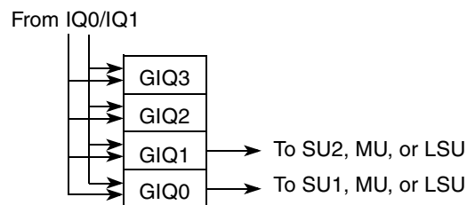
Figure 5-6. GPR Issue Queue (GIQ)
