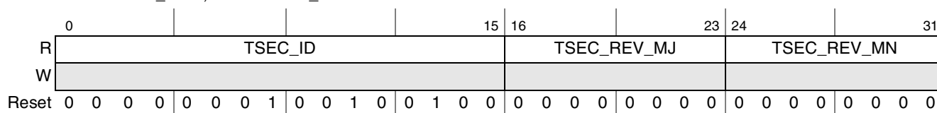
Figure 14-2. TSEC_ID Register
