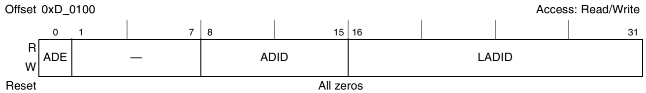
Figure 17-44. Alternate Device ID Command and Status Register (ADIDCSR)
