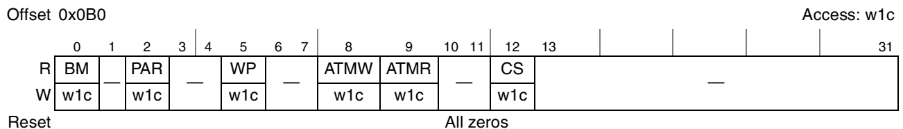
Figure 13-13. Transfer Error Status Register (LTESR)
