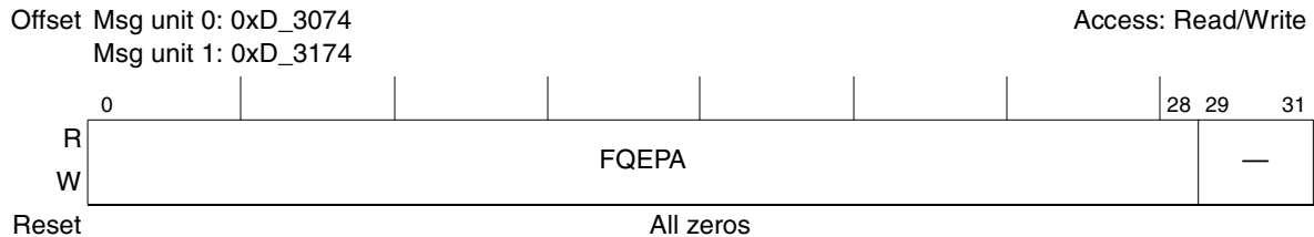
Figure 17-81. Inbound Message n Frame Queue Enqueue Pointer Address Registers (IM n FQEPAR)
