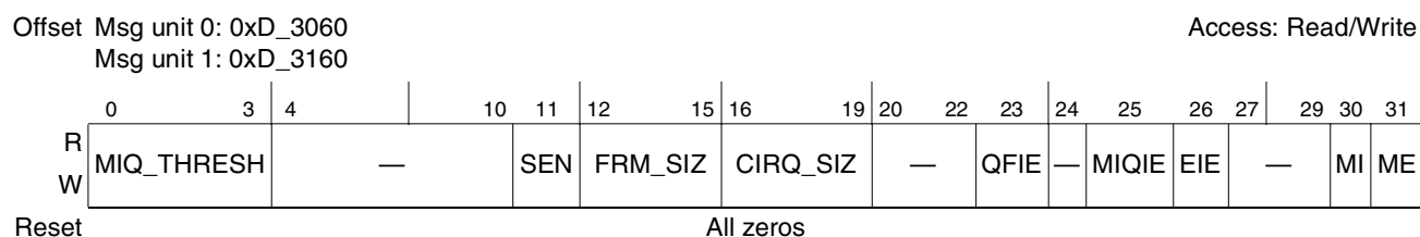
Figure 17-76. Inbound Message n Mode Registers (IM n MR)
