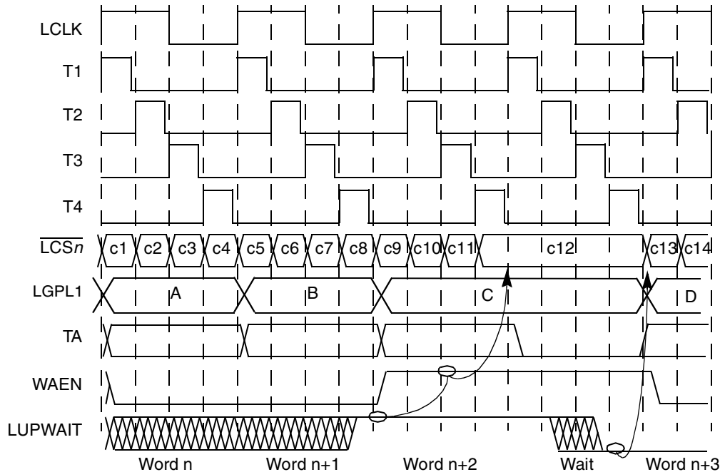
Figure 13-62. Effect of LUPWAIT Signal
