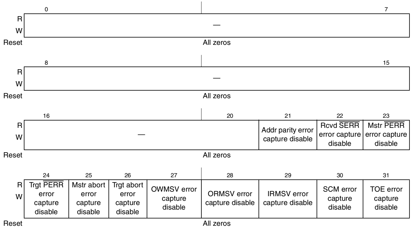
Figure 16-16. PCI/X Error Capture Disable Register (ERR_CAP_DR)
