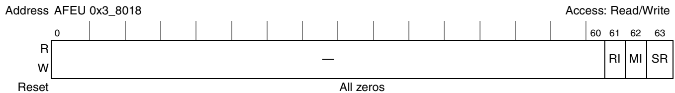
Figure 19-28. AFEU Reset Control Register
