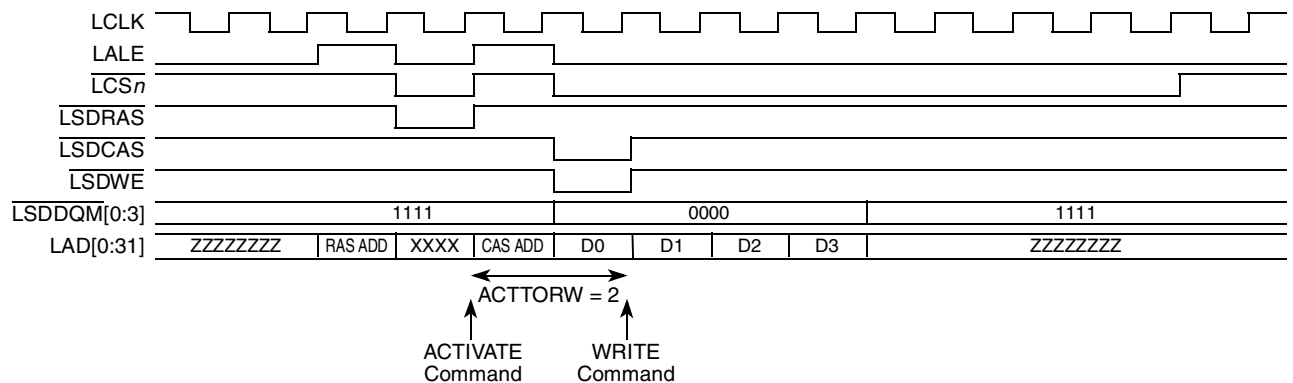
Figure 13-37. ACTTORW = 2 (2 Clock Cycles)
