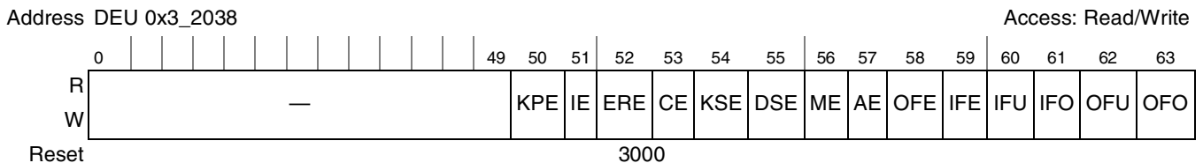
Figure 19-23. DEU Interrupt Control Register
