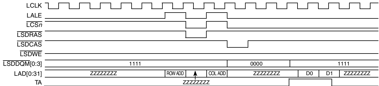
Figure 13-44. SDRAM Two-Beat Burst Read, Page Closed, CL = 3
