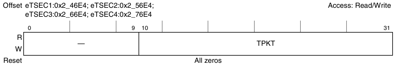
Figure 14-82. Transmit Packet Counter Register Definition
