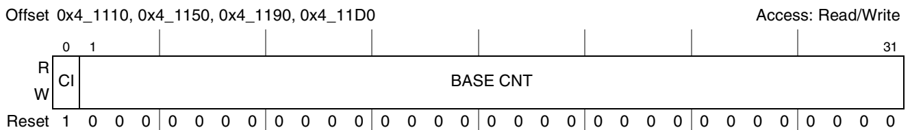
Figure 10-12. Global Timer Base Count Register (GTBCR n )
