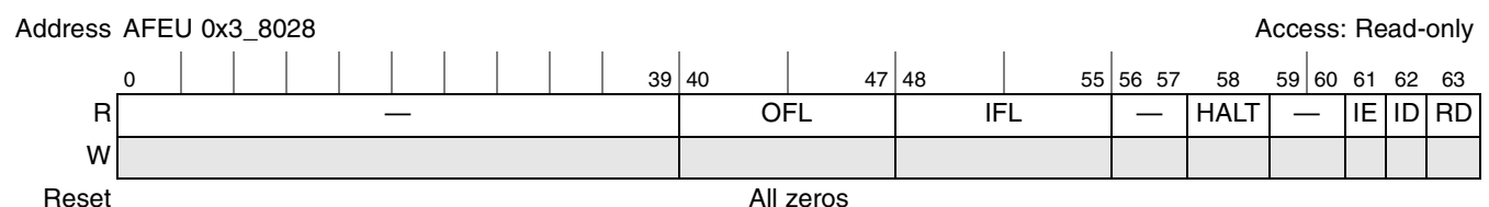
Figure 19-29. AFEU Status Register
