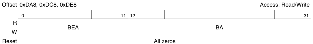
Figure 16-12. PCI/X Inbound Window Base Address Registers
