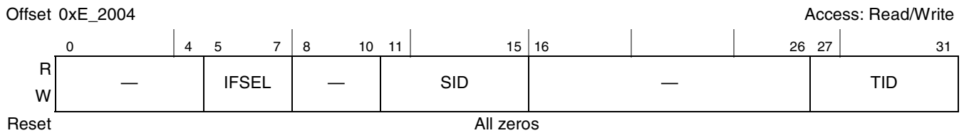
Figure 22-3. Watchpoint Monitor Control Register 1 (WMCR1)
