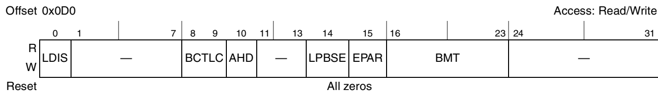
Figure 13-18. Local Bus Configuration Register
