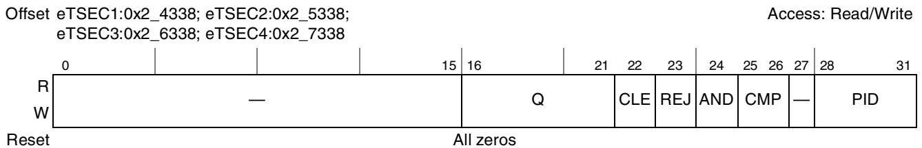
Figure 14-33. Receive Queue Filer Table Control Register Definition
