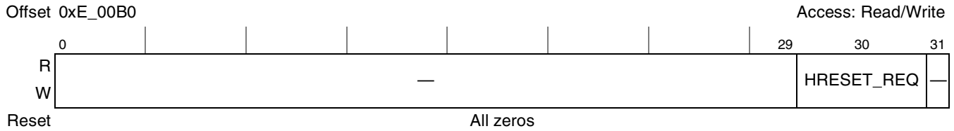
Figure 20-18. Reset Control Register (RSTCR)
