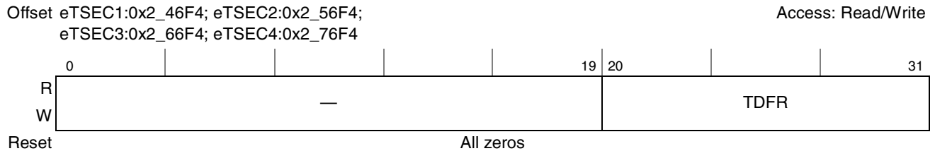
Figure 14-86. Transmit Deferral Packet Counter Register Definition
