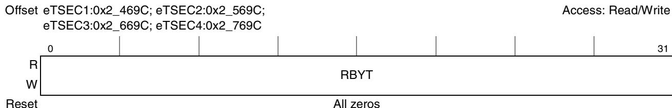
Figure 14-64. Receive Byte Counter Register Definition
