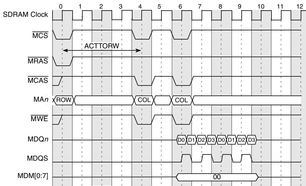
Figure 9-42. Registered DDR SDRAM DIMM Burst Write Timing
