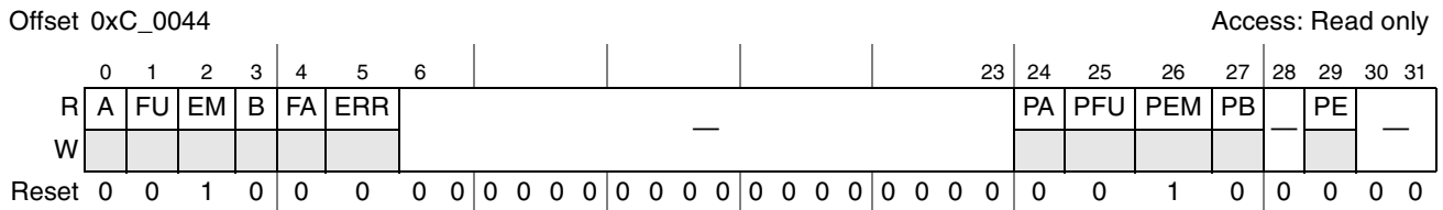
Figure 17-10. Port-Write and Doorbell Command and Status Register (PWDCSR)
