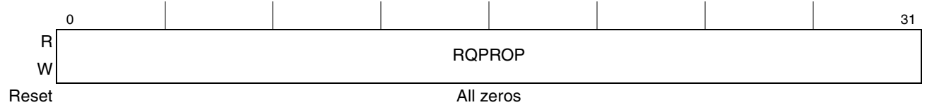
Figure 14-34. Receive Queue Filer Table Property IDs 0, 2–15 Register Definition
