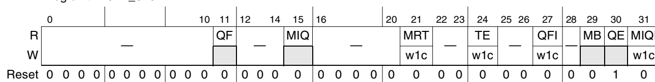
Figure 17-77. Inbound Message n Status Registers (IM n SR)
