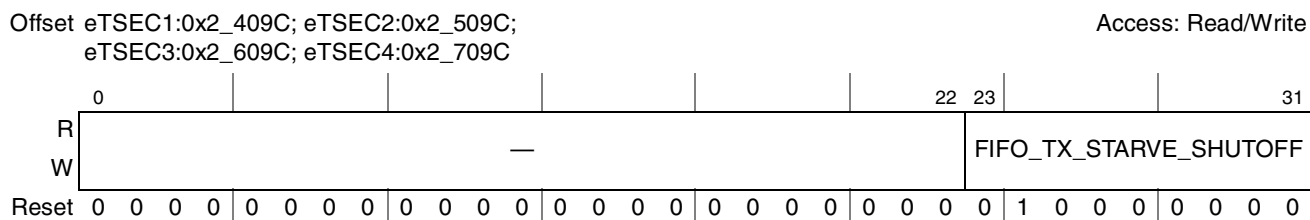
Figure 14-15. FIFO_TX_STARVE_SHUTOFF Register Definition
