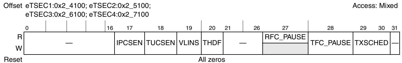
Figure 14-16. TCTRL Register Definition
