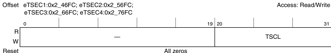
Figure 14-88. Transmit Single Collision Packet Counter Register Definition
