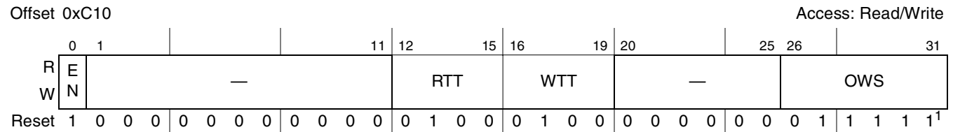
Figure 16-9. PCI/X Outbound Window 0 (Default) Attributes Register (POWAR0)
