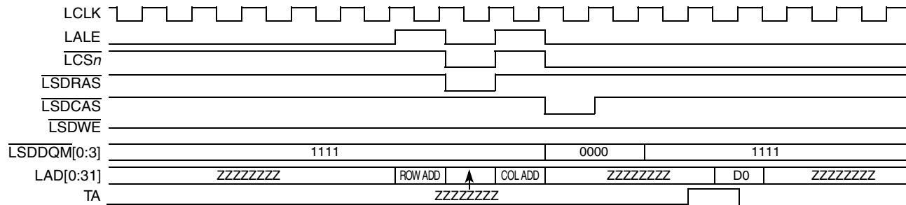
Figure 13-42. SDRAM Single-Beat Read, Page Closed, CL = 3
