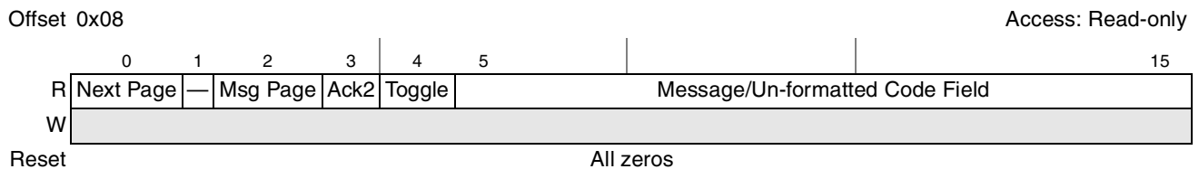
Figure 14-116. AN Link Partner Ability Next Page Register Definition
