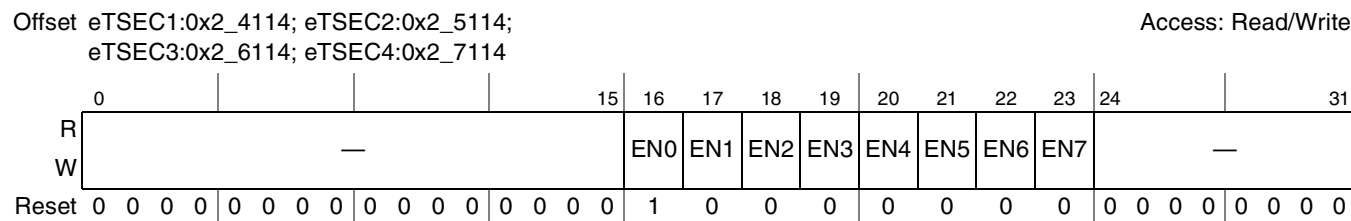
Figure 14-20. TQUEUE Register Definition
