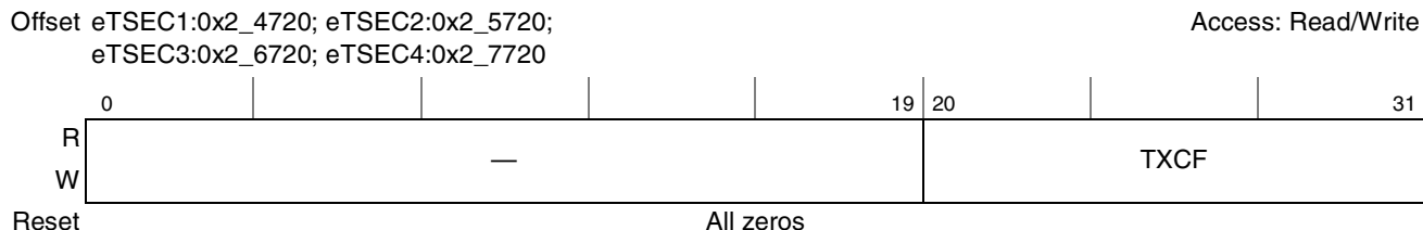
Figure 14-96. Transmit Control Frame Counter Register Definition
