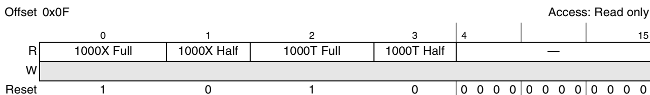
Figure 14-117. Extended Status Register Definition
