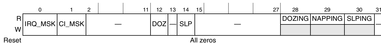
Figure 20-13. Power Management Control and Status Register (POWMGTCSR)
