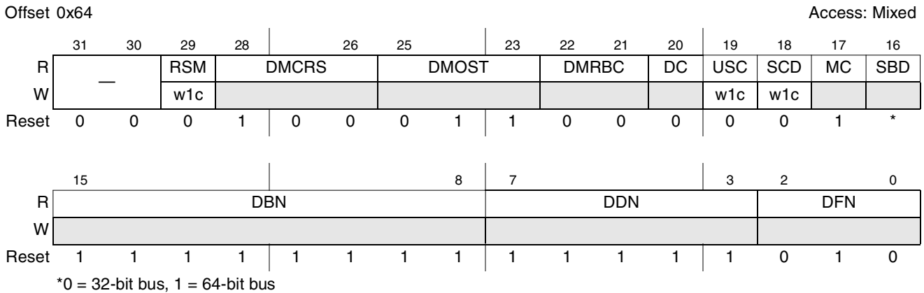
Figure 16-53. PCI-X Status Register
