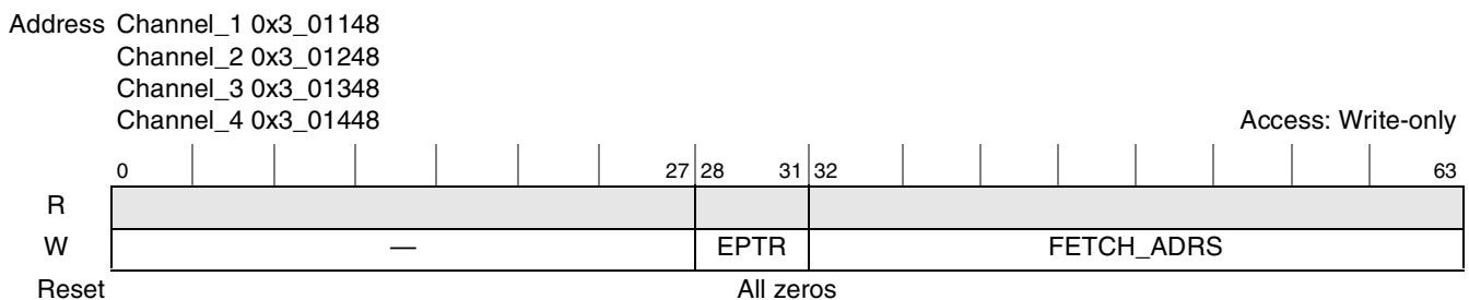
Figure 19-80. Fetch FIFO
