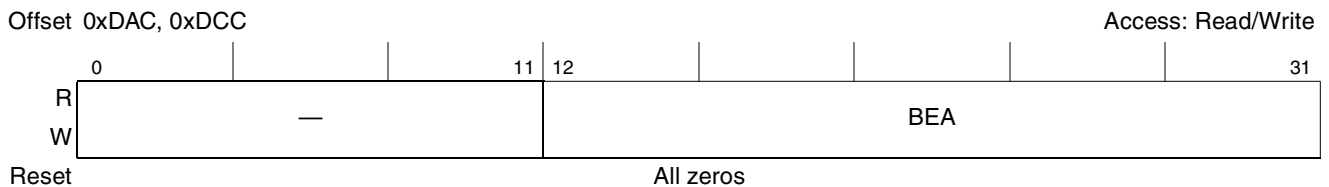
Figure 16-13. PCI/X Inbound Window Base Extended Address Registers (PIWBEAR n )
