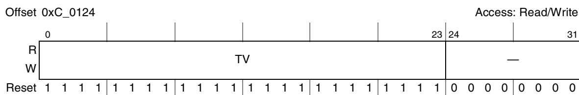
Figure 17-18. Port Response Time-Out Control Command and Status Register (PRTOCCSR)
