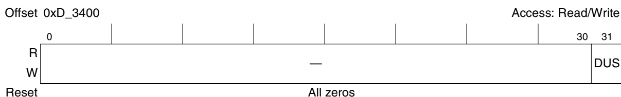
Figure 17-83. Outbound Mode Register (ODMR)
