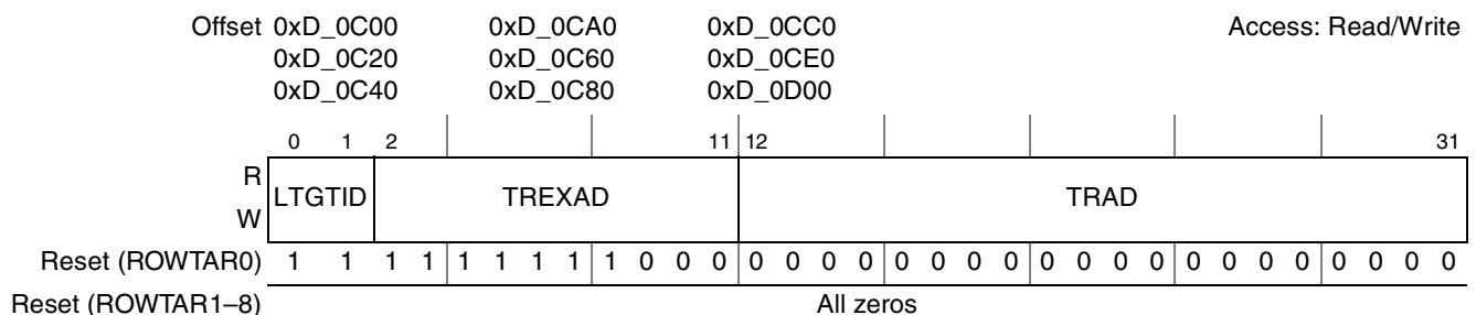
Figure 17-55. RapidIO Outbound Window Translation Address Registers 0–8 (ROWTAR n )
