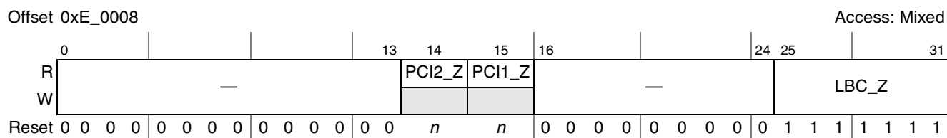
Figure 20-3. POR I/O Impedance Status and Control Register (PORIMPSCR)
