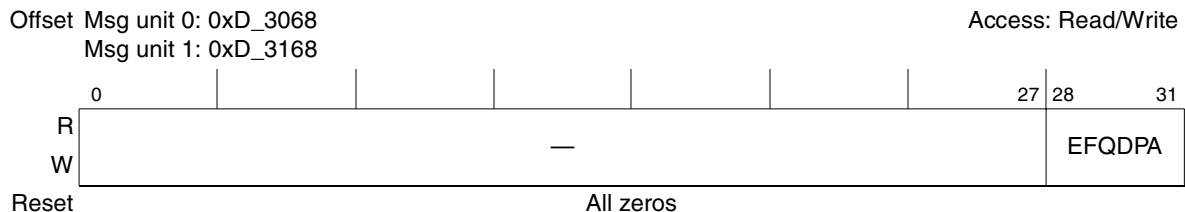
Figure 17-78. Extended Inbound Message n Frame Queue Dequeue Pointer Address Registers (EIMnFQDPAR)
