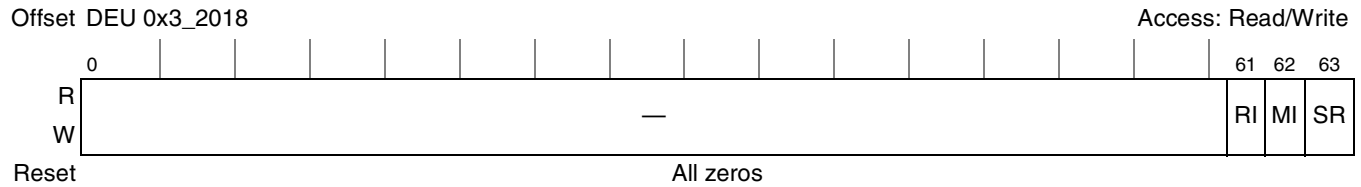
Figure 19-20. DEU Reset Control Register
