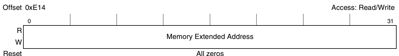
Figure 16-20. PCI/X Error Extended Address Capture Register (ERR_EXT_ADDR)
