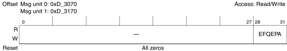
Figure 17-80. Extended Inbound Message n Frame Queue Enqueue Pointer Address Registers (EIM n FQEPAR)
