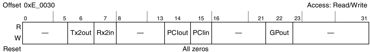
Figure 20-8. General-Purpose I/O Control Register (GPIOCR)
