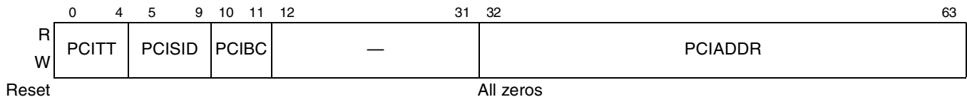
Figure 22-22. PCI Trace Buffer Entry
