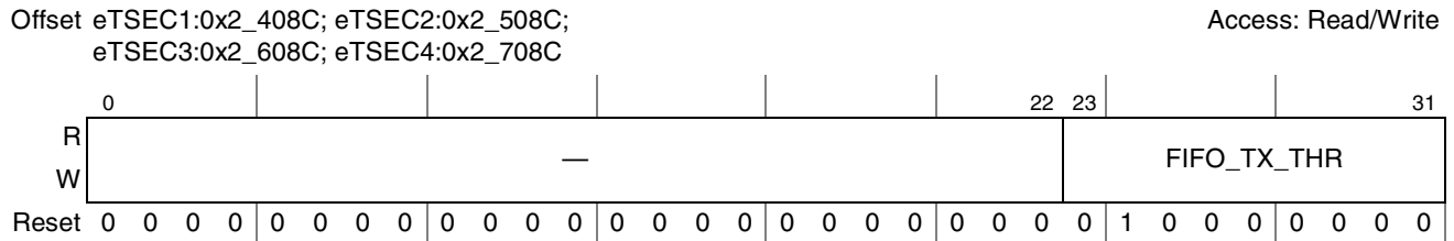
Figure 14-13. FIFO_TX_THR Register Definition
