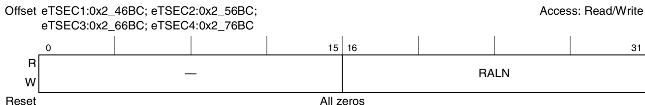
Figure 14-72. Receive Alignment Error Counter Register Definition
