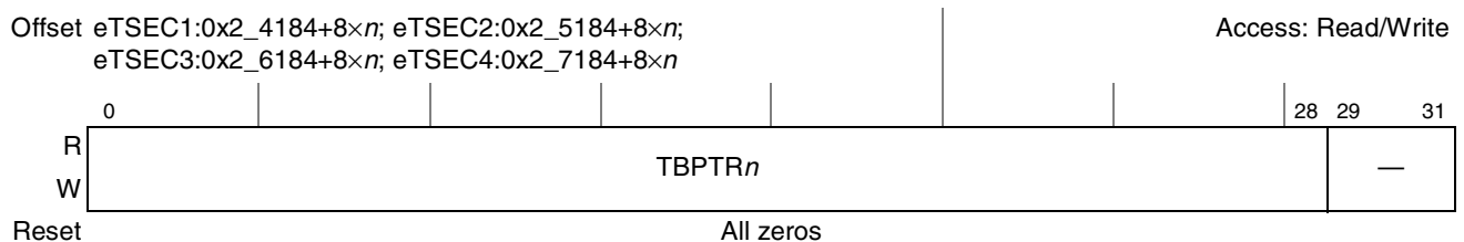
Figure 14-24. TBPTR0–TBPTR7 Register Definition
