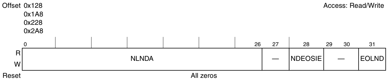
Figure 15-16. Next Link Descriptor Address Registers (NLNDAR n )
