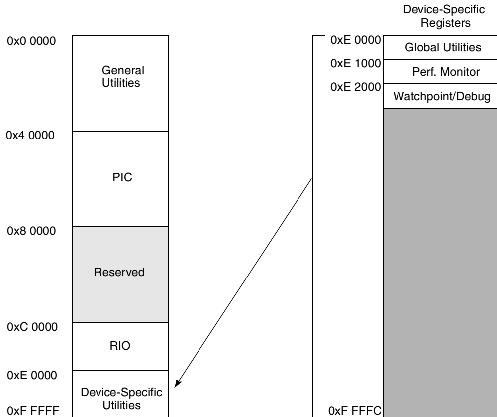
Figure 2-10. Device-Specific Register Mapping to Configuration, Control, and Status Memory Block
