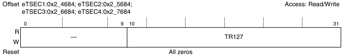
Figure 14-58. Transmit and Receive 65- to 127-Byte Frame Register Definition
