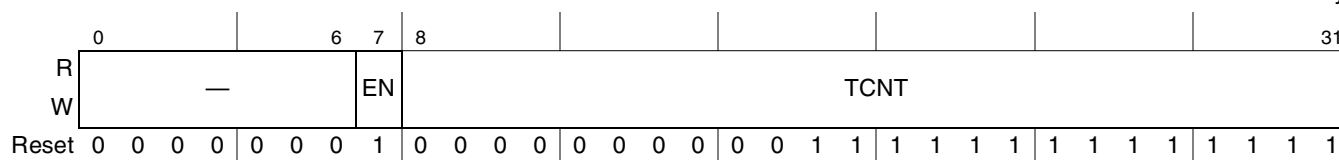
Figure 16-24. PCI-X Split Completion Timer Register (PCIX_TIMR)
