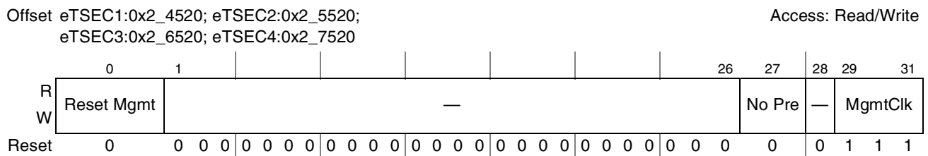
Figure 14-46. MII Management Configuration Register Definition
