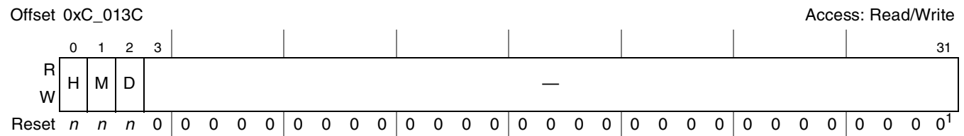
Figure 17-19. General Control Command and Status Register (GCCSR)
