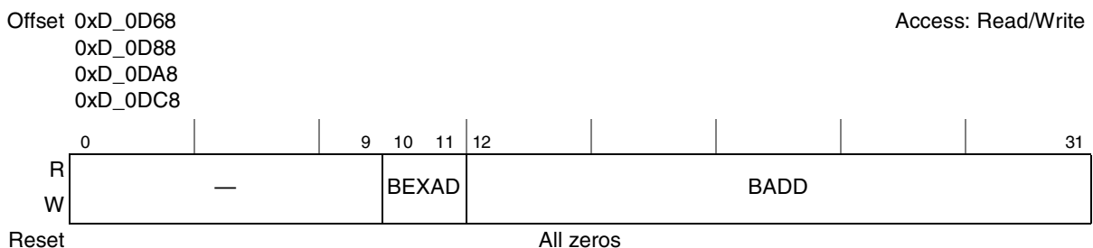
Figure 17-61. RapidIO Inbound Window Base Address Registers1–4
