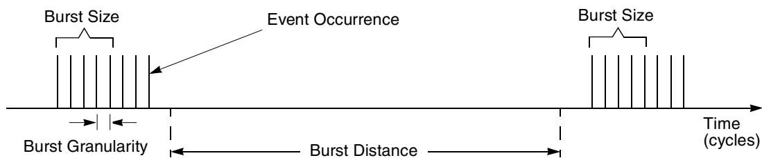
Figure 21-10. Burst Size, Distance, Granularity, and Burstiness Counting
