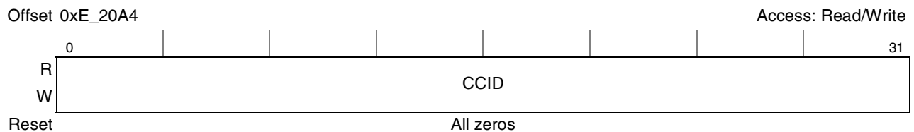
Figure 22-18. Current Context ID Register (CCIDR)
