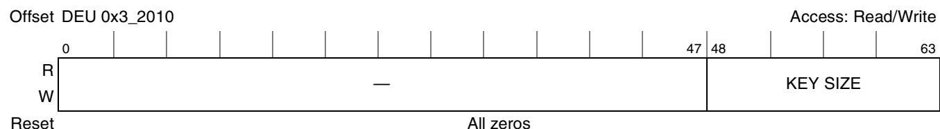
Figure 19-19. DEU Data Size Register
