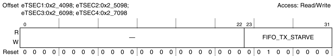
Figure 14-14. FIFO_TX_STARVE Register Definition
