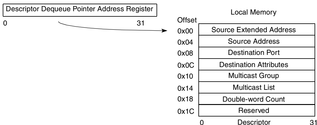
Figure 17-100. Descriptor Dequeue Pointer and Descriptor
