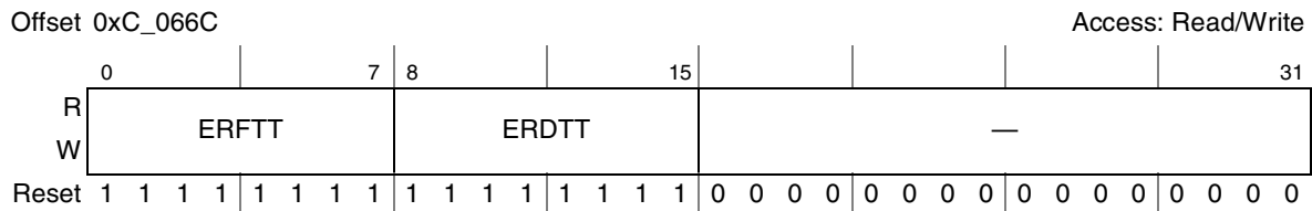
Figure 17-39. Error Rate Threshold Command and Status Register (ERTCSR)
