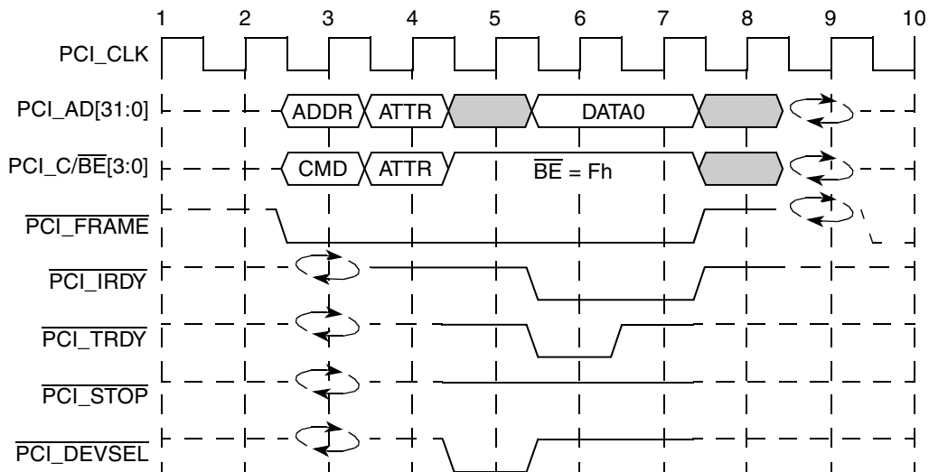
Figure 16-74. Split Response to a DWORD (4-Byte) Write Transaction
