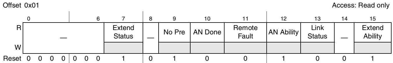
Figure 14-111. Status Register Definition
