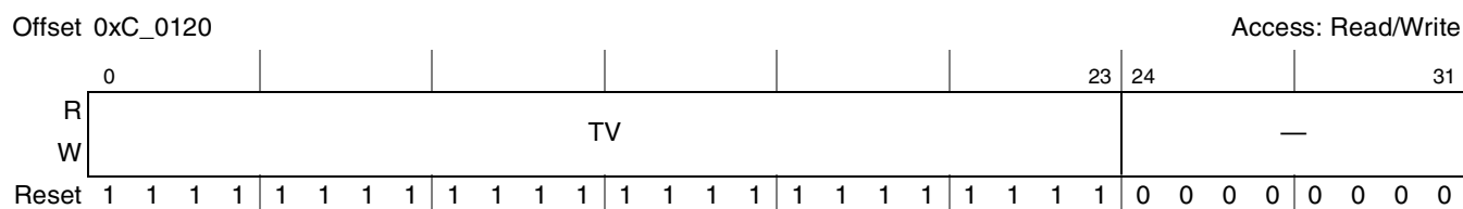
Figure 17-17. Port Link Time-Out Control Command and Status Register (PLTOCCSR)
