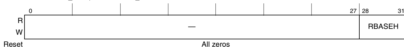
Figure 14-39. RBASEH Register Definition
