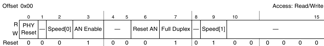
Figure 14-110. Control Register Definition
