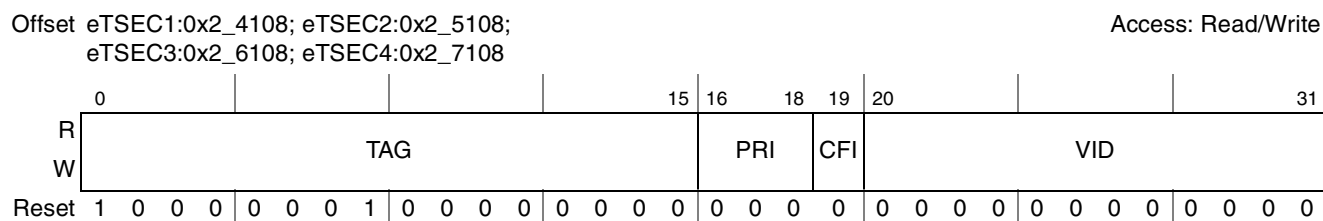
Figure 14-18. DFVLAN Register Definition
