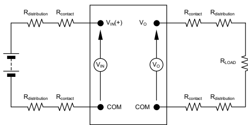
Figure 2. Output Ripple and Noise Test Setup.
