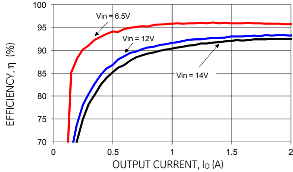
Figure 31. Converter Efficiency versus Output Current.
