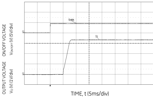
Figure 29. Typical Start-up Using On/Off Voltage (Io = Io,max, Vin=12V, Cext= 22uF)
