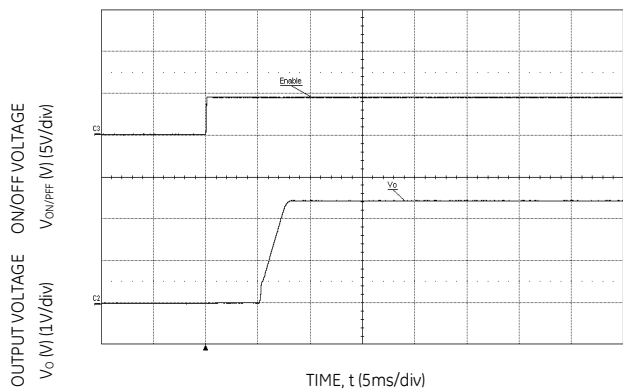
Figure 23. Typical Start-up Using On/Off Voltage (Io = Io,max, Vin=12V, Cext= 22uF).
