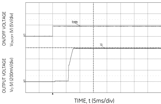
Figure 5. Typical Start-up Using On/Off Voltage (Io = Io,max, Vin=12V,Cext= 22uF).
