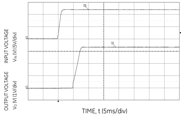
Figure 30. Typical Start-up Using Input Voltage (VIN = 12V, Cext= 22uF, Io = Io,max).
