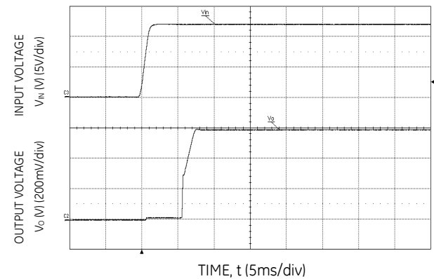
Figure 6. Typical Start-up Using Input Voltage (VIN = 12V, Cext= 22uF ,Io = Io,max).
