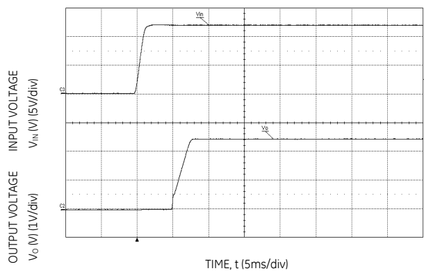
Figure 24. Typical Start-up Using Input Voltage (VIN = 12V, Cext= 22uF, Io = Io,max).
