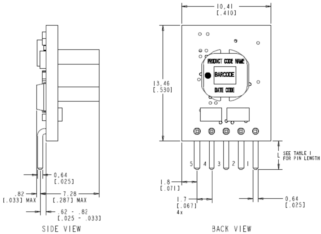
Pin Out
