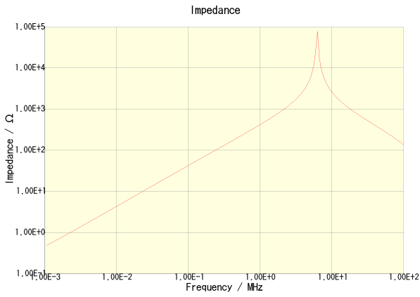
CLF12555T-680M-CA
