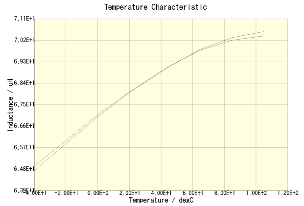
CLF12555T-680M-CA(DC = 0A)
