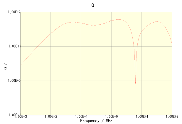
CLF12555T-680M-CA
