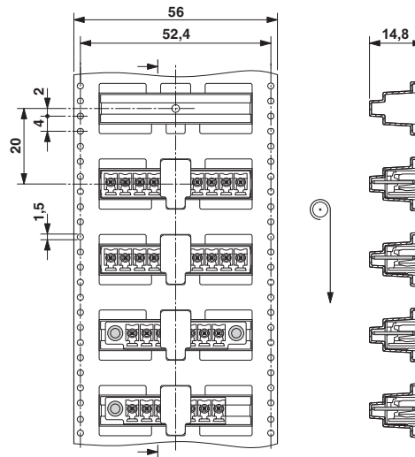
Dimensioned drawing
