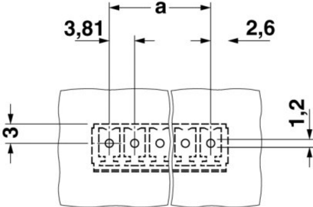
Drilling diagram
