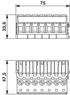
Contact insert
