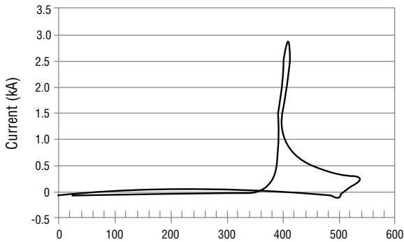
Surge Response - PTVS3-430C
