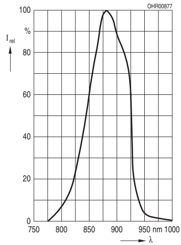
Relative Spectral Emission 2) page 13 Relative spektrale Emission 2) Seite 13 I_{rel} = f(\lambda) , T_A = 25^\circ\text{C}
