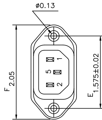
SUGGESTED MOUNTING CUTOUT (MOUNTING FROM FRONT)
