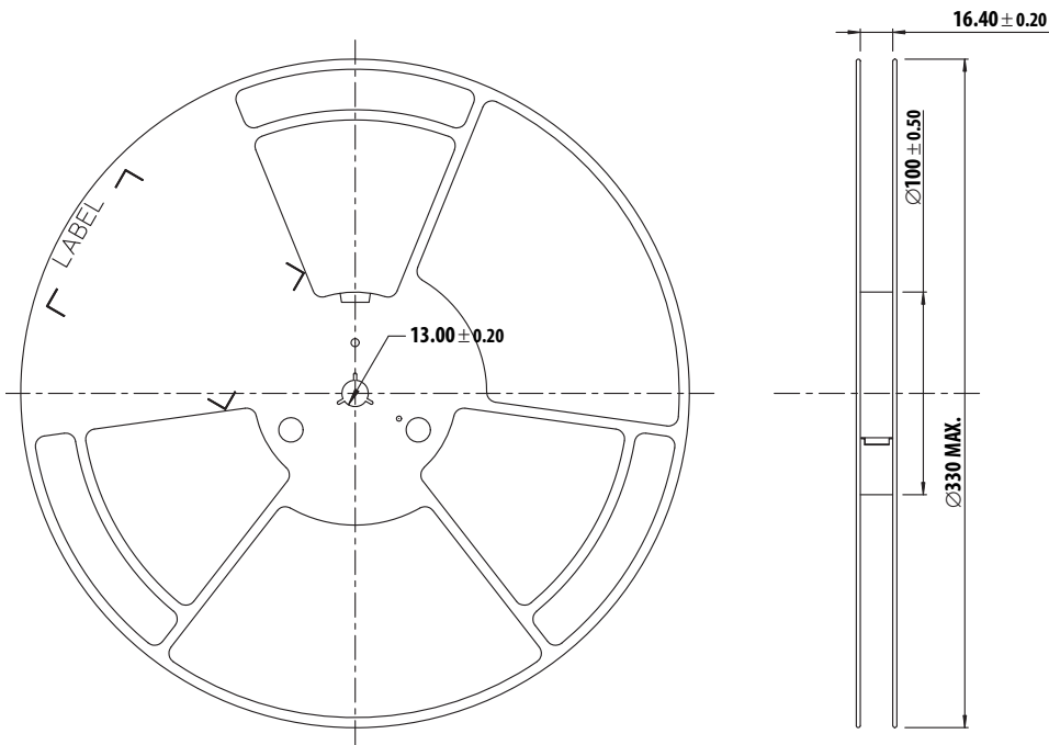
Figure 16. Reel Dimension
