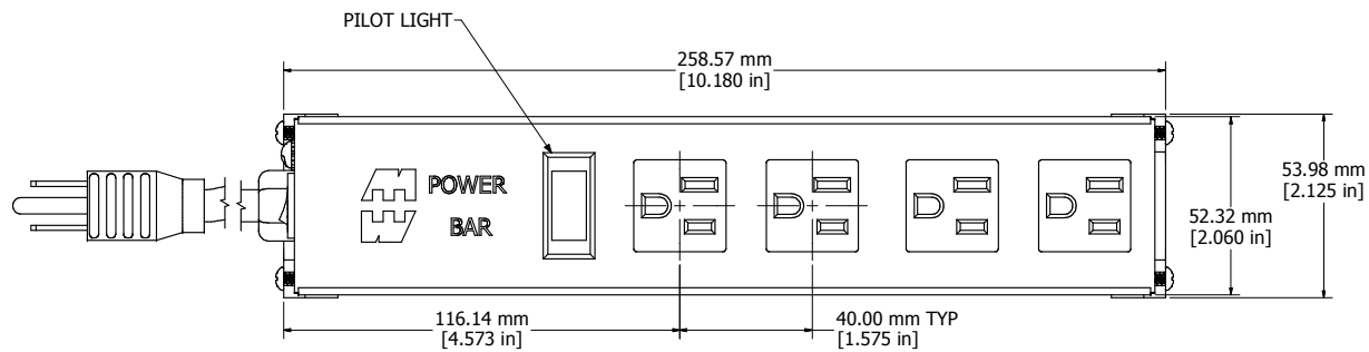
ASSEMBLY - VIEW FROM TOP
