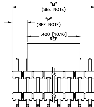
FIG. 5 (-M OPTION) (SEE NOTE 10)
