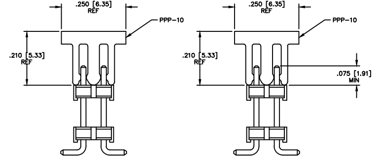
FIG. 5 (-M OPTION) (SEE NOTE 10)
