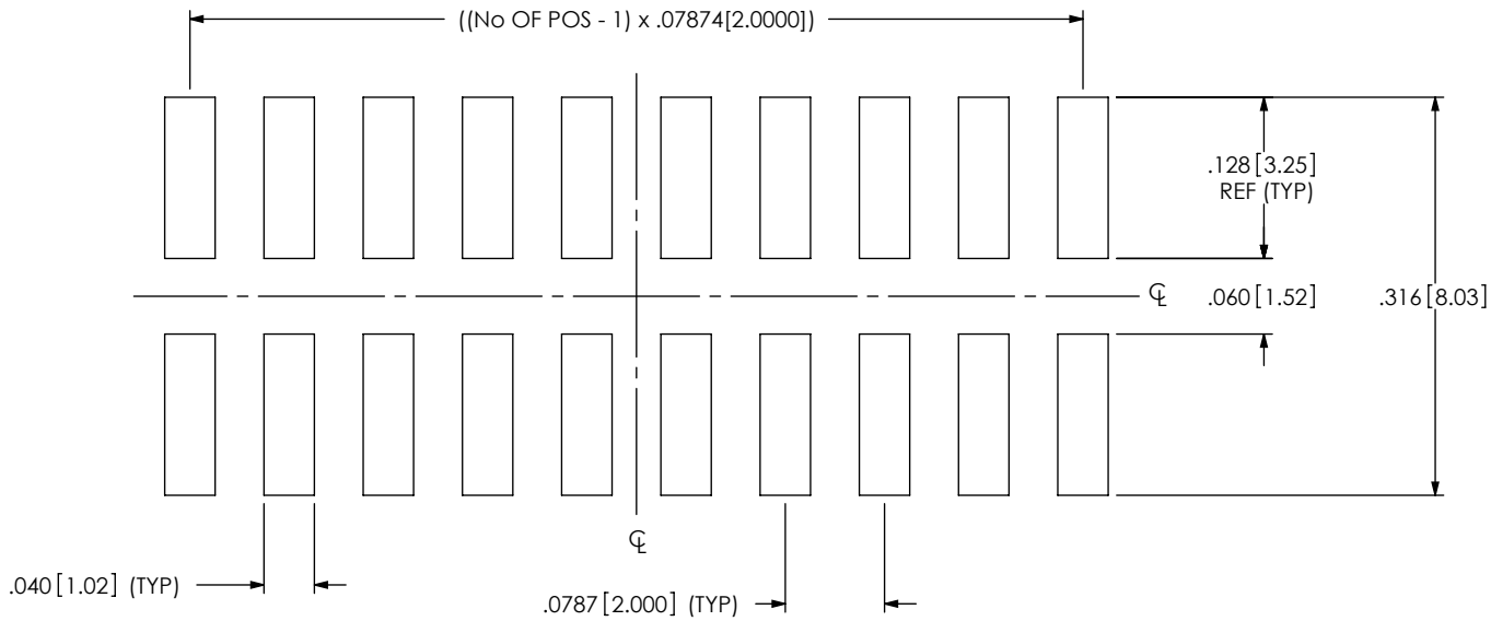
FIG 7 MMT-1XX-XX-XX-DV-XX SHOWN ALL DIMENSIONS ARE SYMMETRIC ABOUT THE CENTERLINE STENCIL TO BE .006[0.15] THICK
