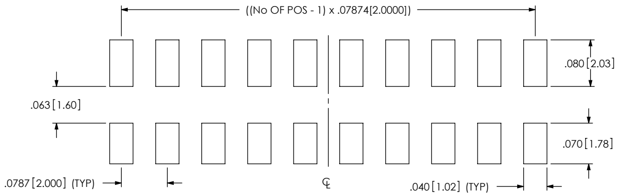
FIG 9 MMT-1XX-XX-XX-DH-XX SHOWN ALL DIMENSIONS ARE SYMMETRIC ABOUT THE CENTERLINE STENCIL TO BE .006[0.15] THICK
