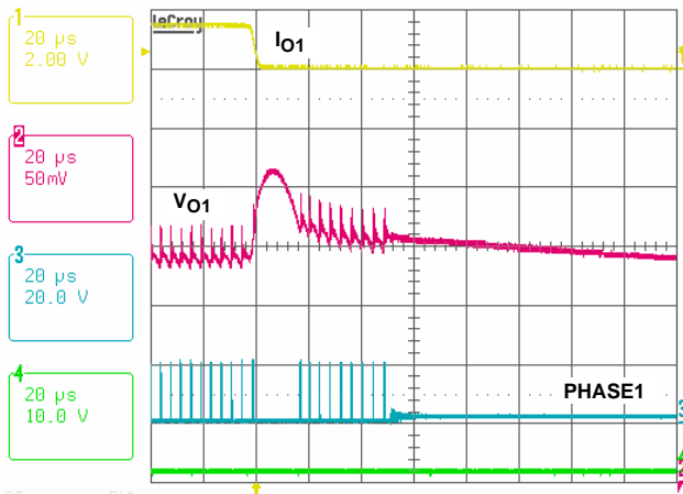
FIGURE 10. LOAD RELEASE RESPONSE, V_{IN} = 19V , V_O = 1.5V , I_O = 0.1A/8.1A @ 2.55A/\mu s
