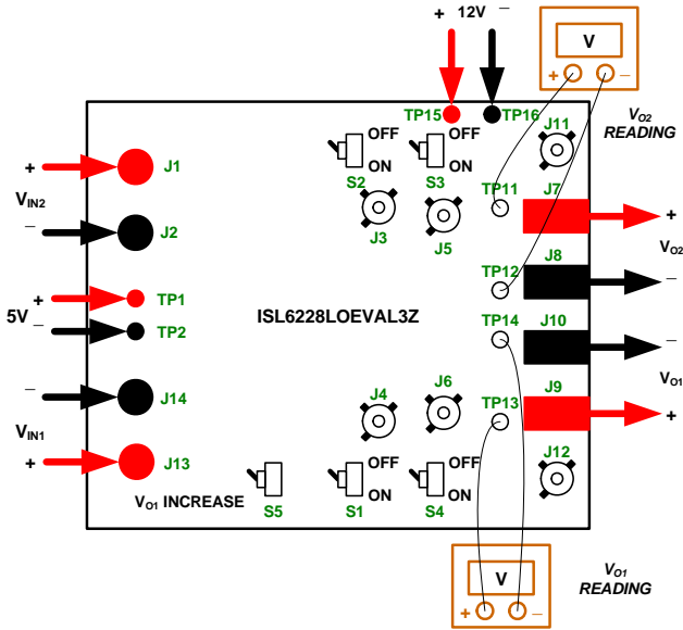
FIGURE 1. TEST SET-UP
