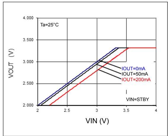
Figure 4. Output Voltage
