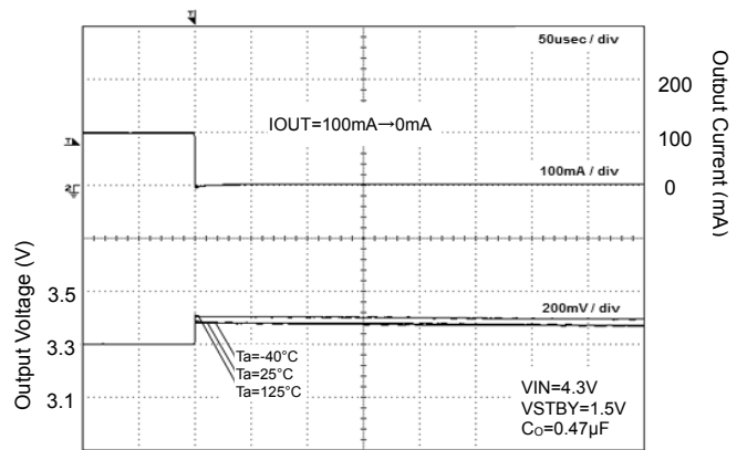
Figure 18. Load Response
