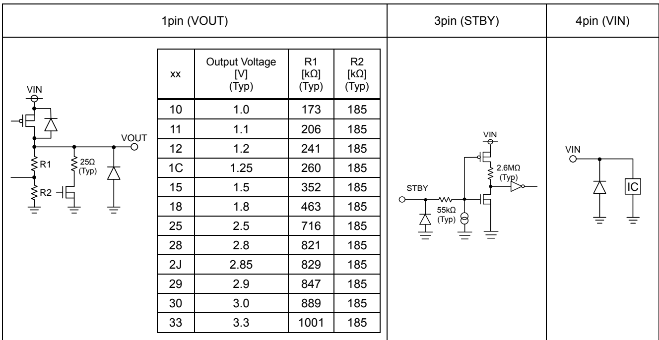
Figure 42. Input / Output equivalent circuit
