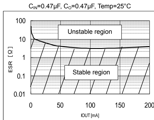
Figure 40. Stable region
