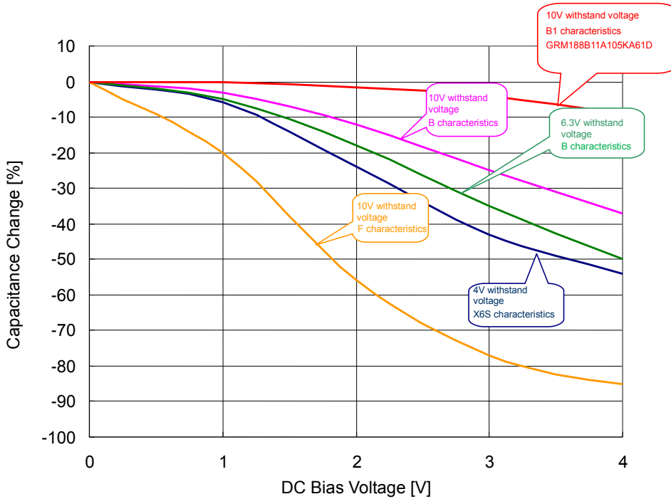
Figure 41. Capacity-bias characteristics (Characteristics Example)
