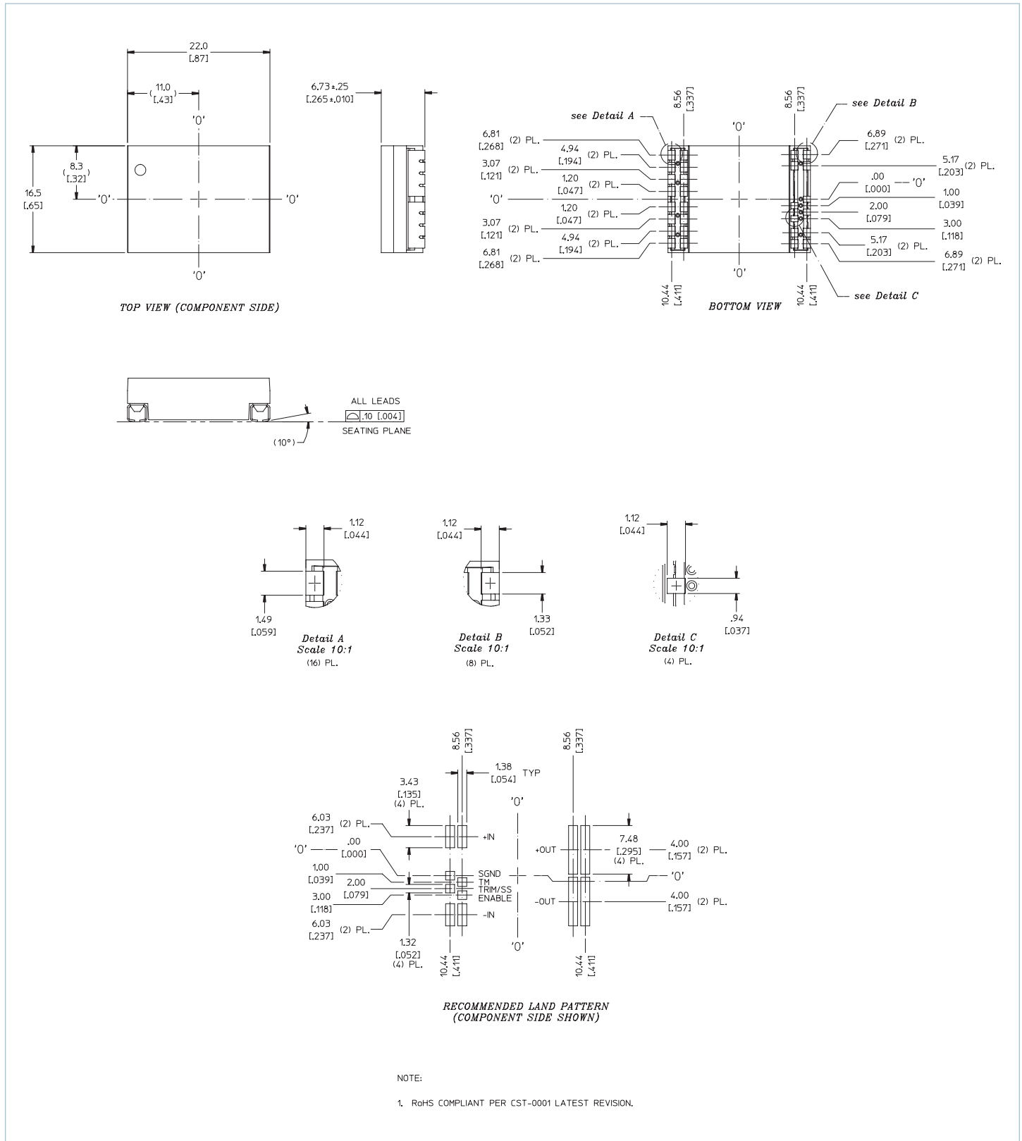
Figure 43 — Package Outline & Recommended PCB Land Pattern
