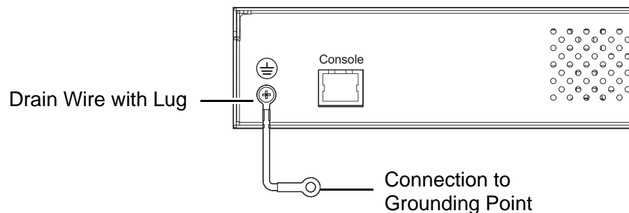
Figure 2.13 Grounding Connection
