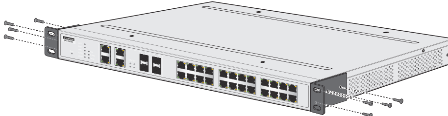
Figure 2.1 Installing the Rack Mount Brackets
