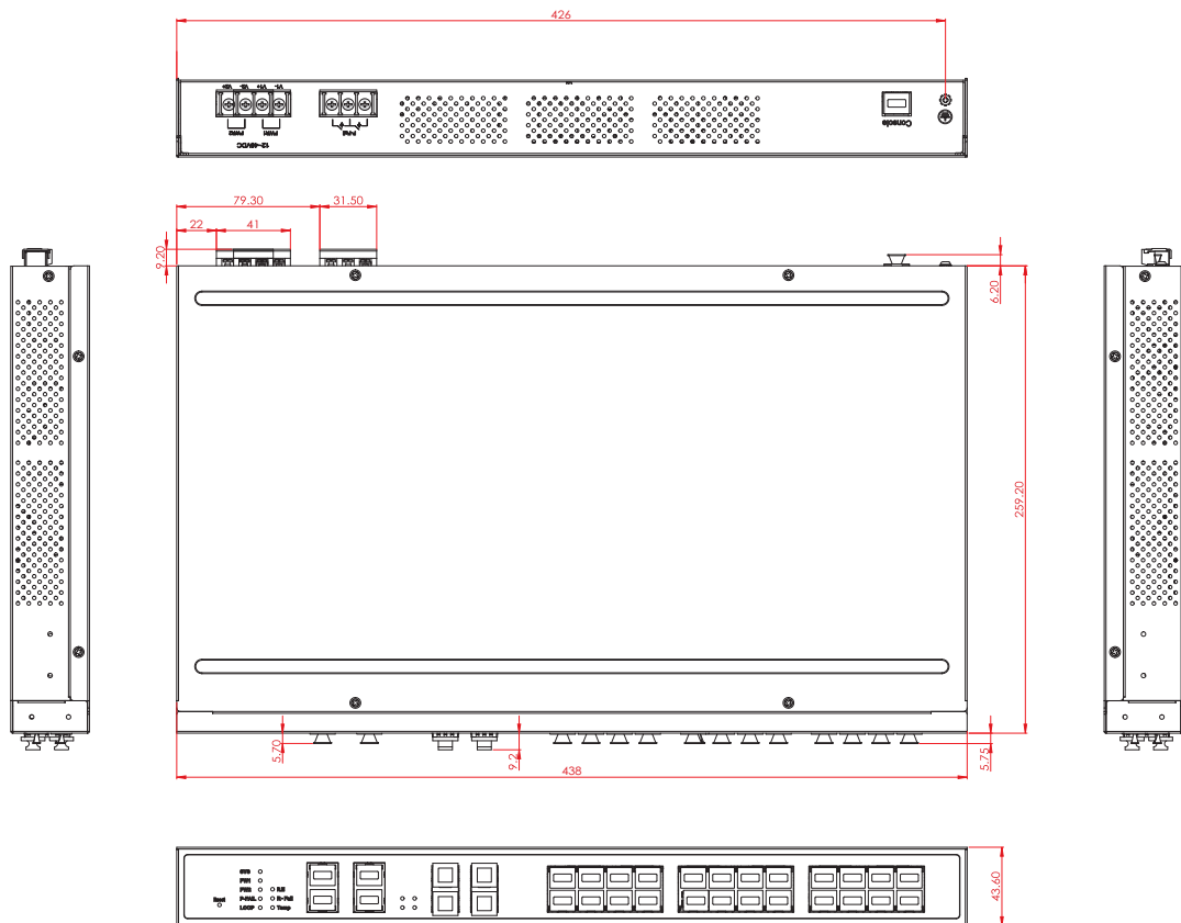
Figure 1.4 Dimensions
