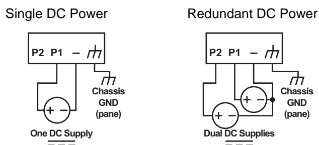
Figure 2.12 Power Wiring for EKI-9628G
