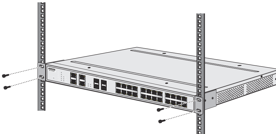
Figure 2.2 Installing the Switch
