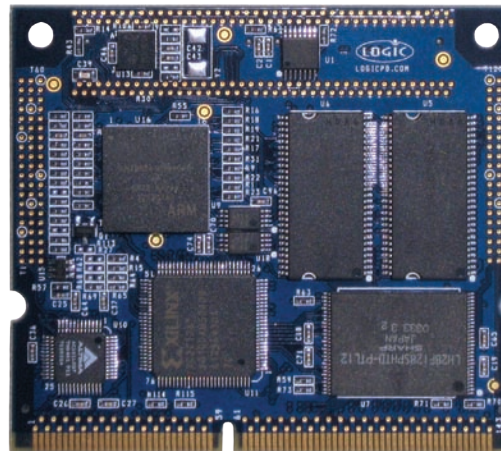
LH79524 CARD ENGINE
