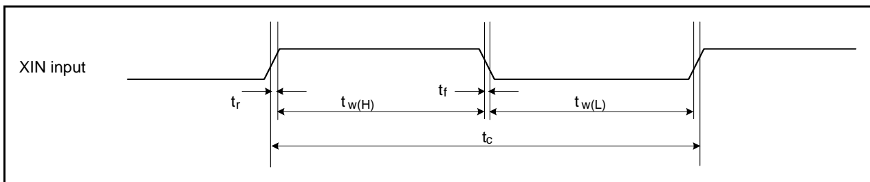
Figure 31.37 External Clock Input (XIN Input)
