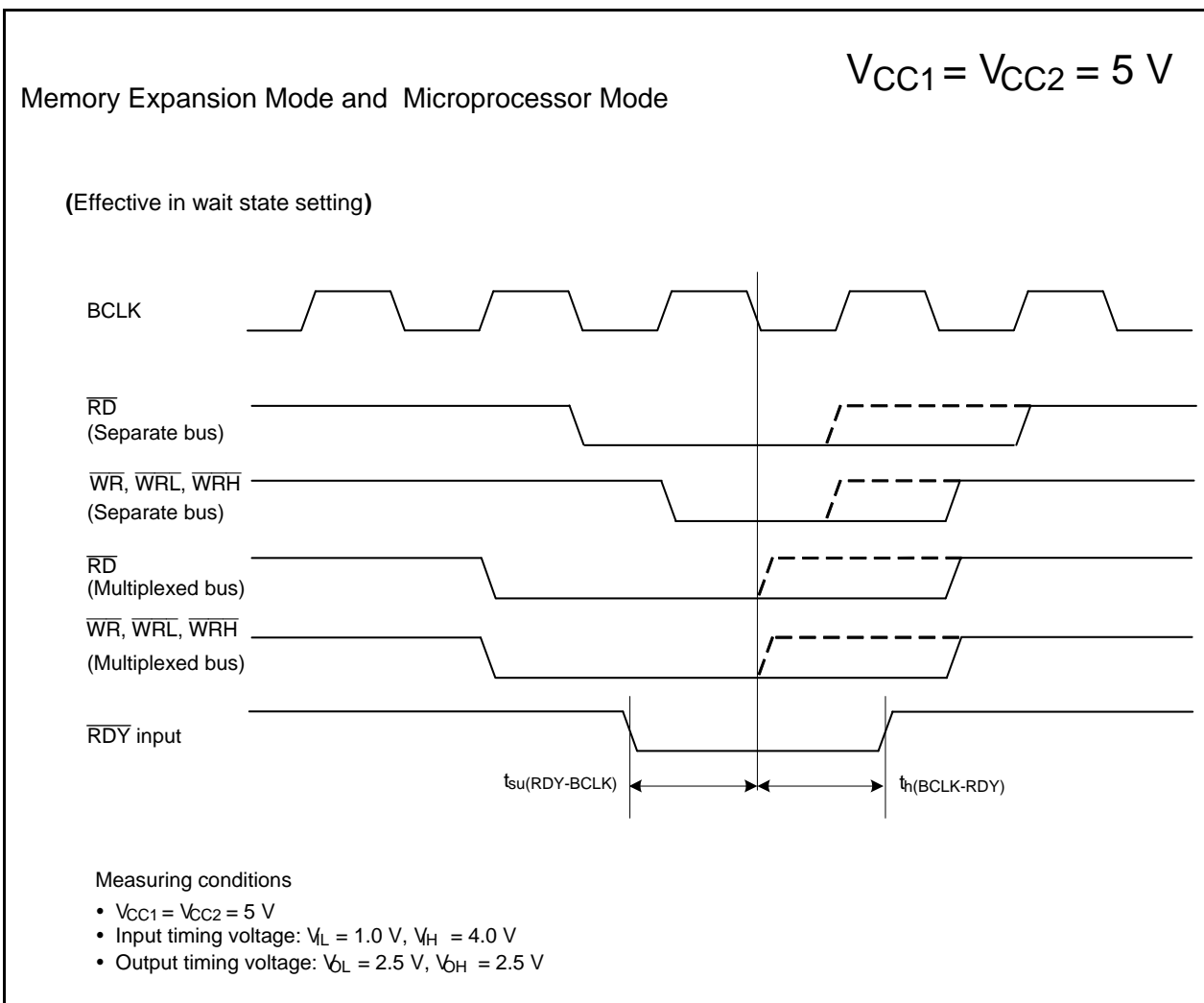
Figure 31.14 Timing Diagram
