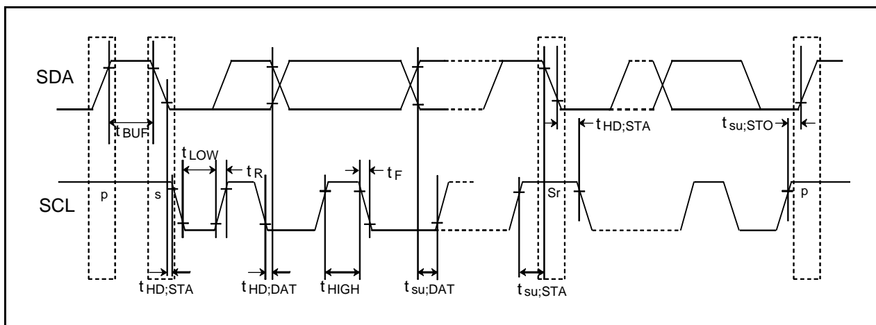
Figure 31.28 Multi-master I 2 C-bus
