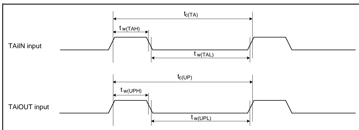
Figure 31.38 Timer A Input
