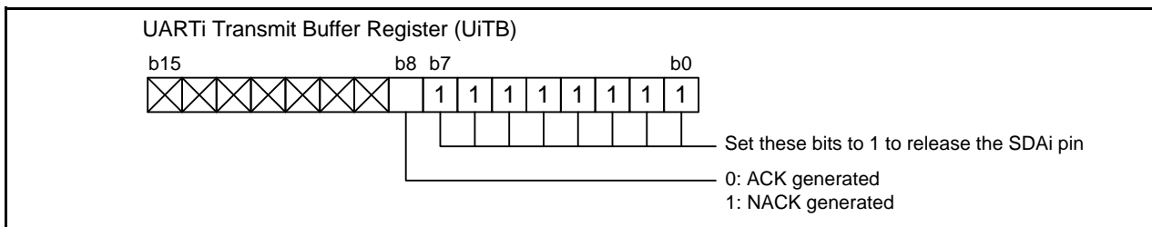
Figure 23.30 UiTB Register Setting (SDA Input)
