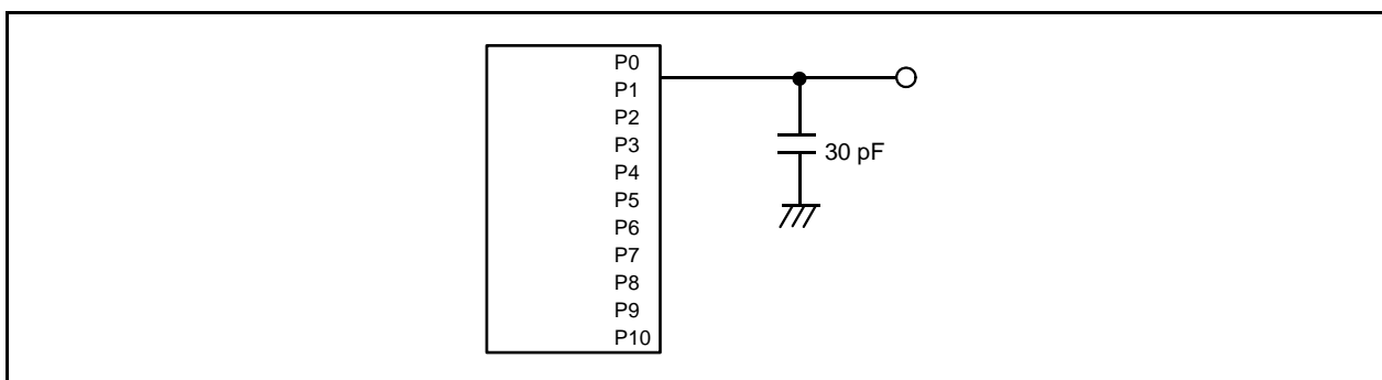
Figure 31.30 Ports P0 to P10 Measurement Circuit
