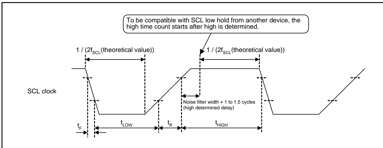
Figure 23.26 SCL Clock
