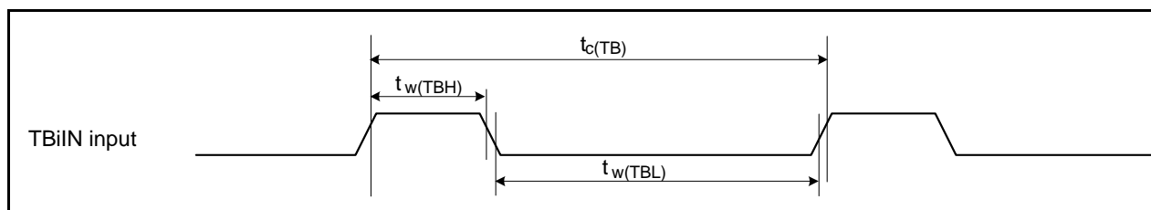
Figure 31.40 Timer B Input
