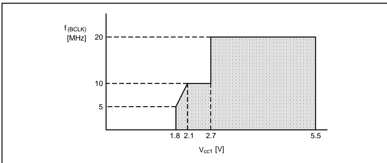
Figure 31.1 Relation between f_{(BCLK)} and V_{CC1}
