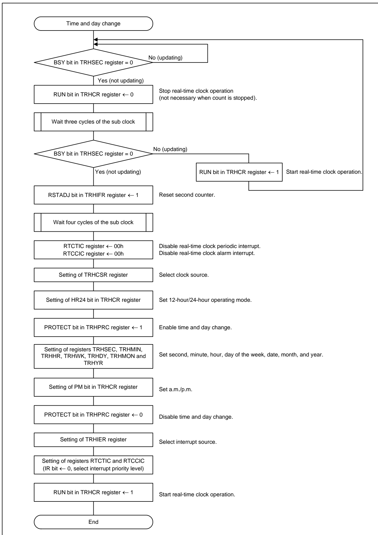
Figure 20.4 Procedure for Changing Time and Date
