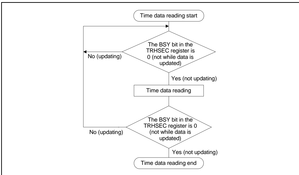
Figure 32.10 Time Data Reading
