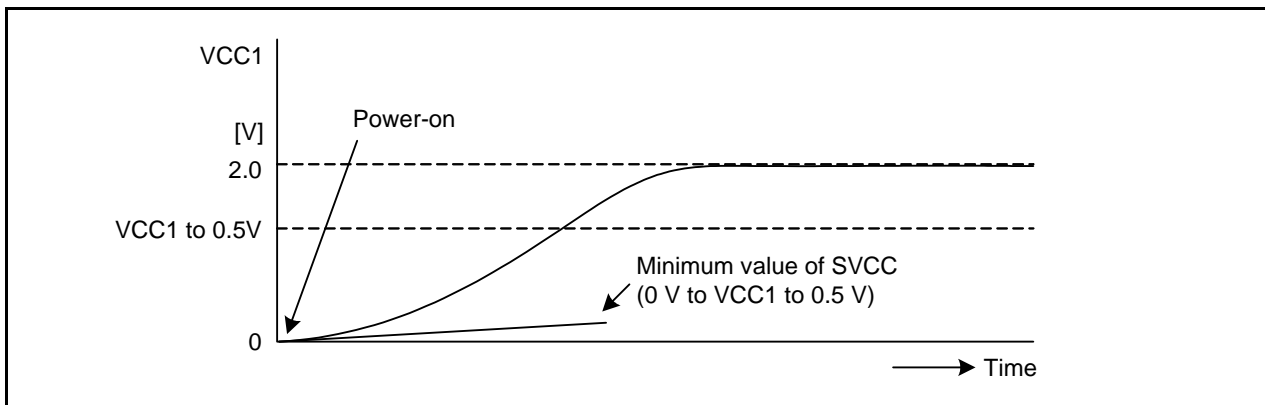
Figure 6.9 SVCC Timing ( 1.8\text{ V} \leq VCC1 < 2.2\text{ V} )
