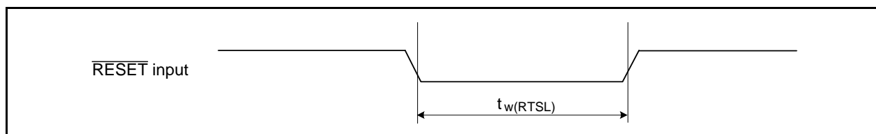
Figure 31.21 Reset Input ( \overline{\text{RESET}} Input)
