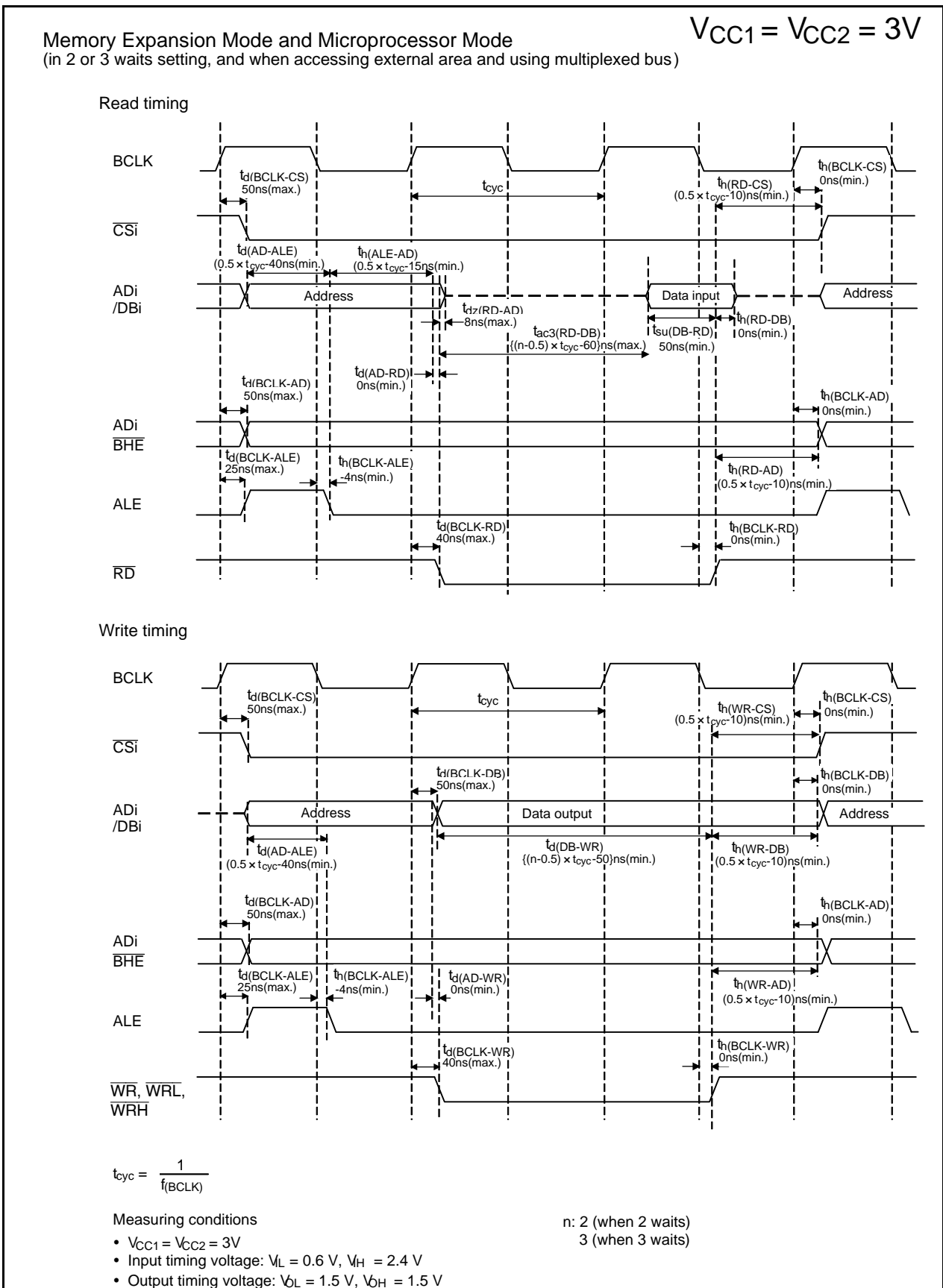
Figure 31.33 Timing Diagram
