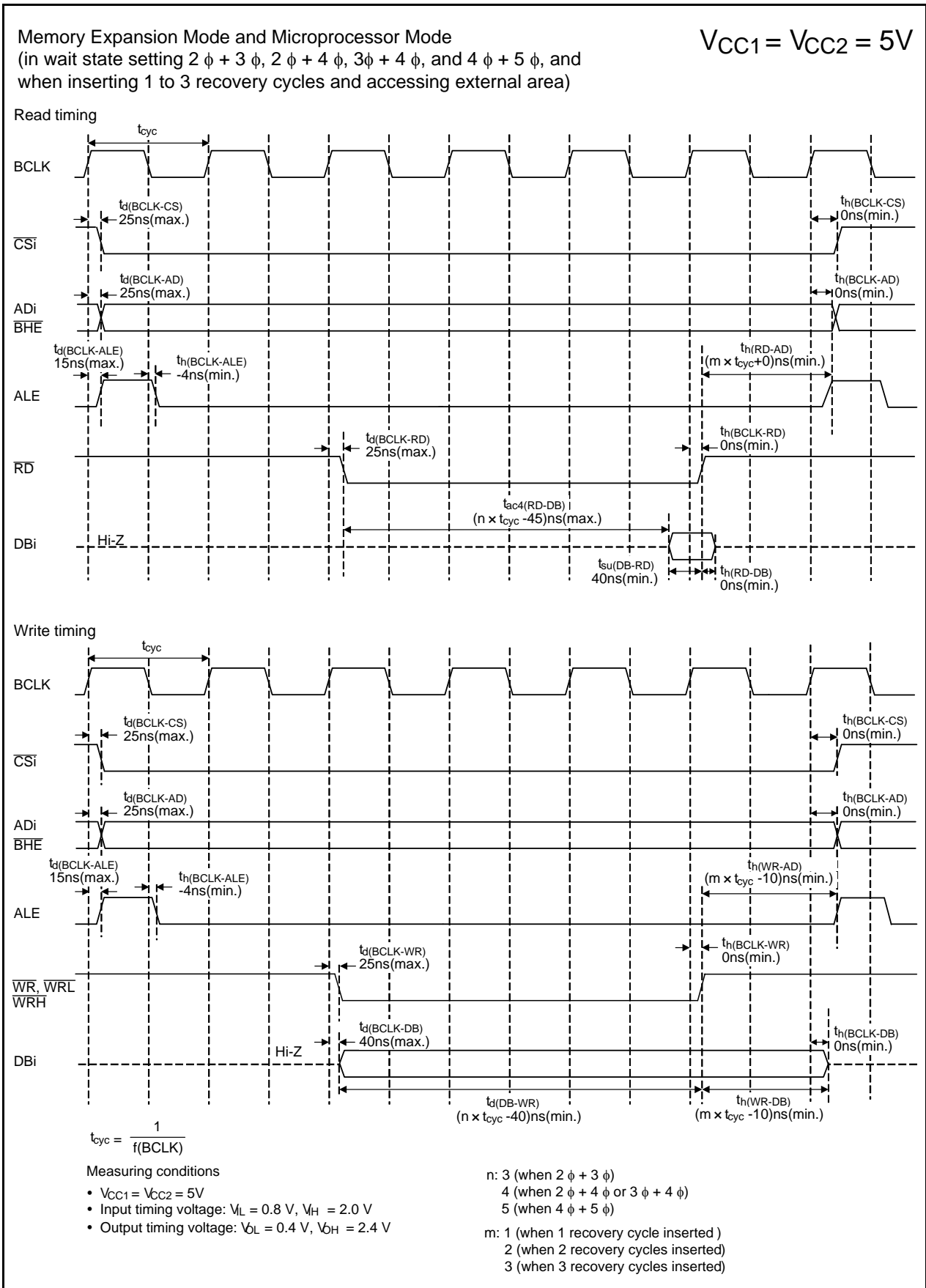
Figure 31.20 Timing Diagram
