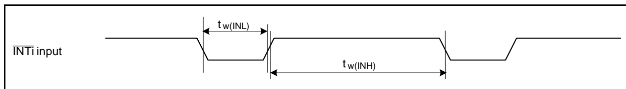
Figure 31.12 External Interrupt \overline{\text{INTi}} Input
