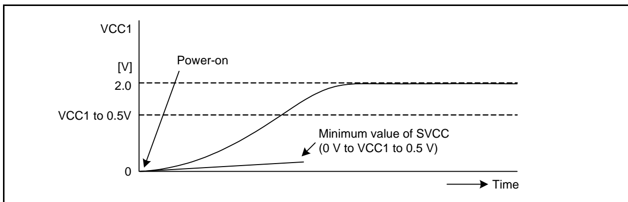
Figure 32.4 SVCC Timing ( 1.8\text{ V} \leq VCC1 < 2.2\text{ V} )
