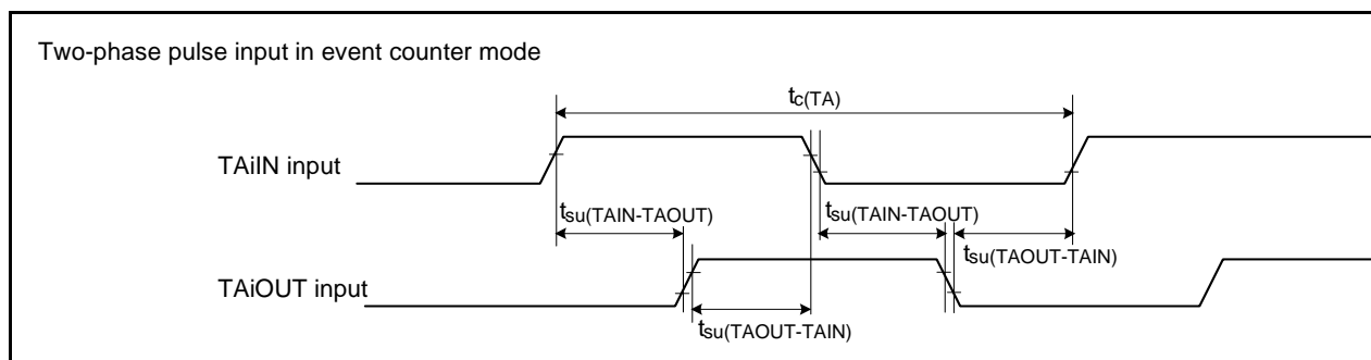
Figure 31.39 Timer A Input (Two-Phase Pulse Input in Event Counter Mode)
