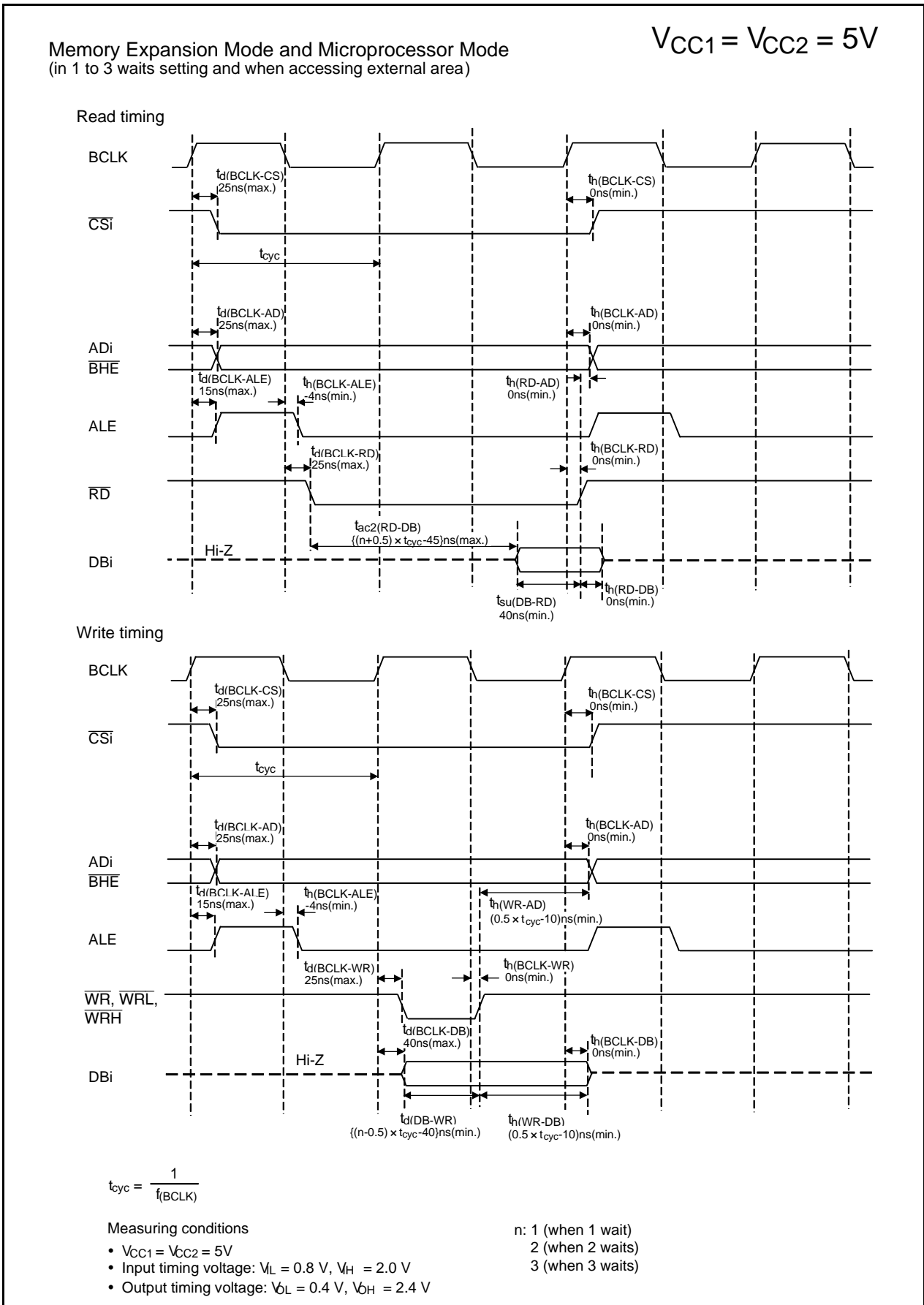
Figure 31.17 Timing Diagram
