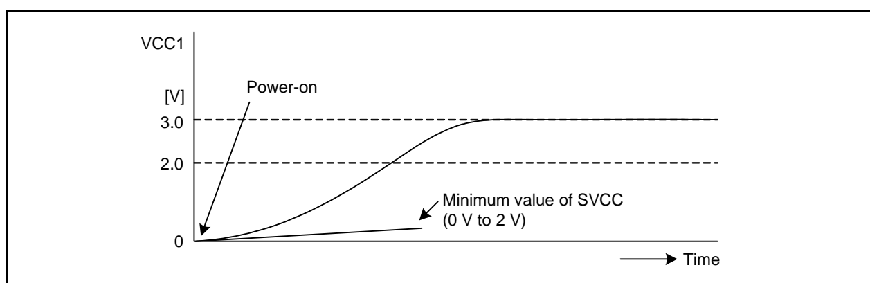
Figure 6.8 SVCC Timing ( 2.2 \text{ V} \leq V_{CC1} \leq 3.6 \text{ V} )
