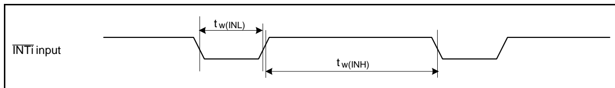
Figure 31.42 External Interrupt \overline{\text{INT}}_i Input
