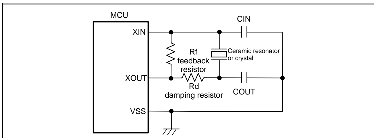
Figure 8.6 Oscillator Example
