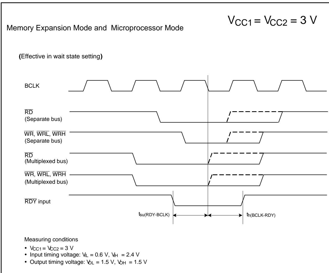
Figure 31.29 Timing Diagram
