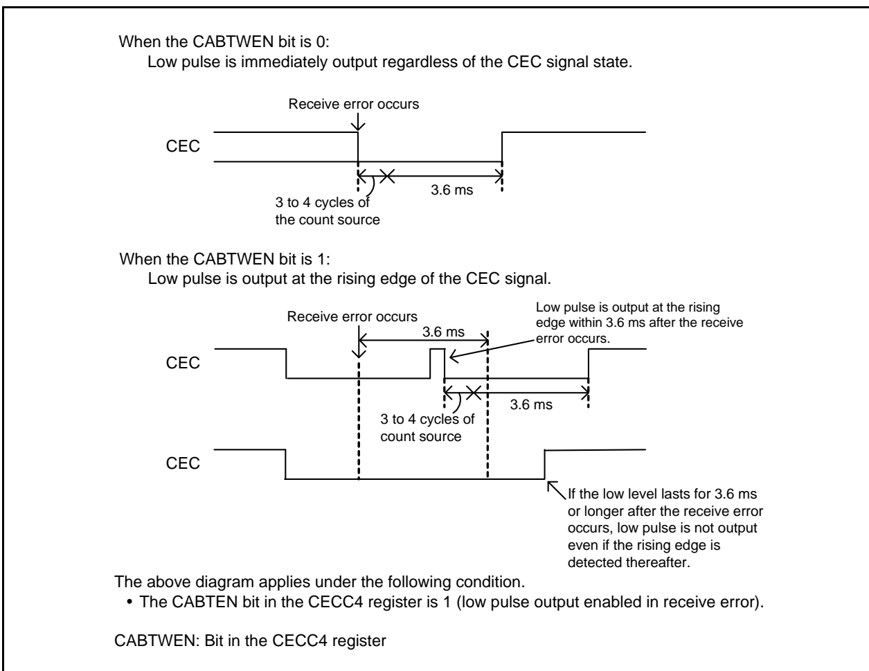
Figure 26.8 Low Pulse Output in Receive Error
