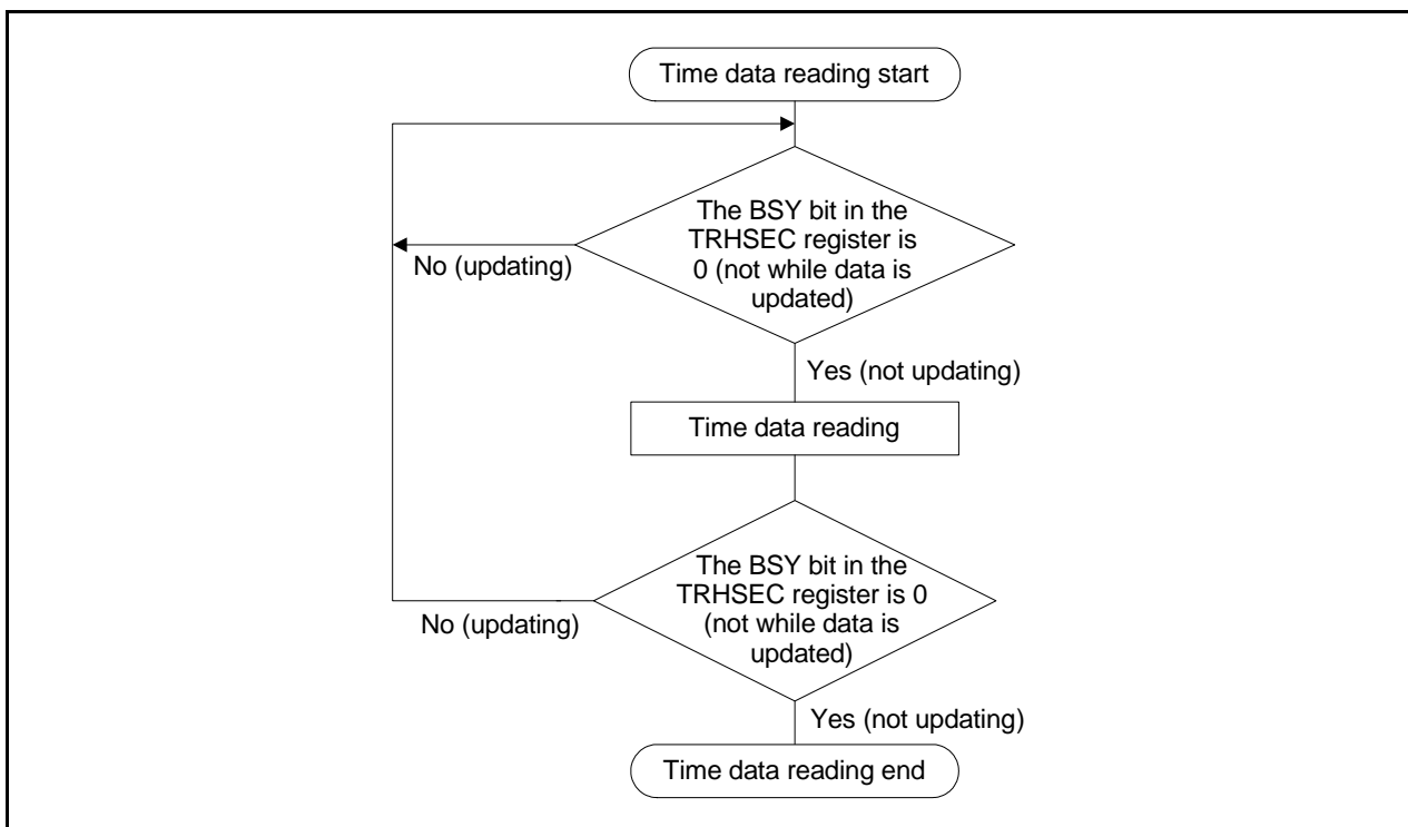
Figure 20.7 Time Data Reading
