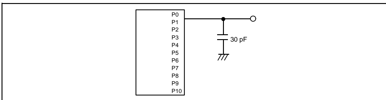
Figure 31.15 Ports P0 to P10 Measurement Circuit
