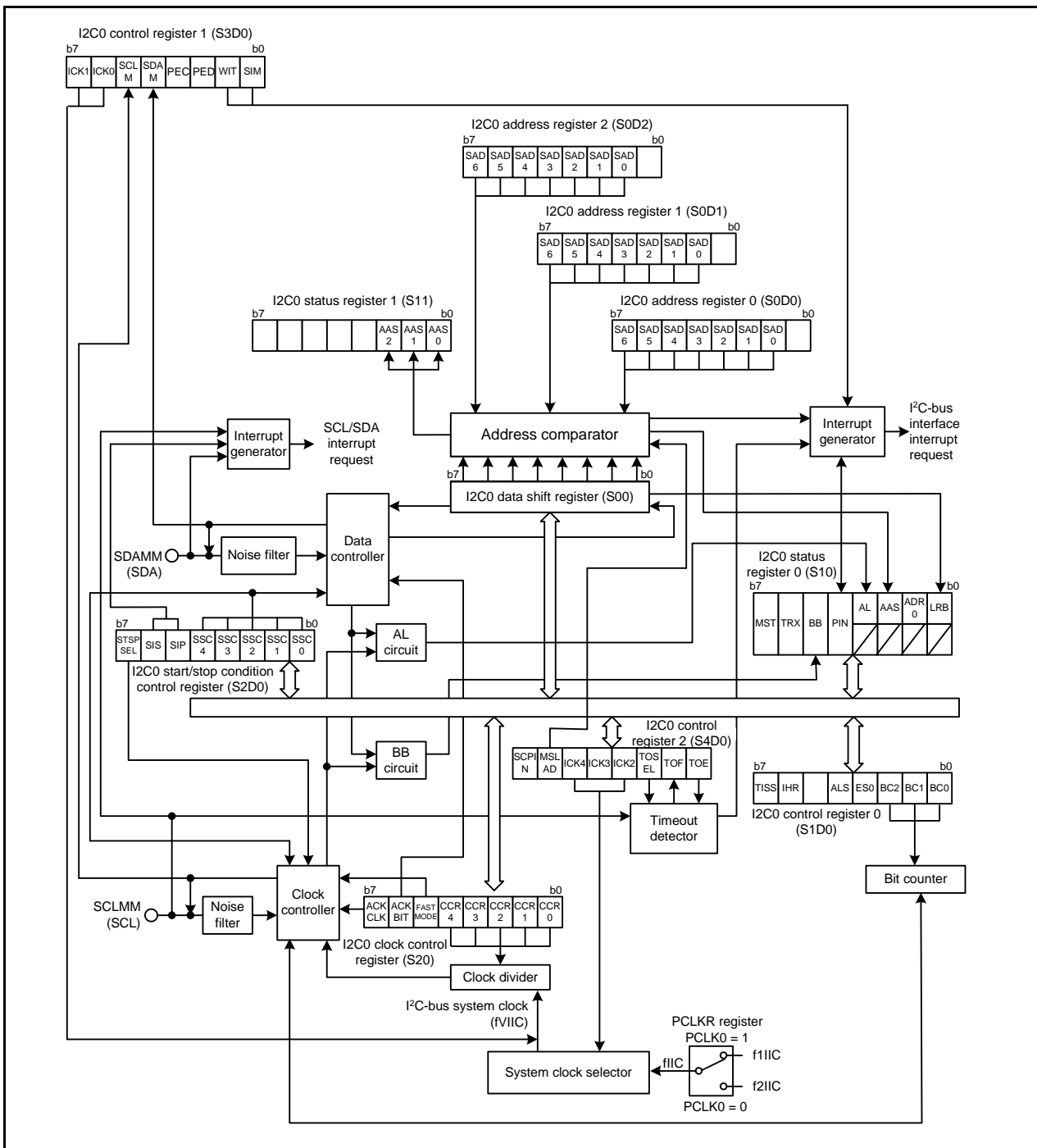
Figure 25.1 Multi-master I 2 C-bus Interface Block Diagram
