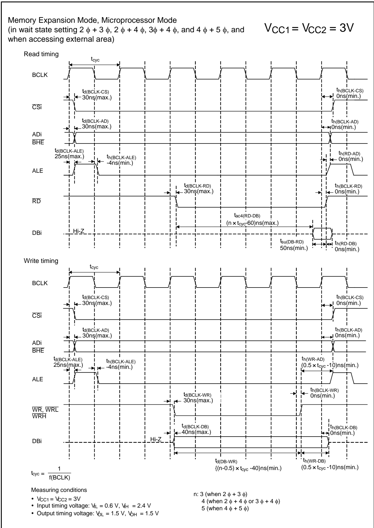
Figure 31.34 Timing Diagram
