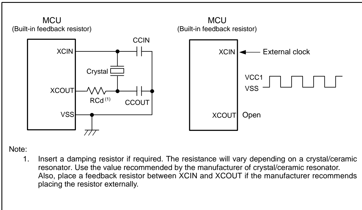
Figure 8.3 Sub Clock Connection Example
