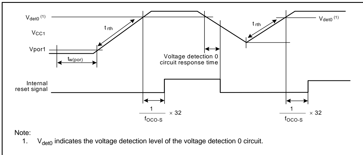
Figure 31.4 Power-On Reset Circuit Electrical Characteristics
