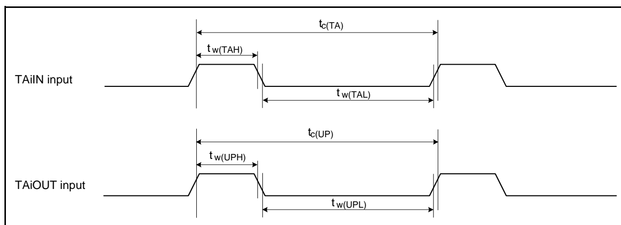
Figure 31.23 Timer A Input
