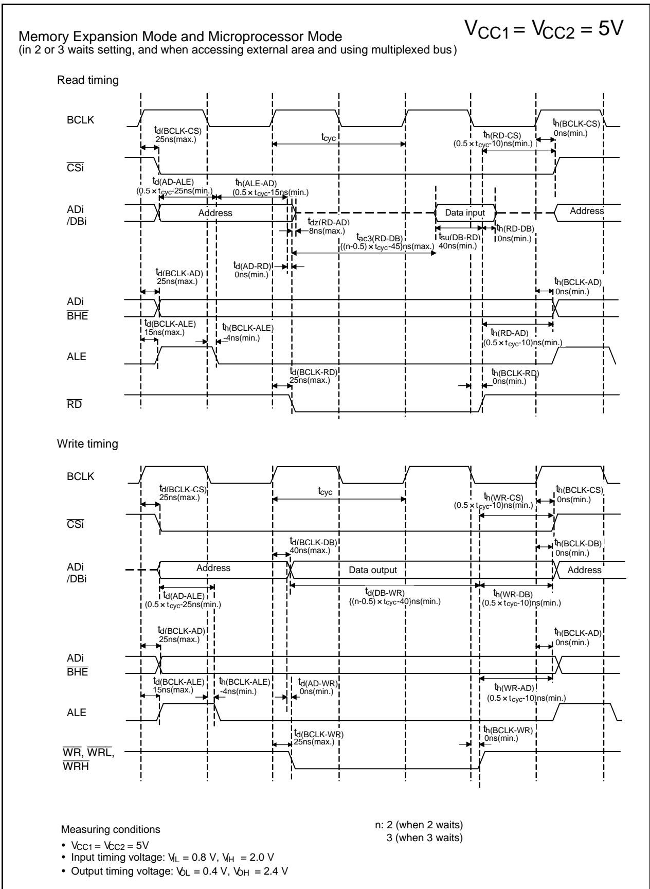
Figure 31.18 Timing Diagram
