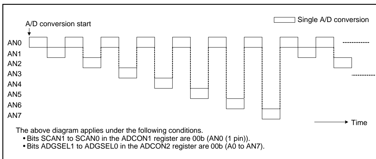
Figure 27.14 Operation Example in Repeat Sweep Mode 1
