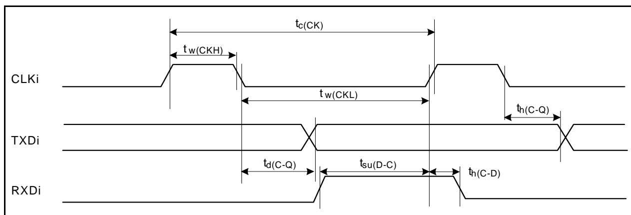
Figure 31.11 Serial Interface
