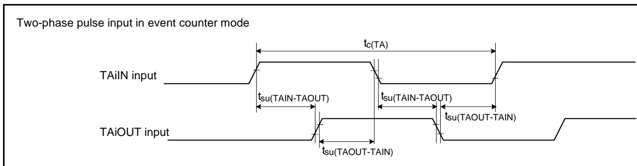
Figure 31.24 Timer A Input (Two-Phase Pulse Input in Event Counter Mode)
