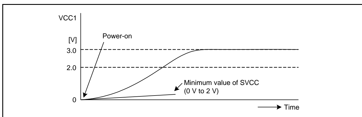
Figure 32.3 SVCC Timing ( 2.2 \text{ V} \leq V_{CC1} \leq 3.6 \text{ V} )
