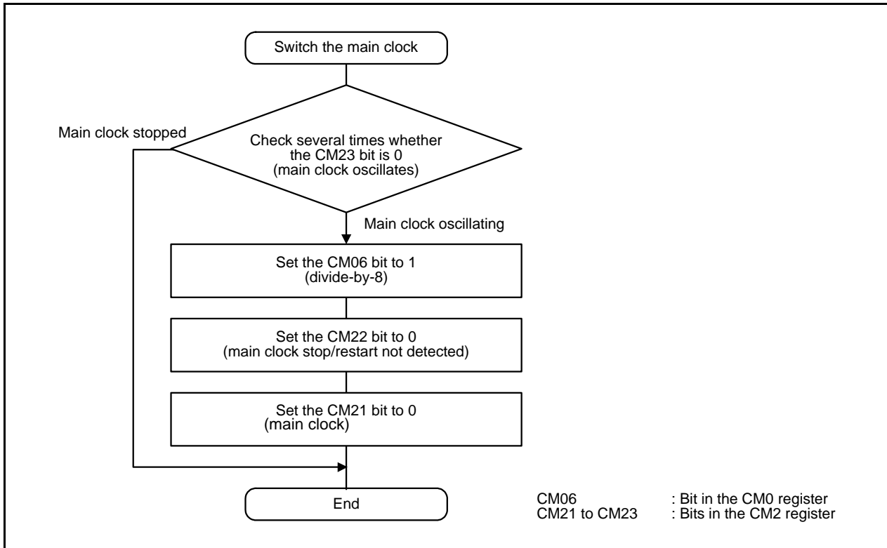
Figure 8.5 Switching from On-Chip Oscillator Clock to Main Clock
