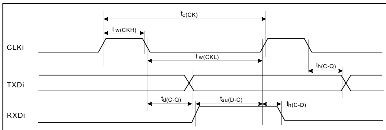
Figure 31.41 Serial Interface
