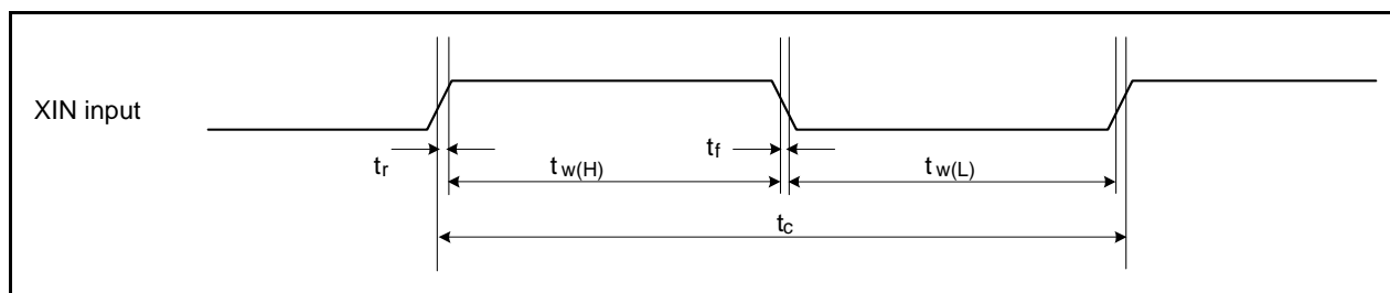
Figure 31.22 External Clock Input (XIN Input)
