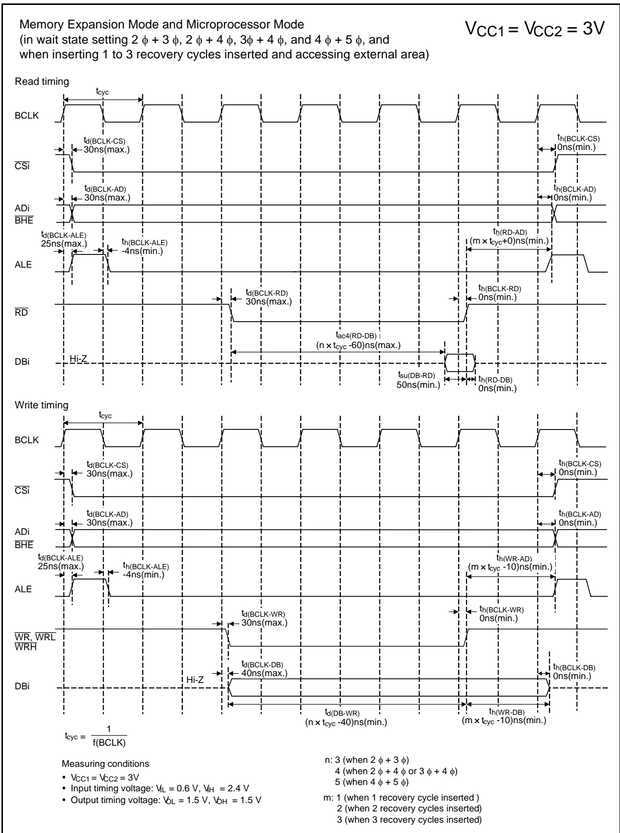
Figure 31.35 Timing Diagram
