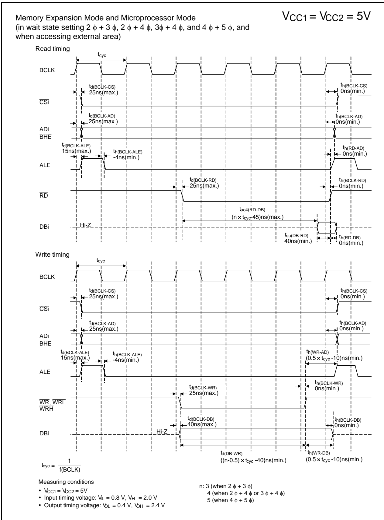
Figure 31.19 Timing Diagram
