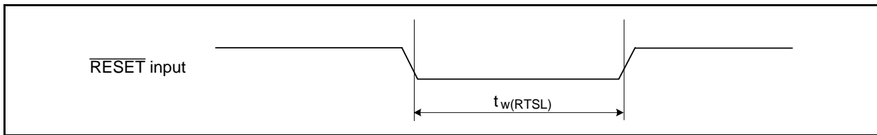
Figure 31.36 Reset Input ( \overline{\text{RESET}} Input)
