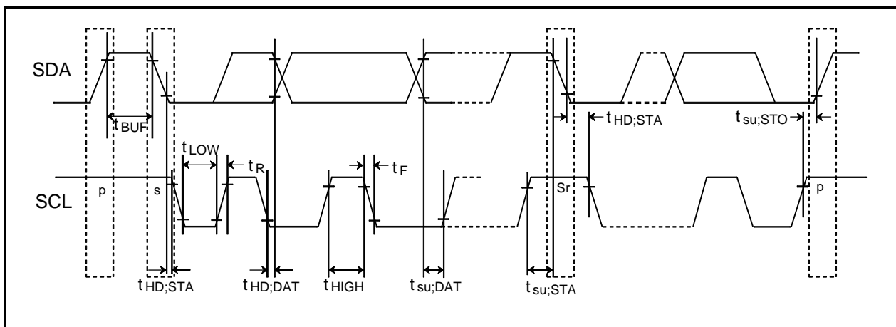
Figure 31.13 Multi-master I 2 C-bus
