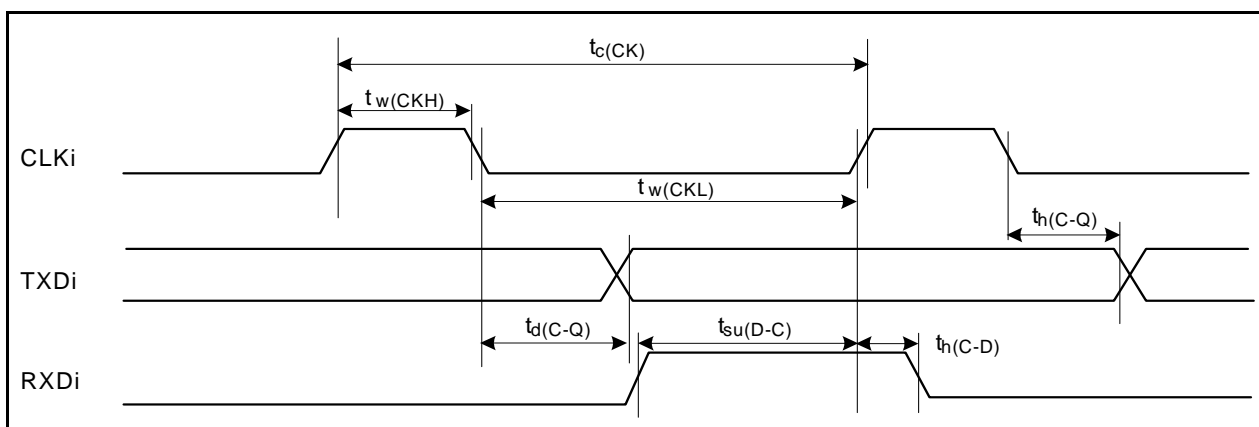
Figure 31.26 Serial Interface
