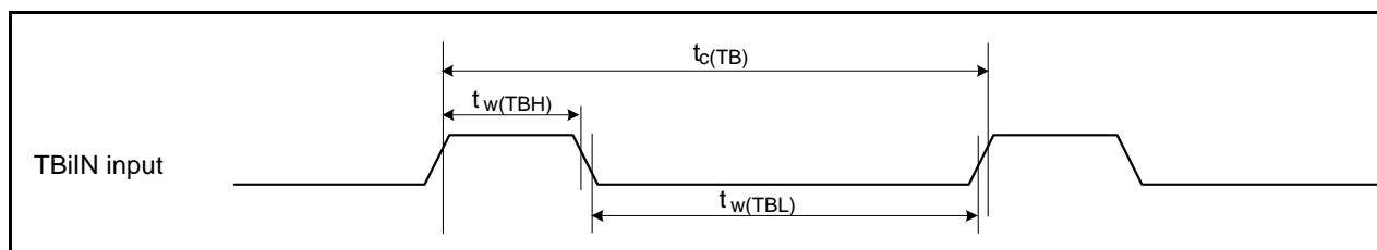
Figure 31.25 Timer B Input
