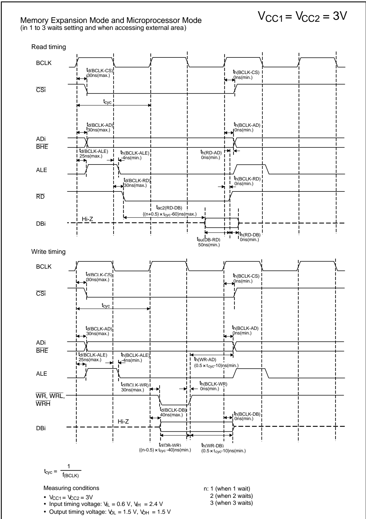
Figure 31.32 Timing Diagram
