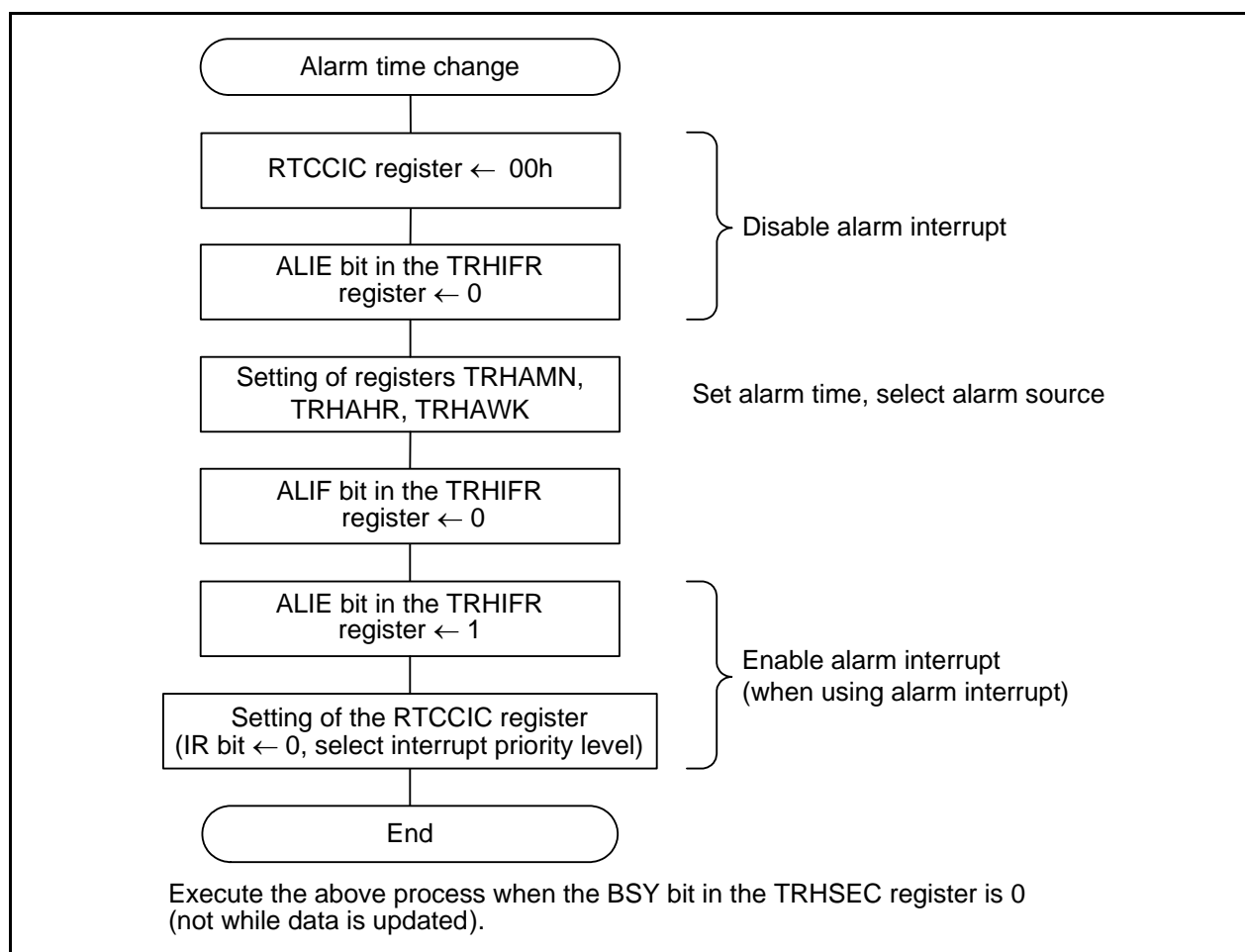
Figure 20.5 Procedure for Setting Alarm Time
