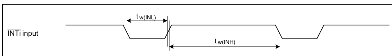
Figure 31.27 External Interrupt \overline{INTi} Input
