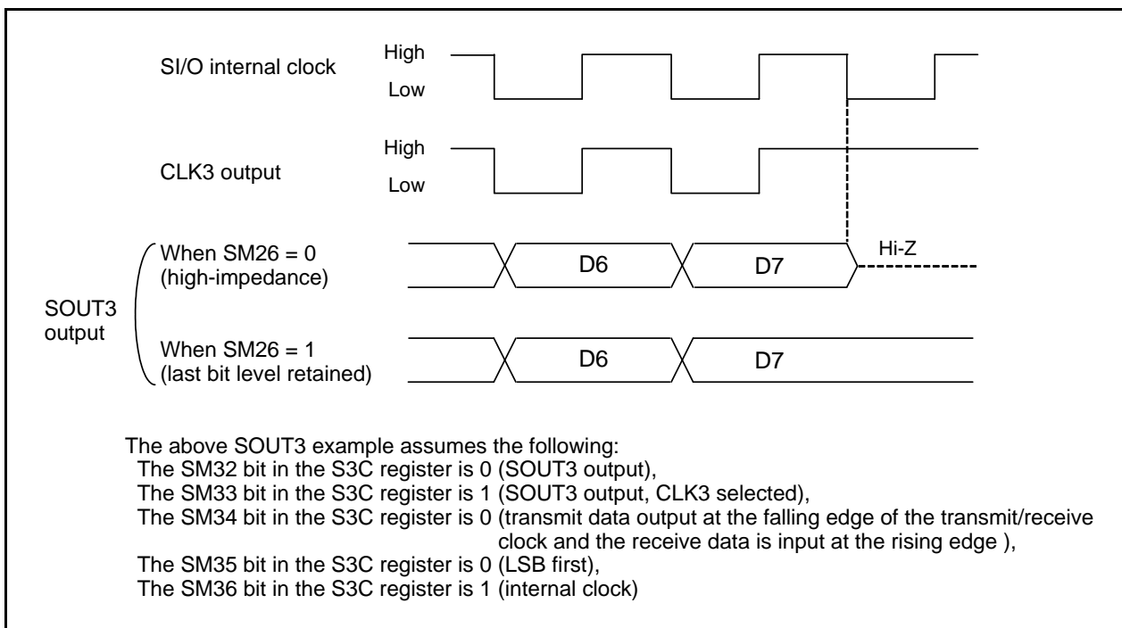
Figure 24.5 SOUT3 Pin Level after Transmission
