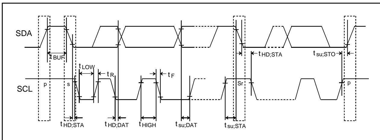
Figure 31.43 Multi-master I 2 C-bus
