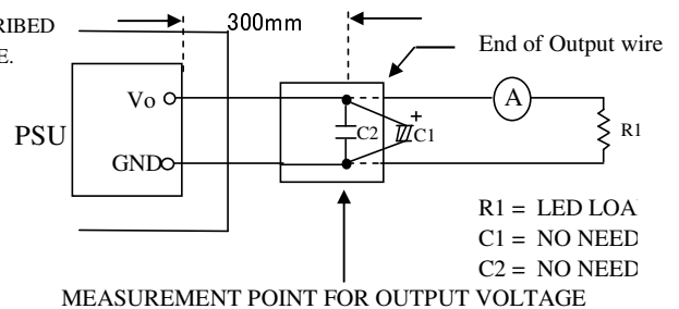
FIGURE A MEASUREMENT SETUP
