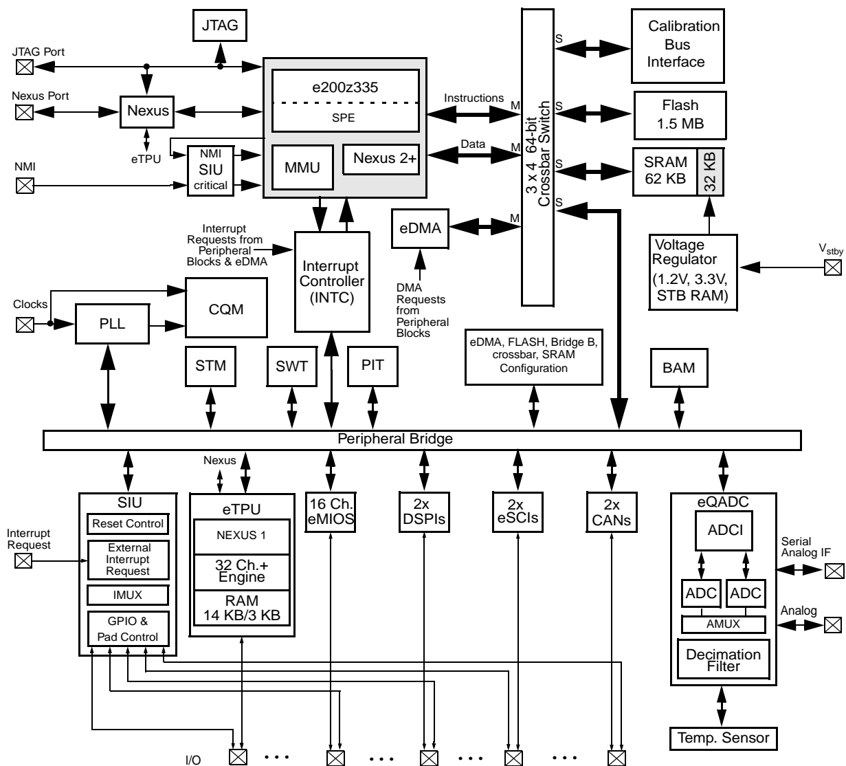
Figure 1. MPC563xM Block Diagram
