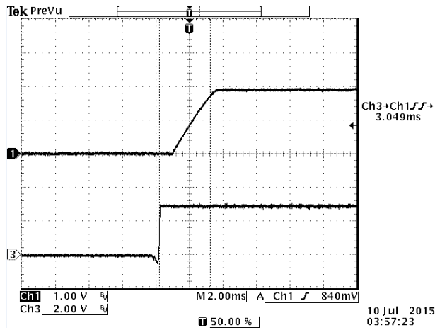
Figure 20. Start up time at full load, 12VDC input 2.0VDC/30A output and Ta=25 °C
