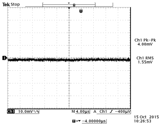
Figure 6. Ripple and noise at full load, 12VDC input 0.6VDC/30A output and T_a=25^\circ\text{C}
