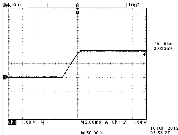
Figure 17. Rise time at full load, 12VDC input 2.0VDC/30A output and T_a=25^\circ\text{C}
