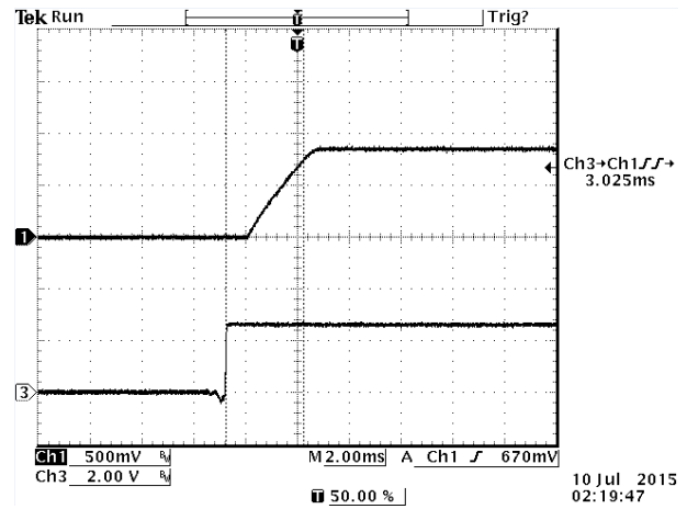
Figure 19. Start up time at full load, 12VDC input 0.9VDC/30A output and Ta=25 °C
