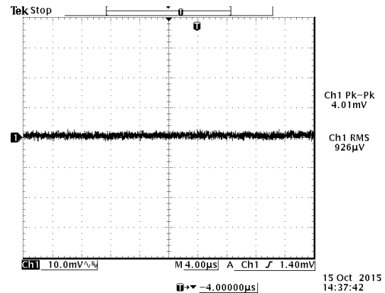
Figure 7. Ripple and noise at full load, 12VDC input 0.9VDC/30A output and T_a=25^\circ\text{C}
