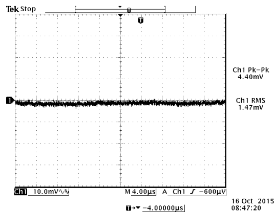
Figure 8. Ripple and noise at full load, 12VDC input 2.0VDC/30A output and T_a=25^\circ\text{C}
