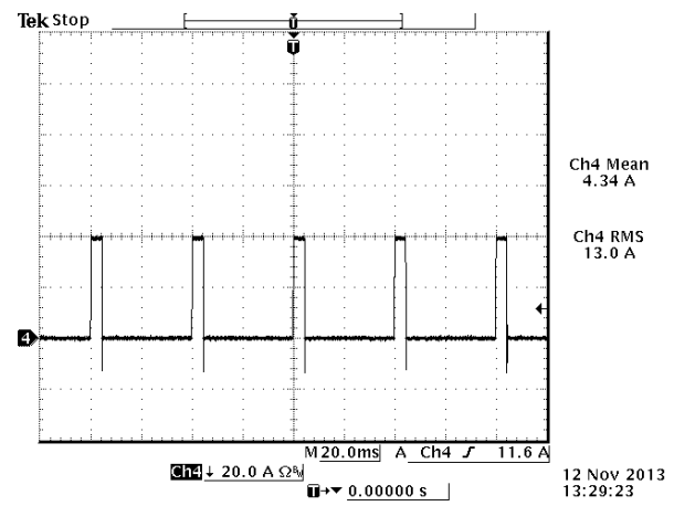
Figure 24. Output current @ SCP, V_{in} = 12V V_{out} = 2.0V, T_a = 25^\circ C
