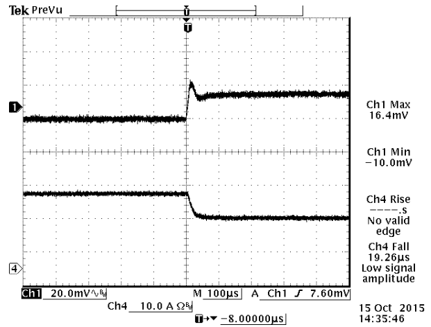
Figure 14. V_{in} = 75% - 50% Load Transient at V_{in} = 12 VDC V_{out} = 2.0VDC @ T_a = 25 °C
