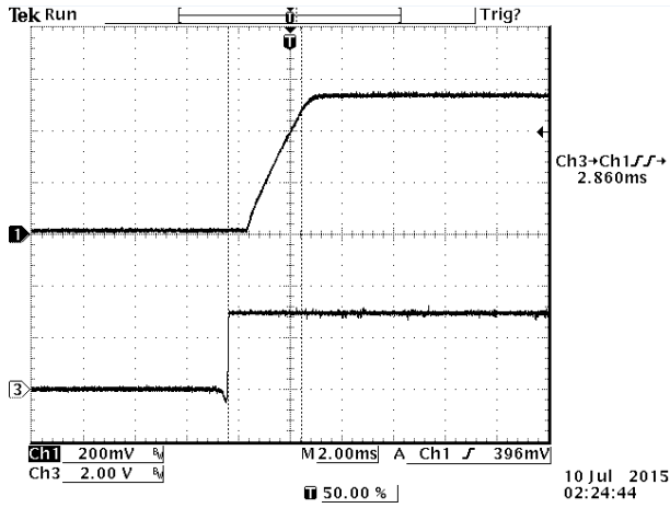
Figure 18. Start up time at full load, 12VDC input 0.6VDC/30A output and Ta=25 °C
