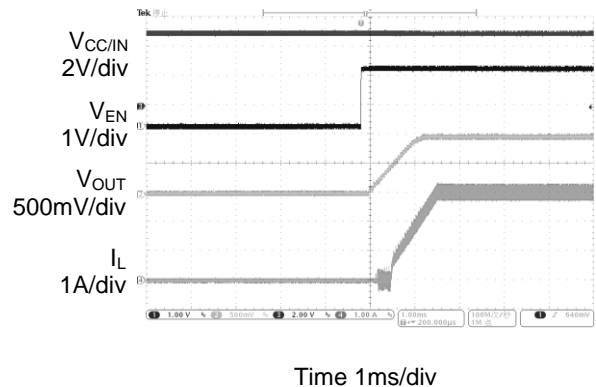
Enable Waveform (V_IN = V_CC = 5V, V_OUT = 1V, I_OUT = 3A)
